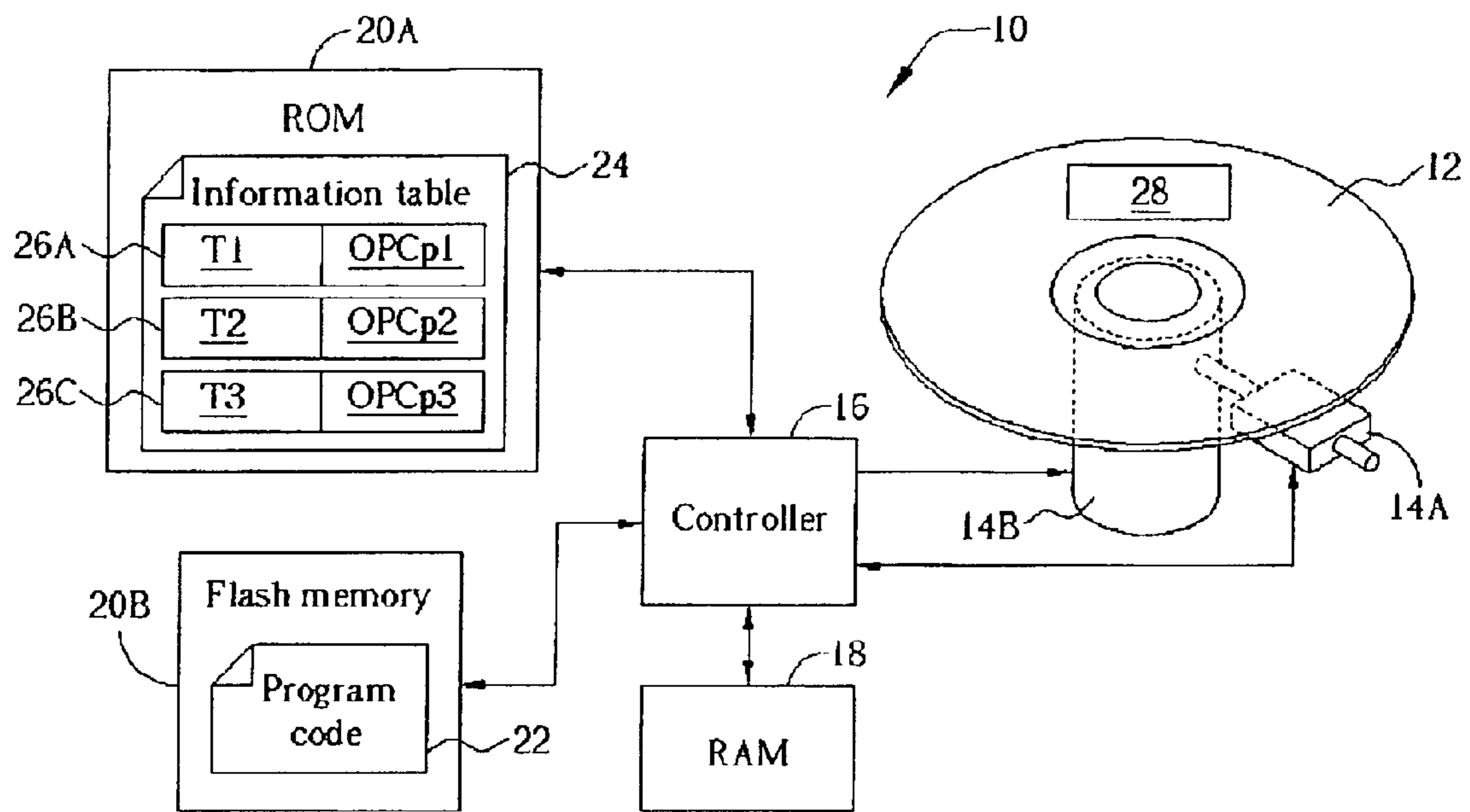
Fig. 1 Prior art
