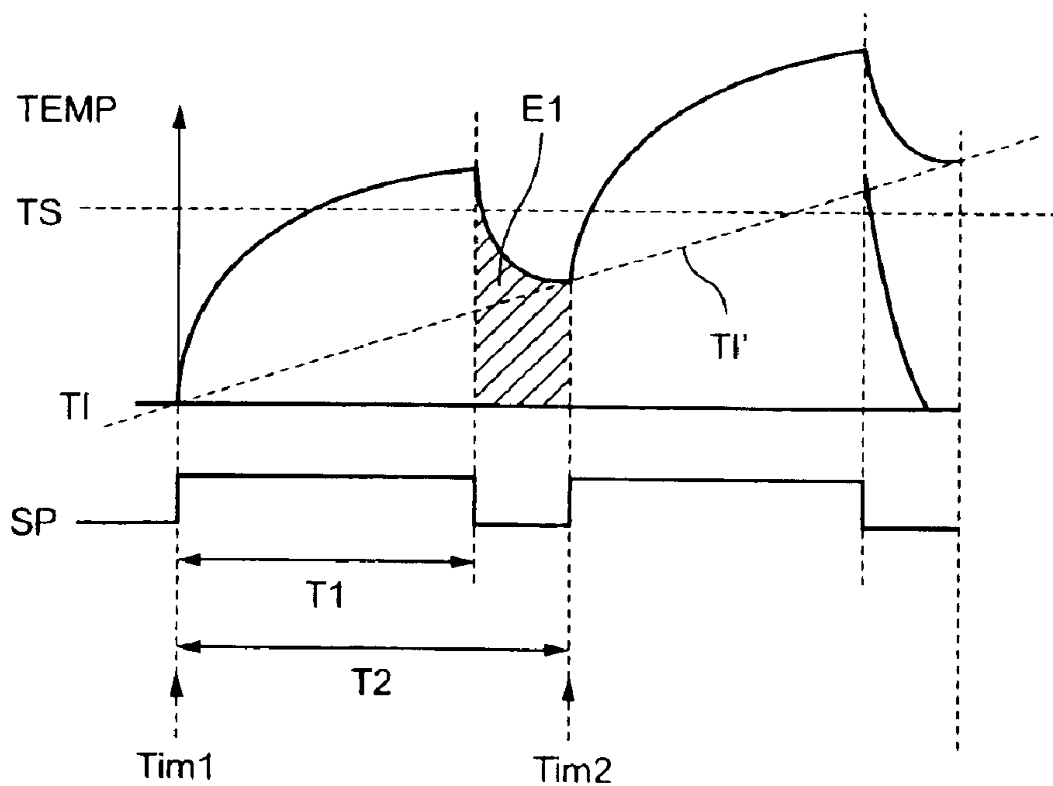
ACTUAL CHARACTERISTICS (UNDER NO CONTROL)
