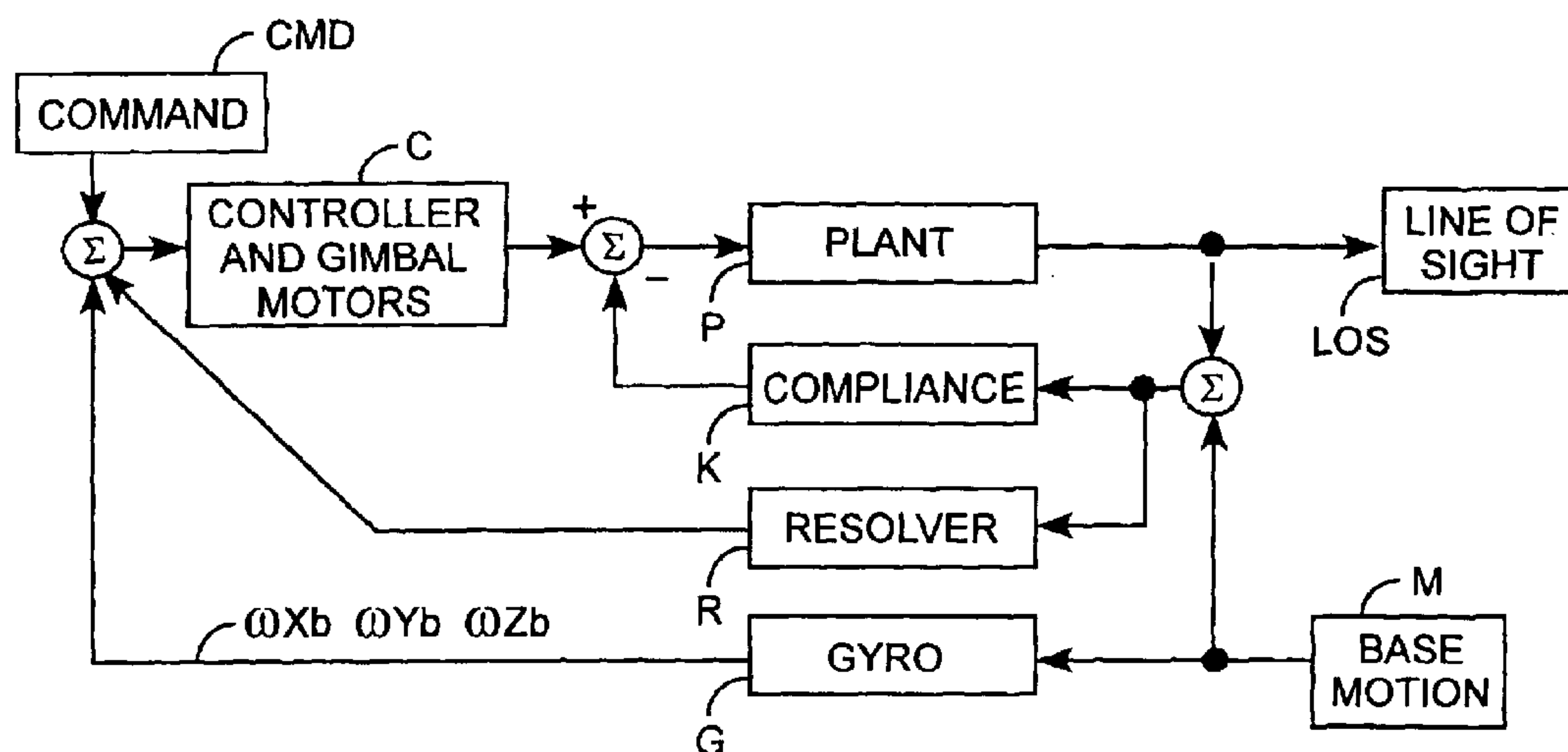
OFF-GIMBAL CONTROL SYSTEM (PRIOR ART)
