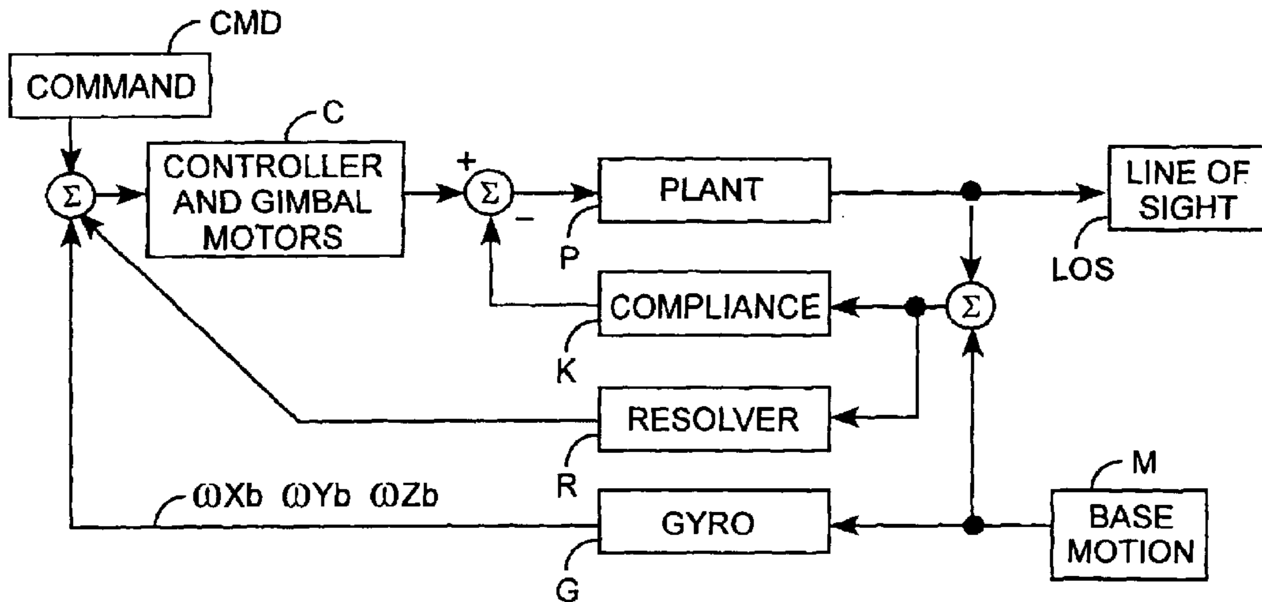
OFF-GIMBAL CONTROL SYSTEM (PRIOR ART)
