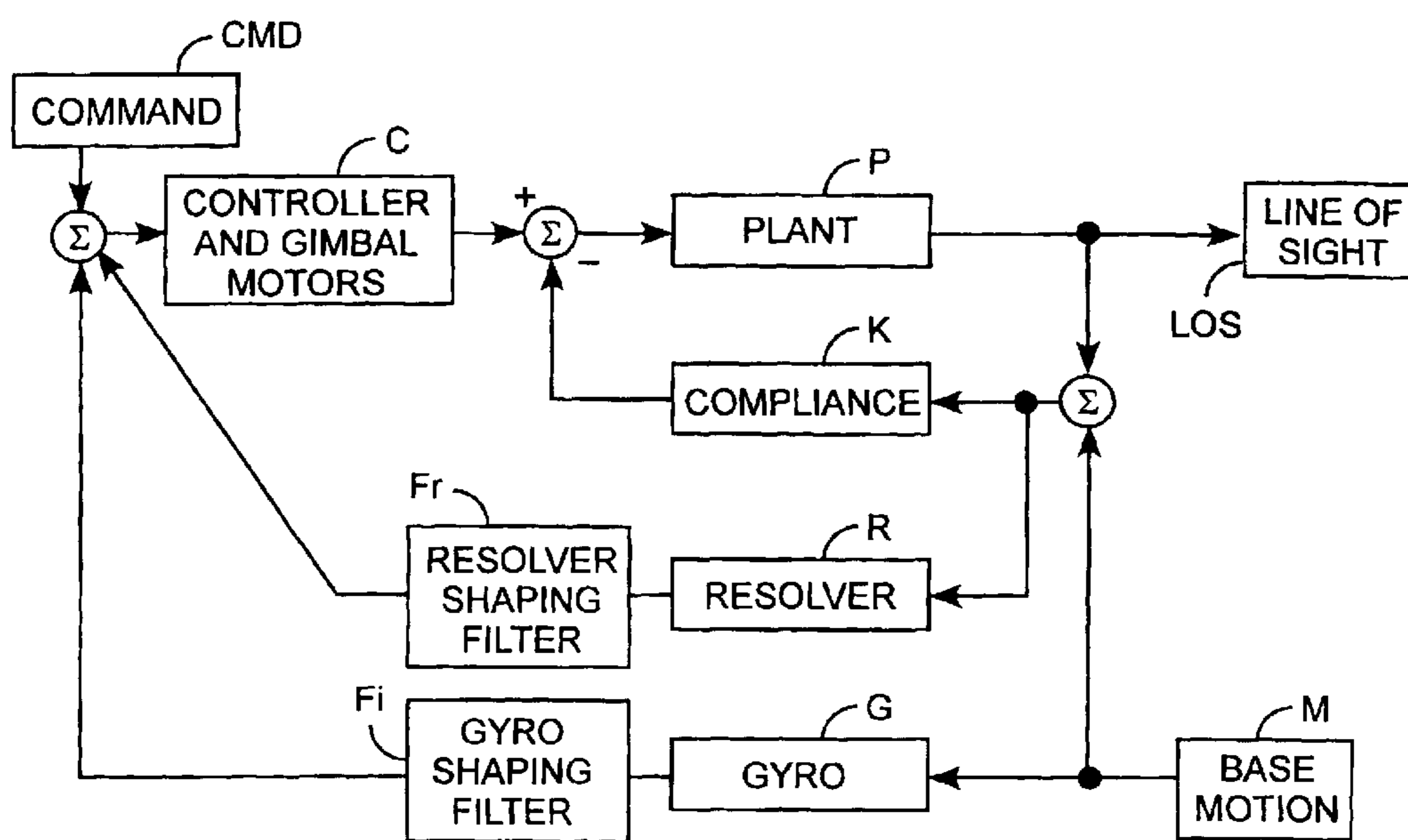
OFF-GIMBAL CONTROL SYSTEM (NEW) FIG. 3
