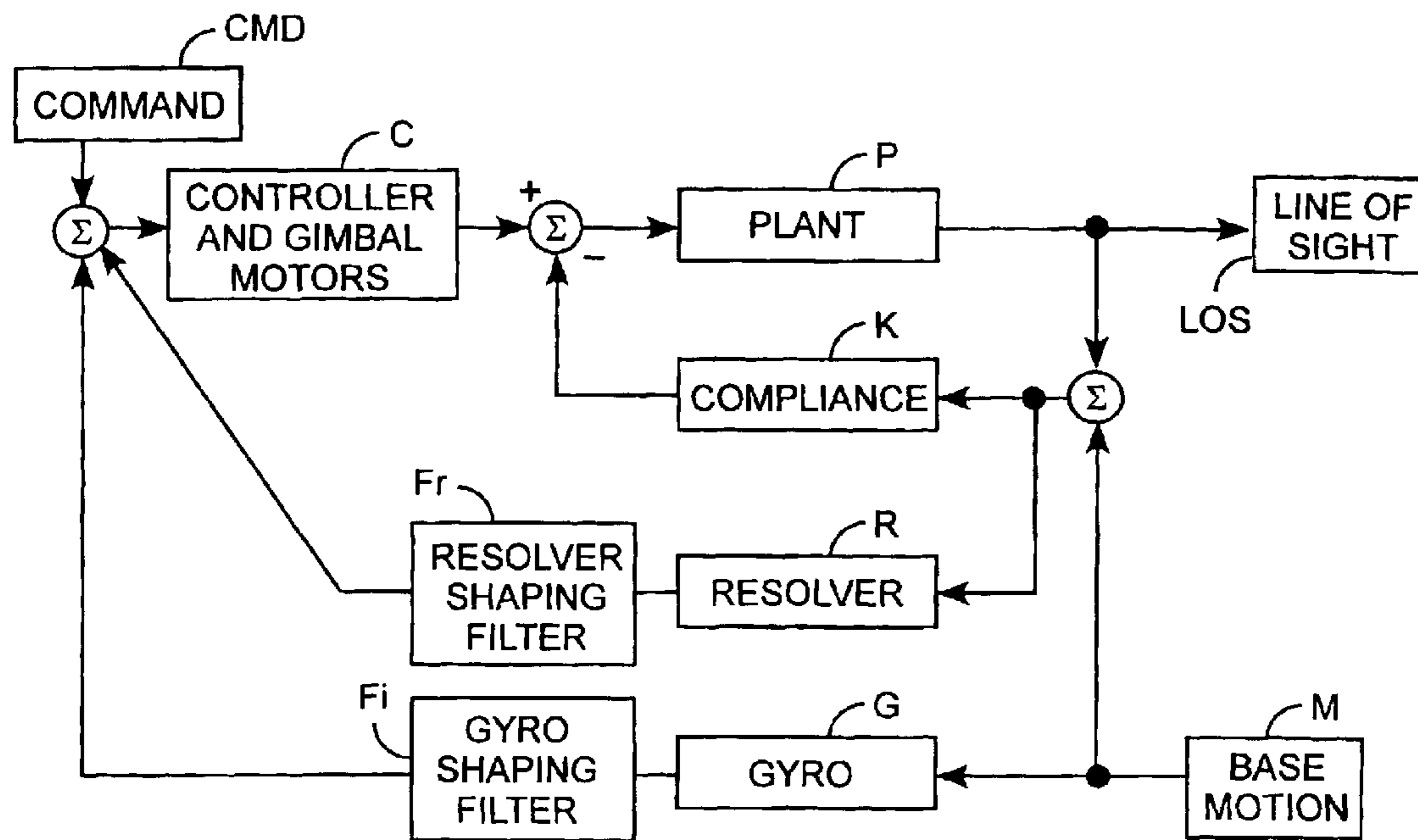
OFF-GIMBAL CONTROL SYSTEM (NEW)
