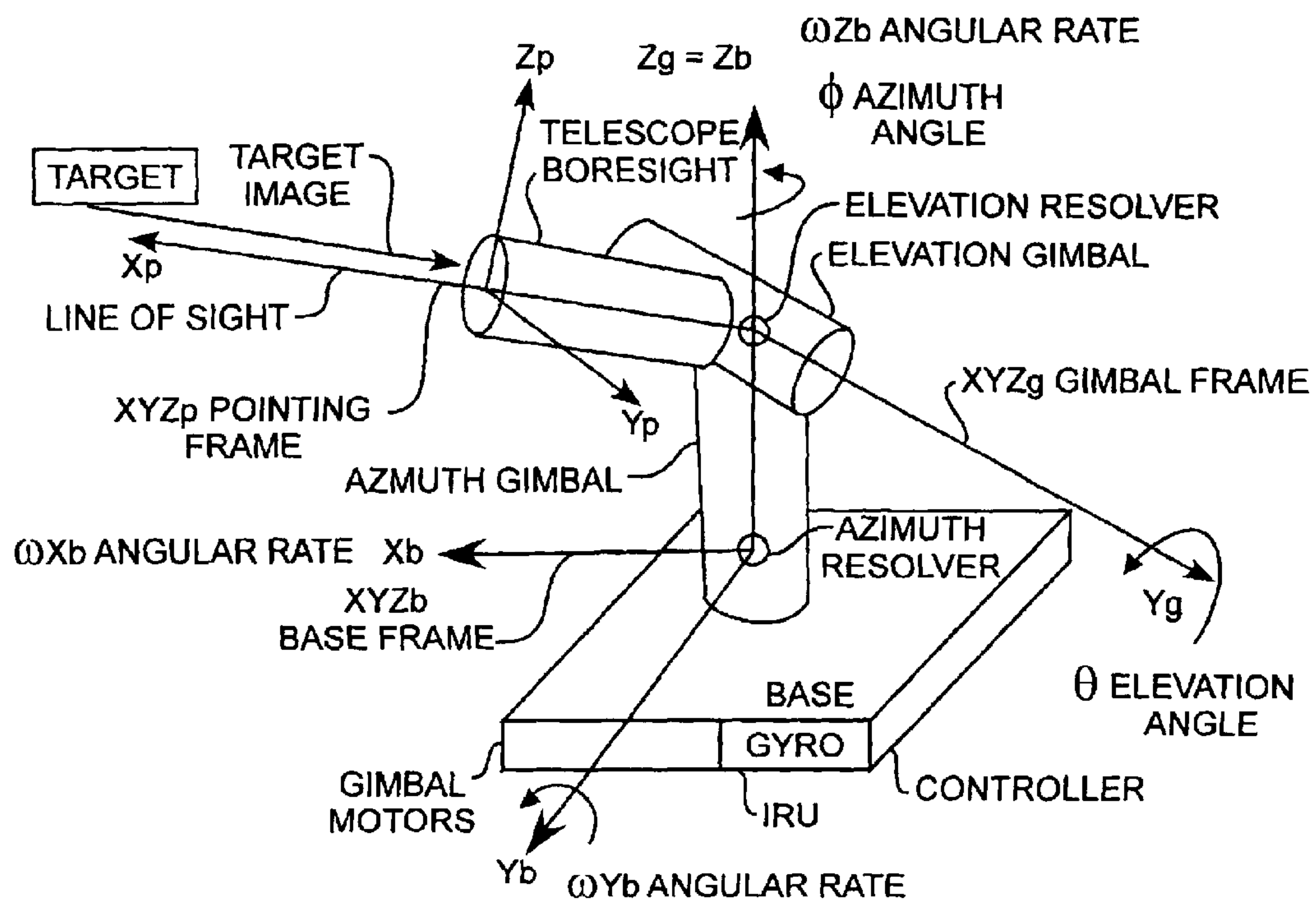
OFF-GIMBAL CONFIGURATION
