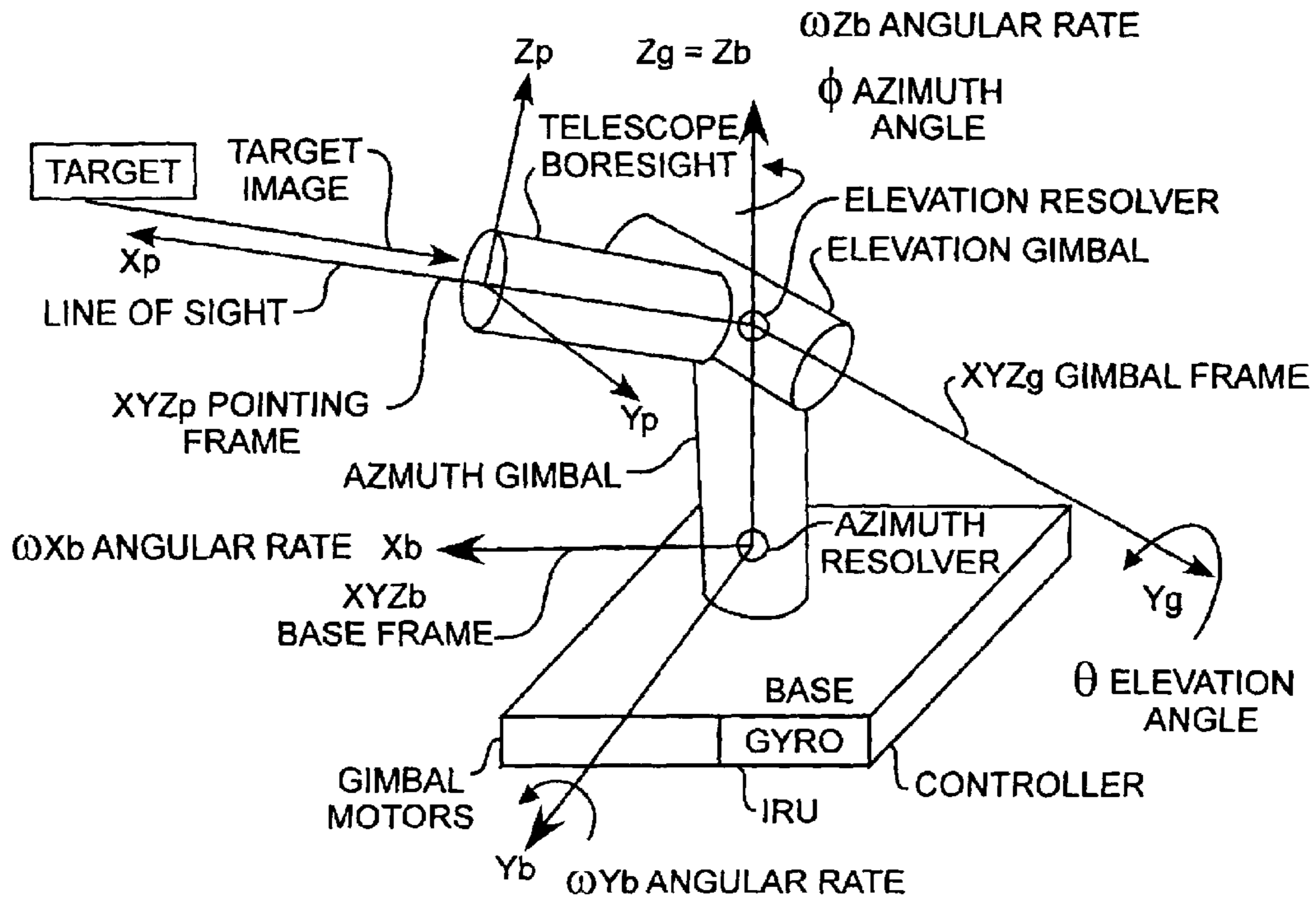
OFF-GIMBAL CONFIGURATION FIG. 1
