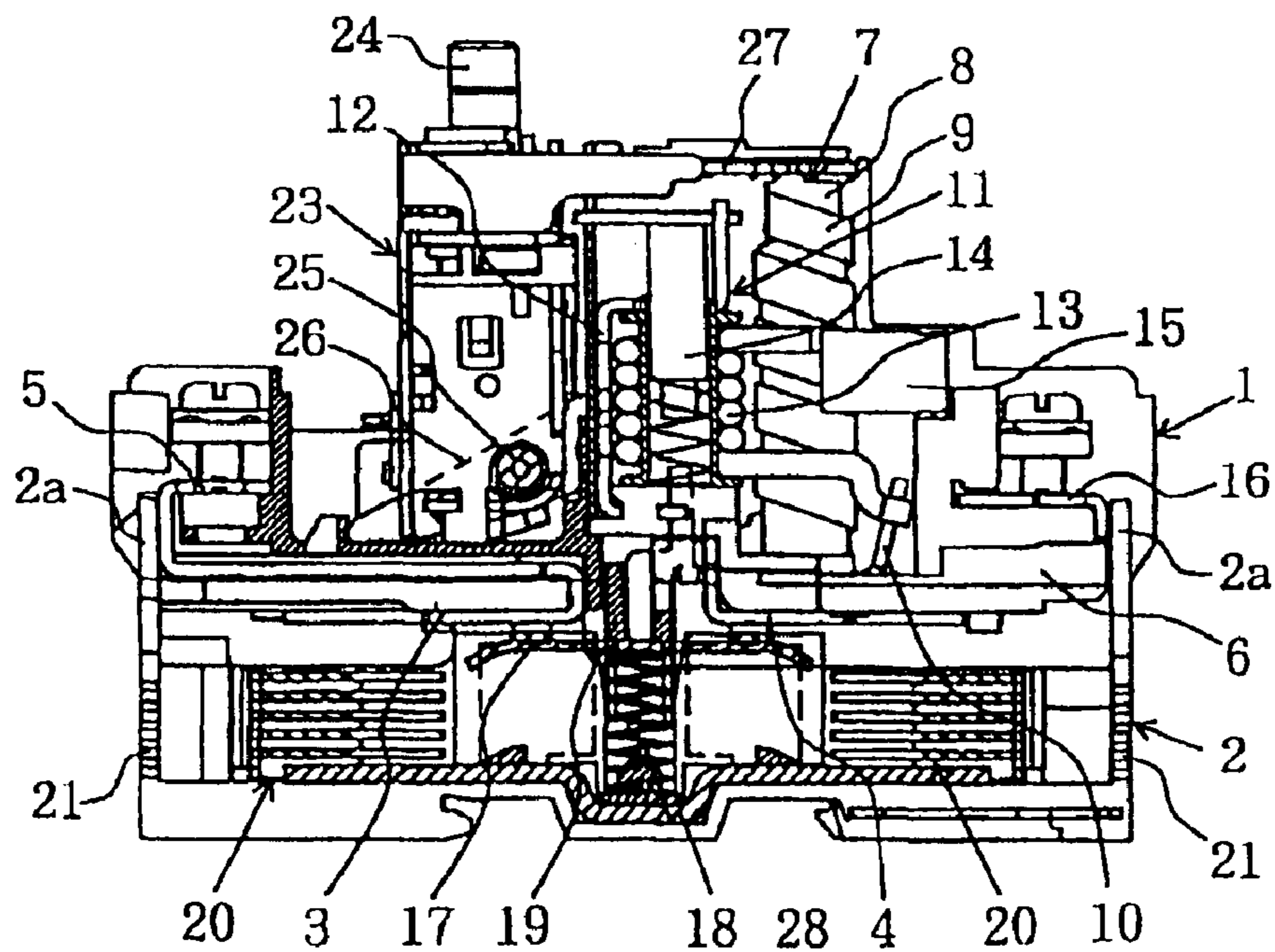
Fig. 6 Prior Art
