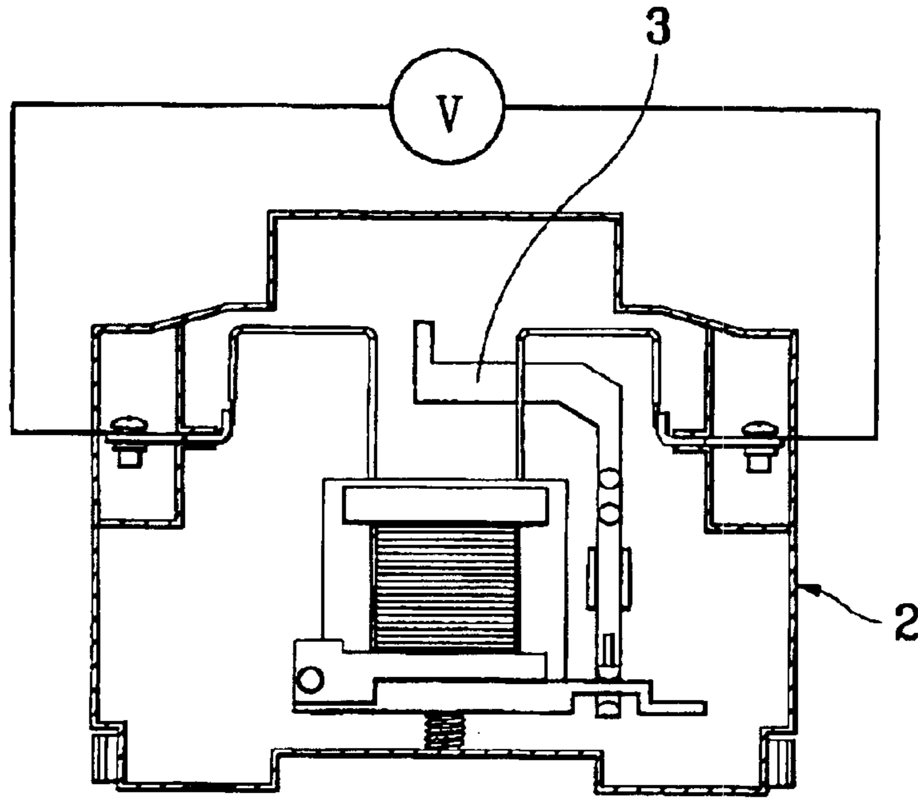
FIG. 2 PRIOR ART
