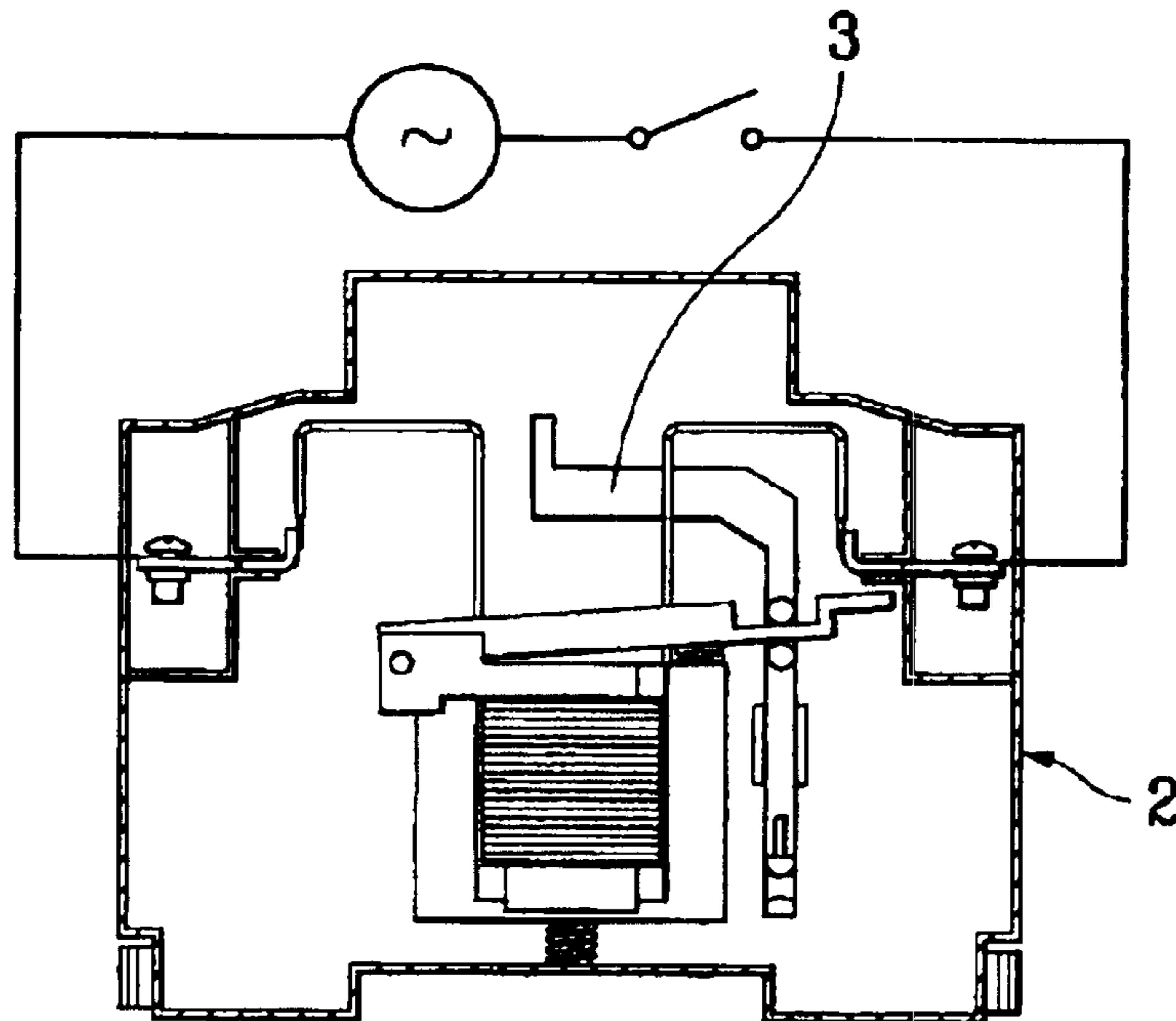
FIG. 3 PRIOR ART
