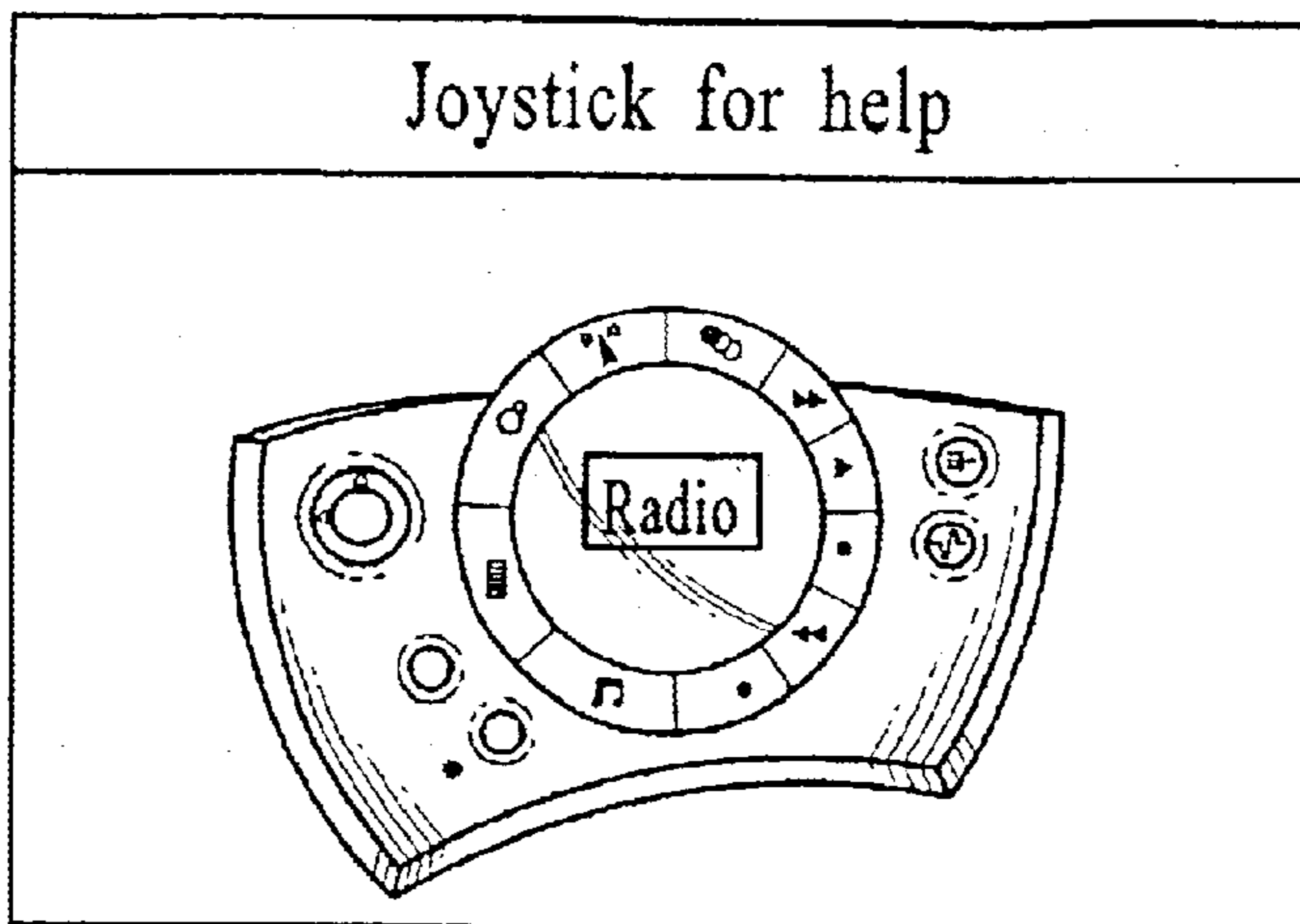
Home Screen
