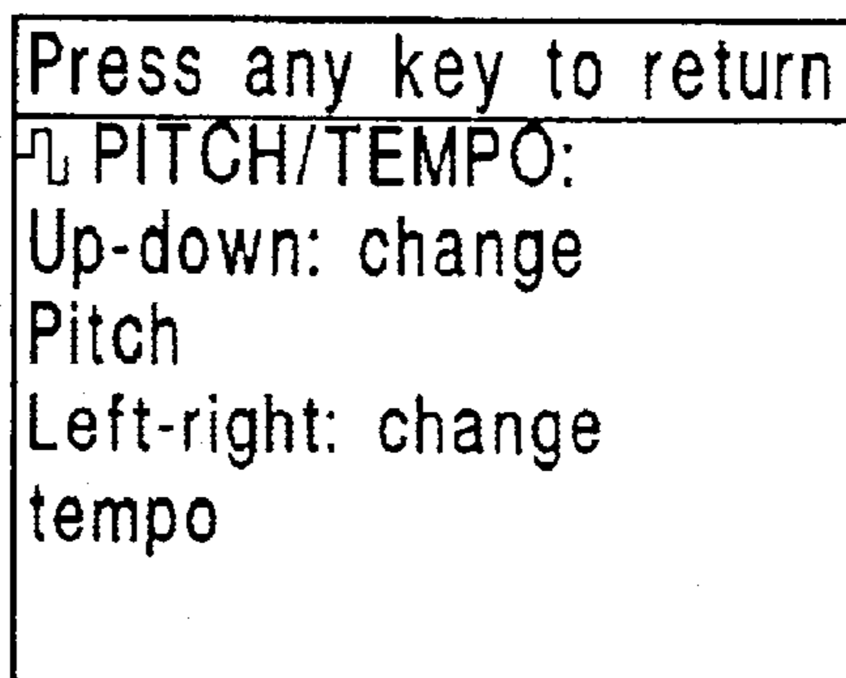
Help Screen
