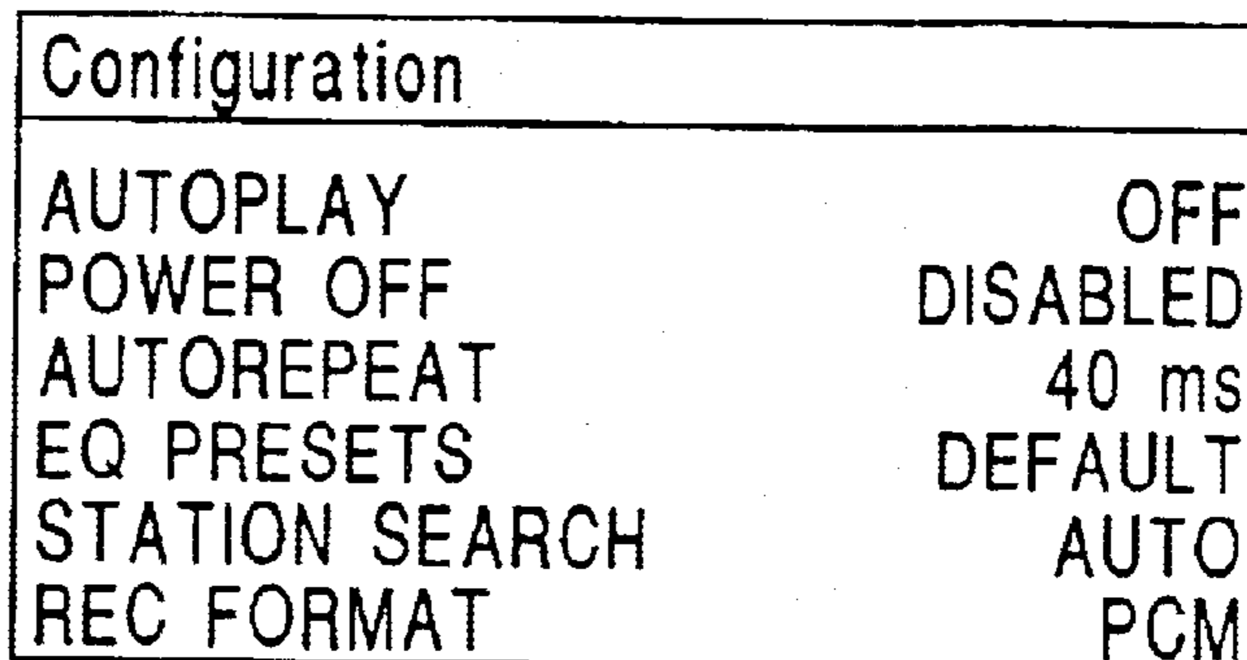
Configuration Screen
