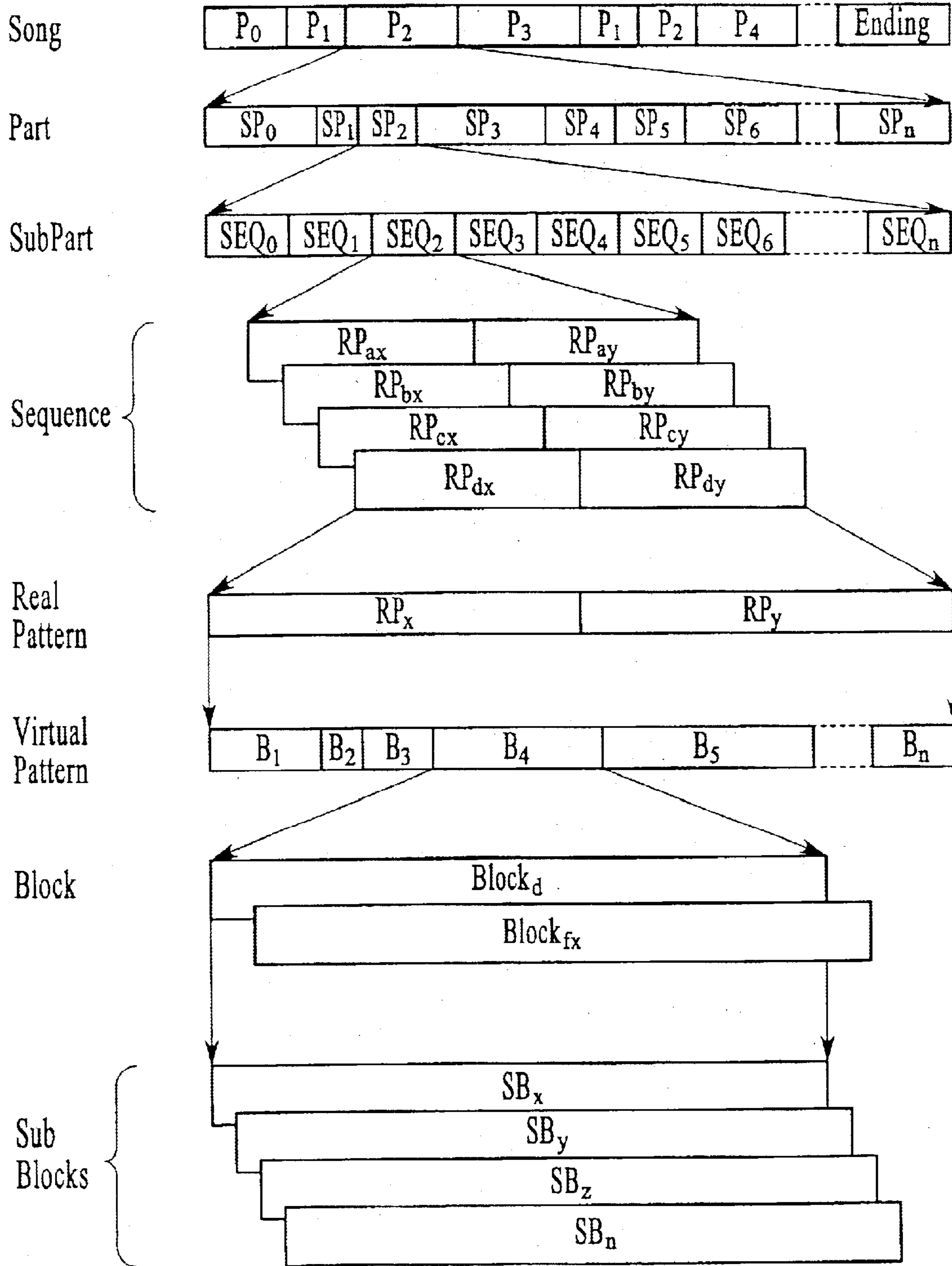
Song Structure
