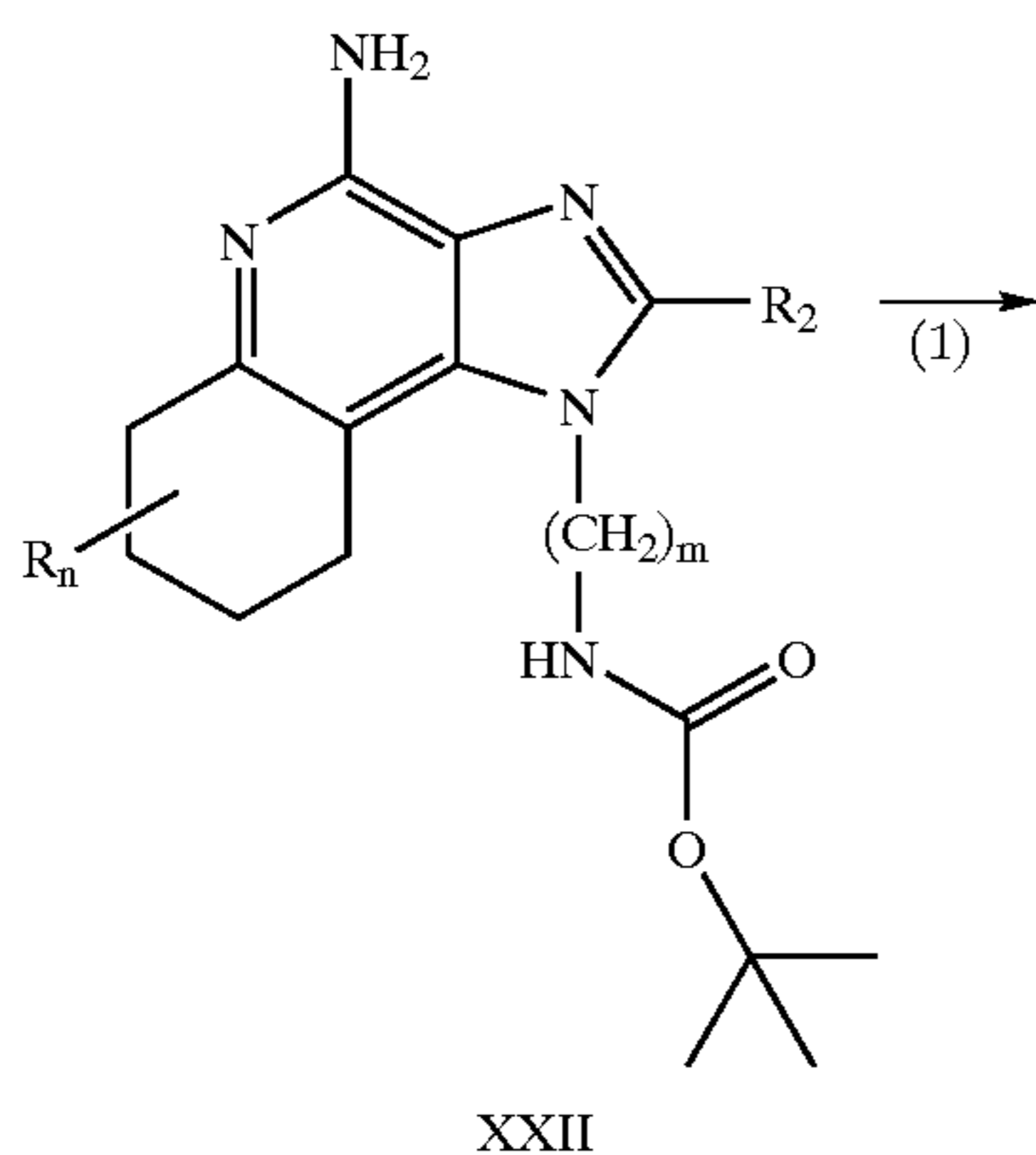
Reaction Scheme VIII
