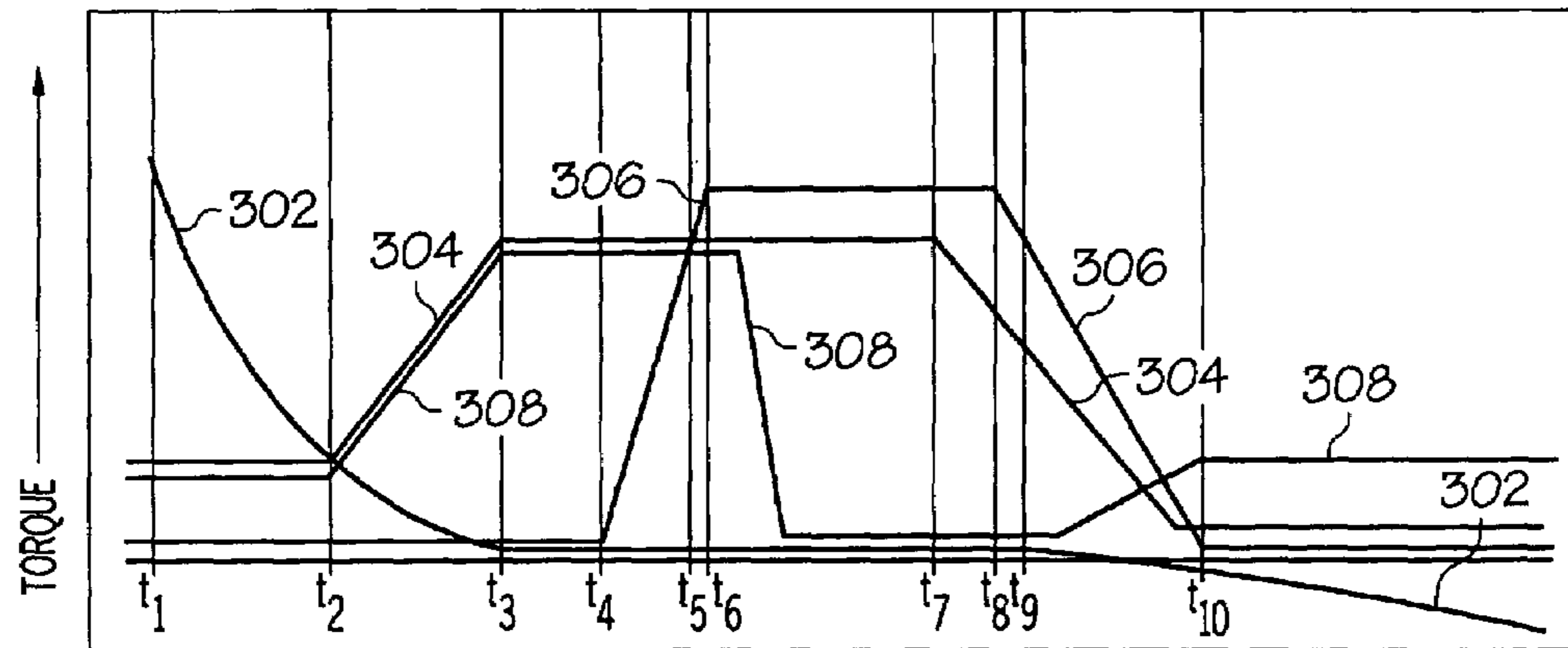
TIME → FIG. 4
