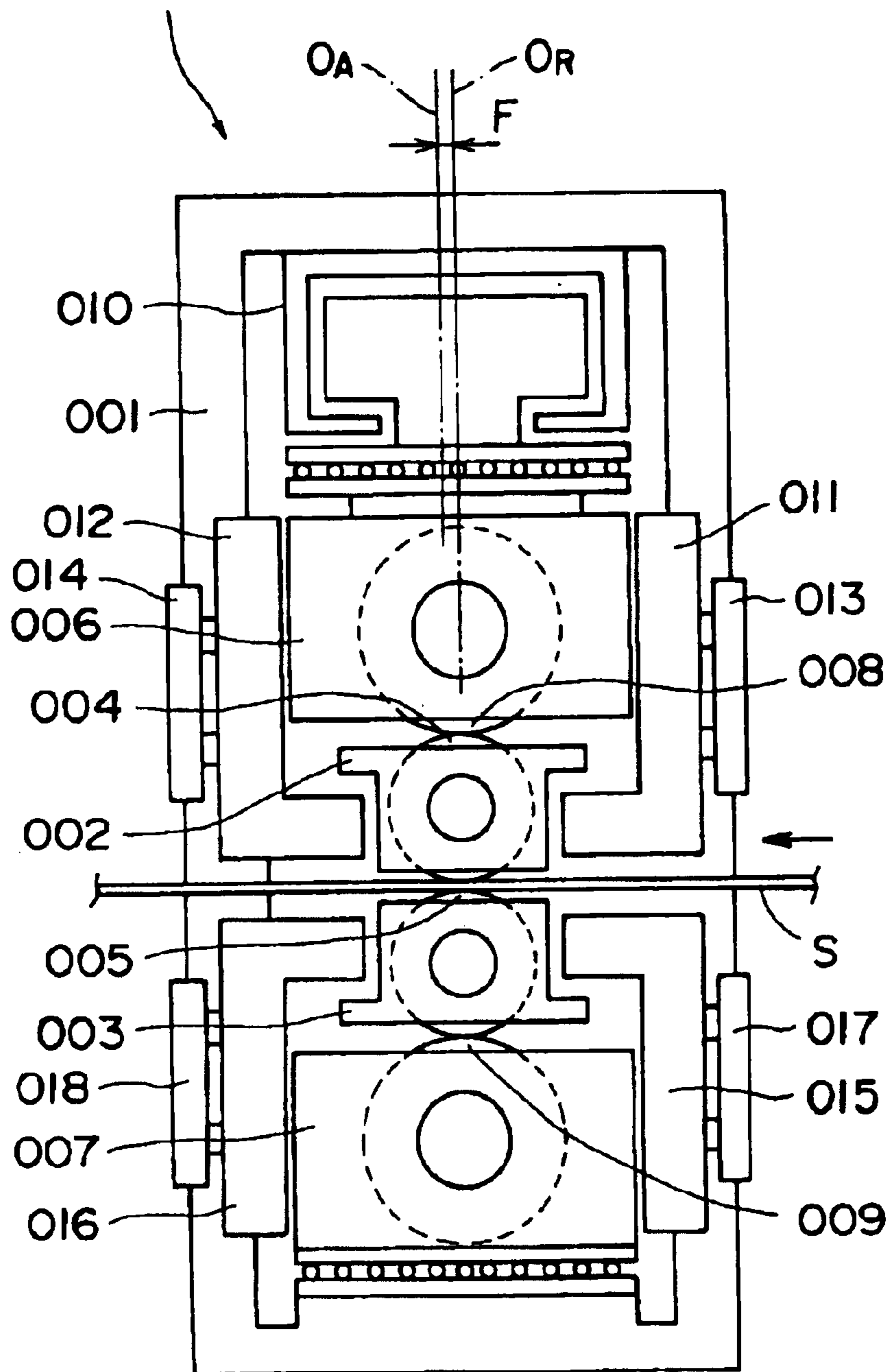
Conventional Cross Rolling Mill
