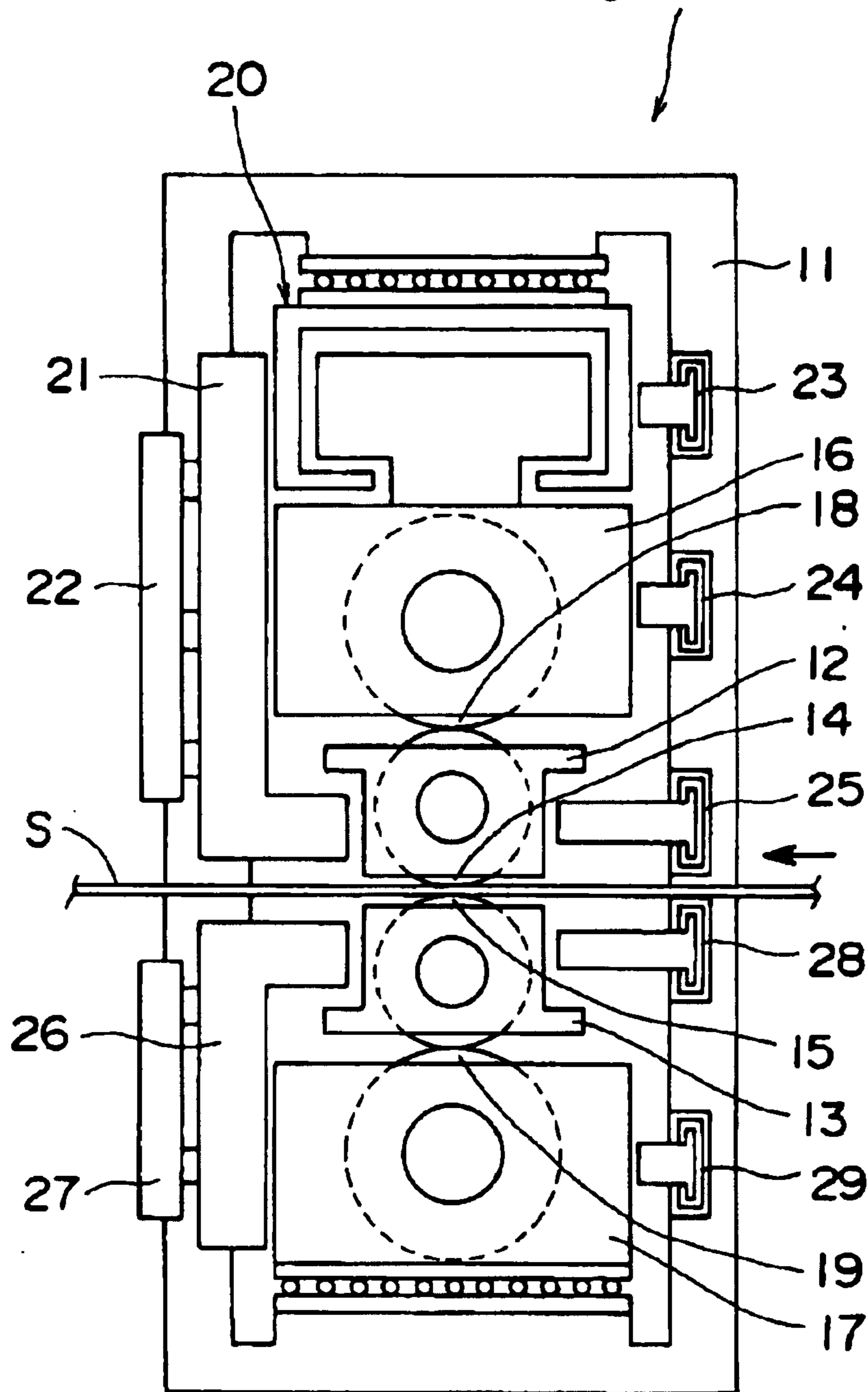
Cross Rolling Mill of First Embodiment
