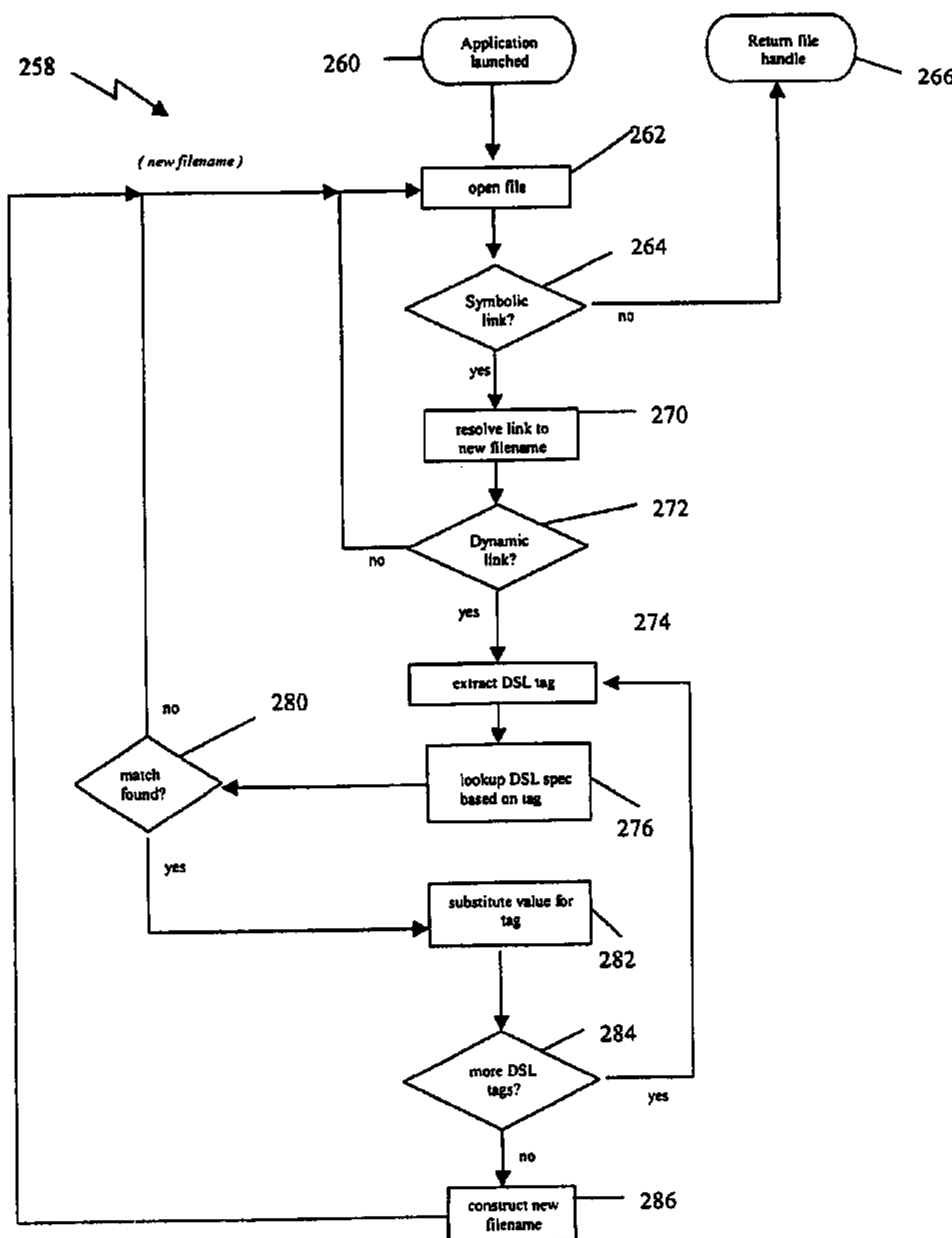
Flowchart of dynamic symbolic link resolution.
