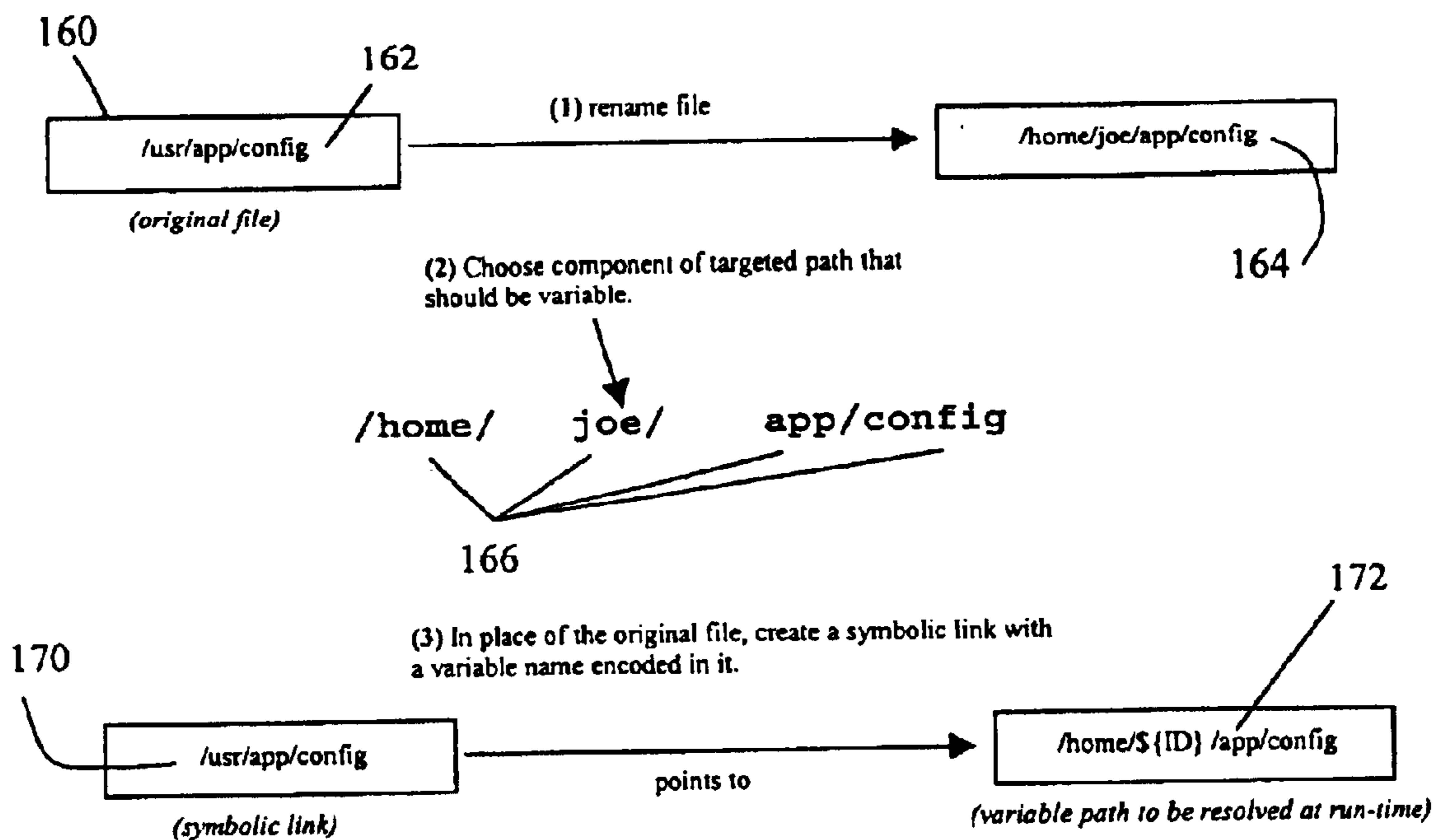
Creation of a dynamic symbolic link.
