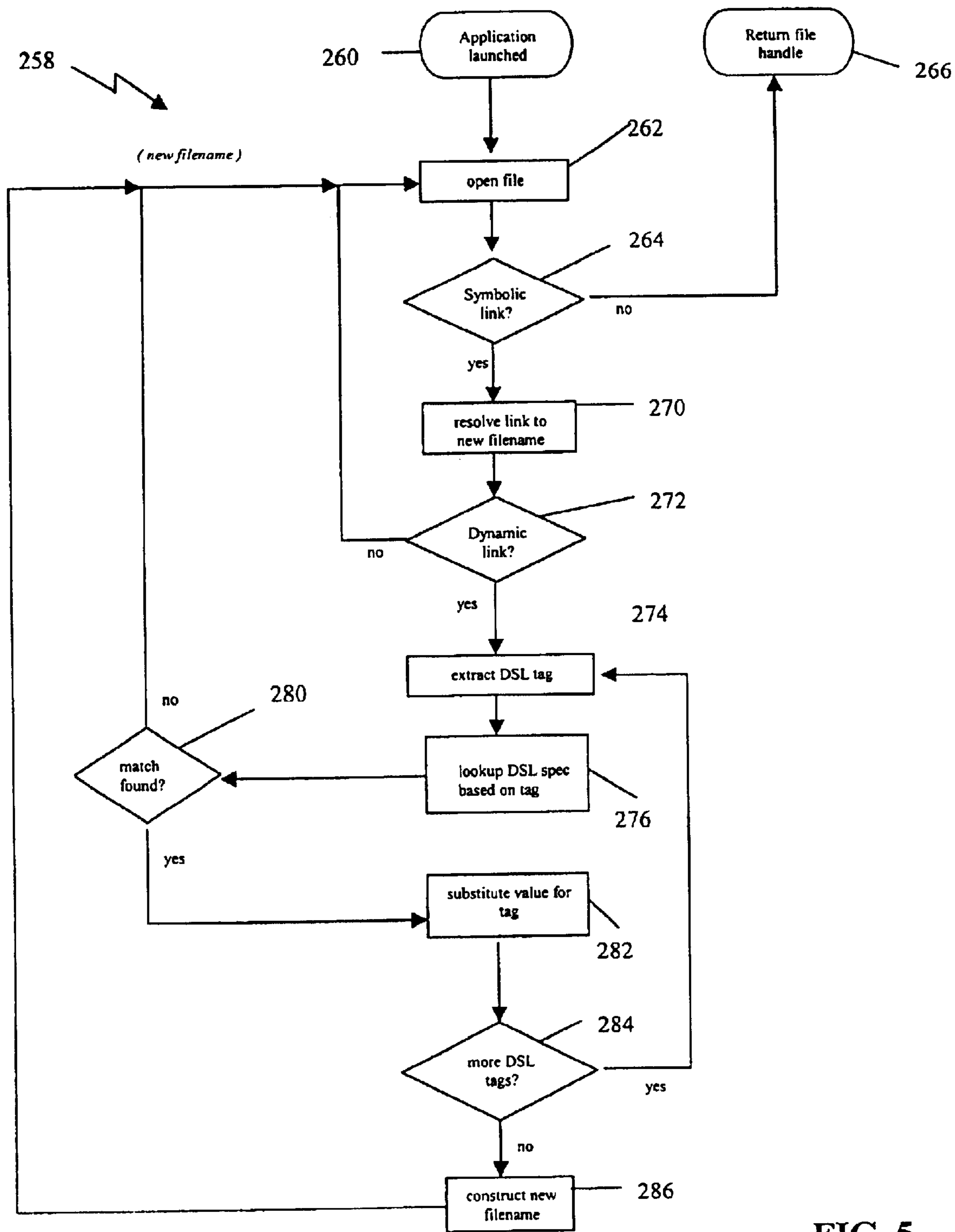
Flowchart of dynamic symbolic link resolution.
