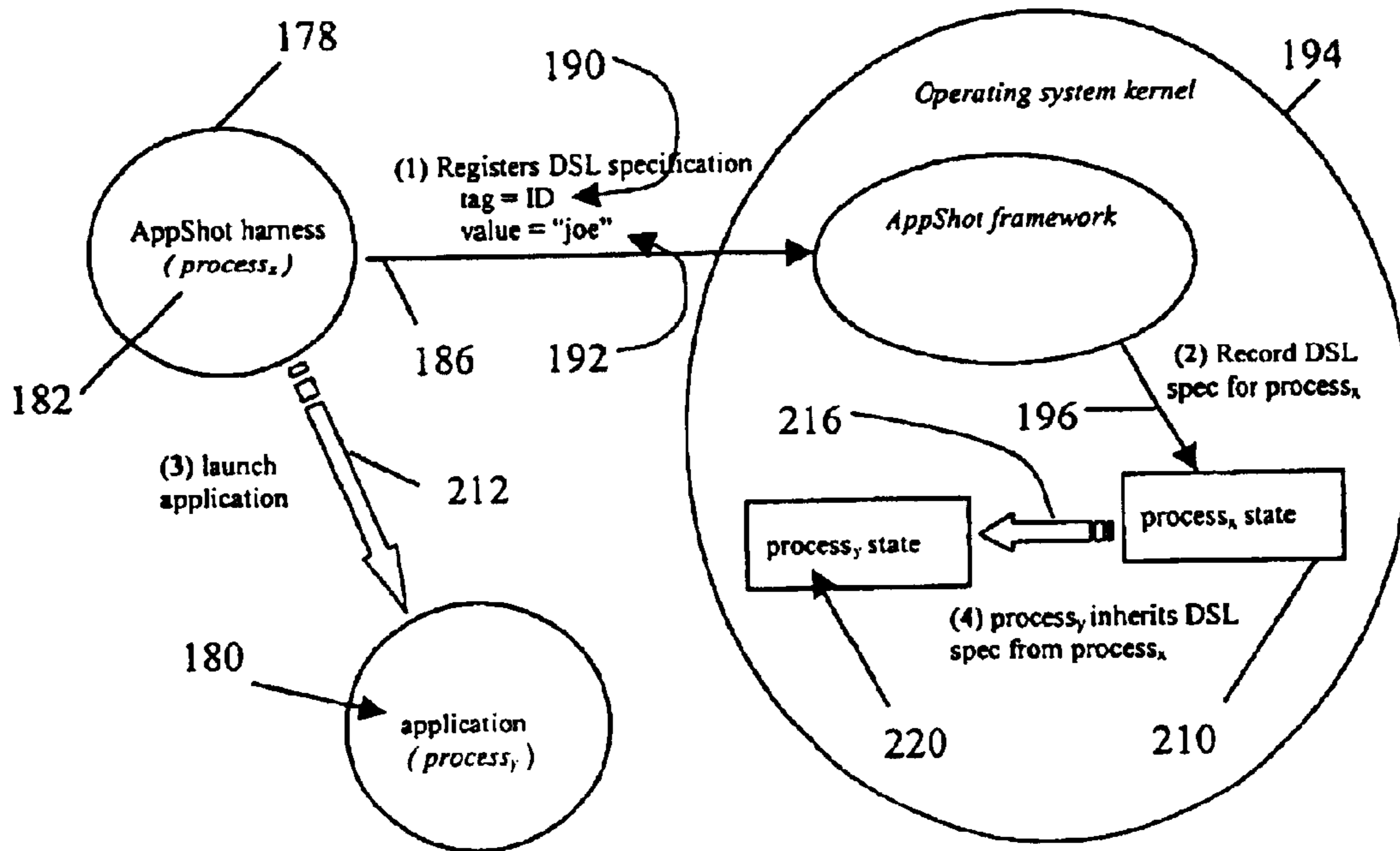
Registration of a dynamic symbolic link specification.
