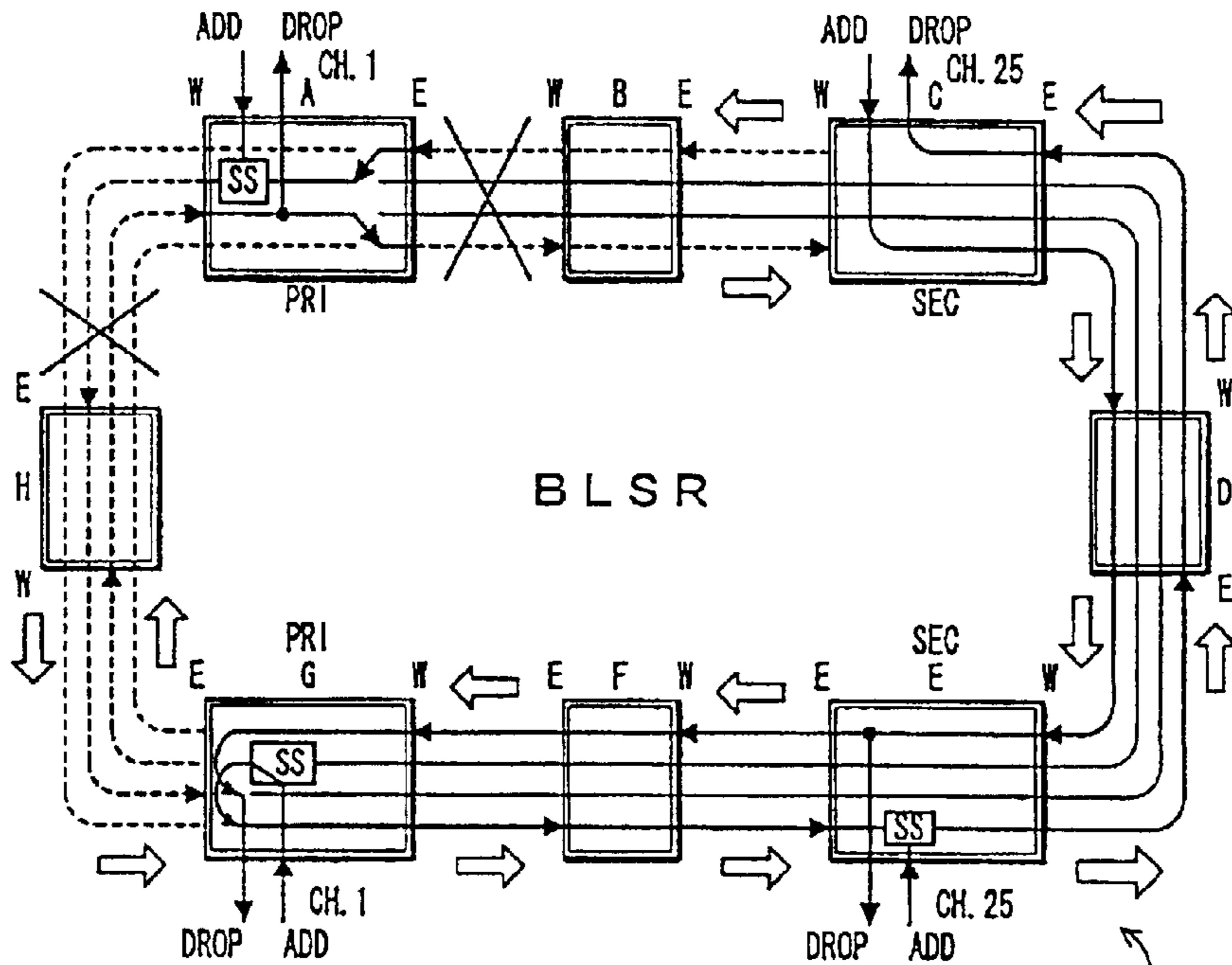
NETWORK STRUCTURE[G] CH. 1
