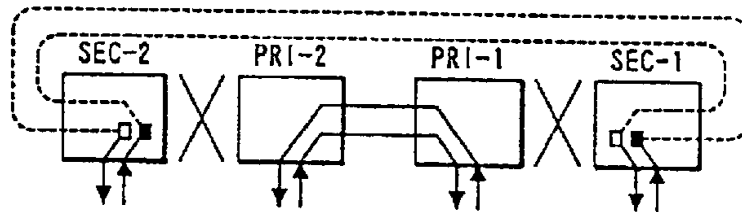
FIG. 34(f) FAILURE POSITION LOOKED FROM SEC-1 N1-R2 FAILURE POSITION LOOKED FROM PRI-1 N3-R4
