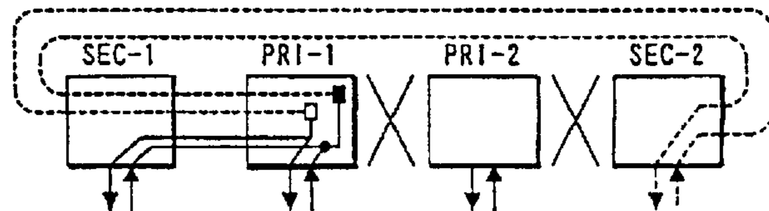
FIG. 31(g) FAILURE POSITION LOOKED FROM SEC-1 N2-R2 FAILURE POSITION LOOKED FROM PRI-1 N2-R2
