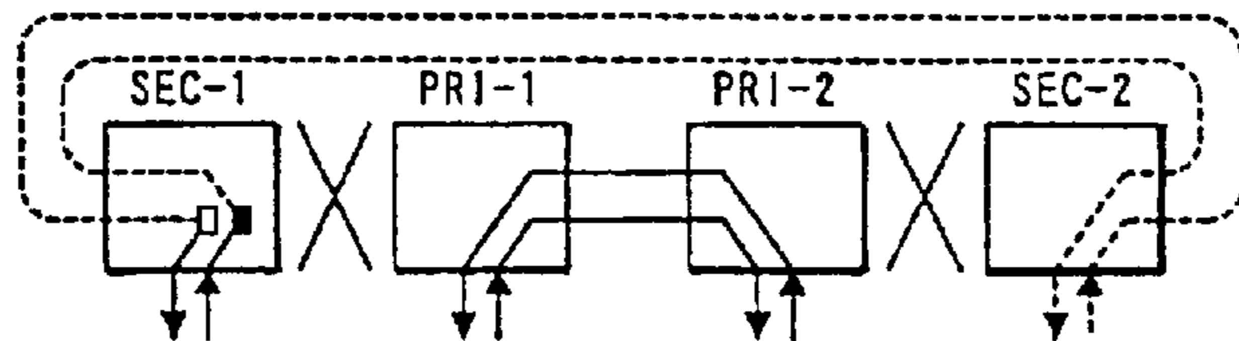
FIG. 31(f) FAILURE POSITION LOOKED FROM SEC-1 N1-R2 FAILURE POSITION LOOKED FROM PRI-1 N3-R4
