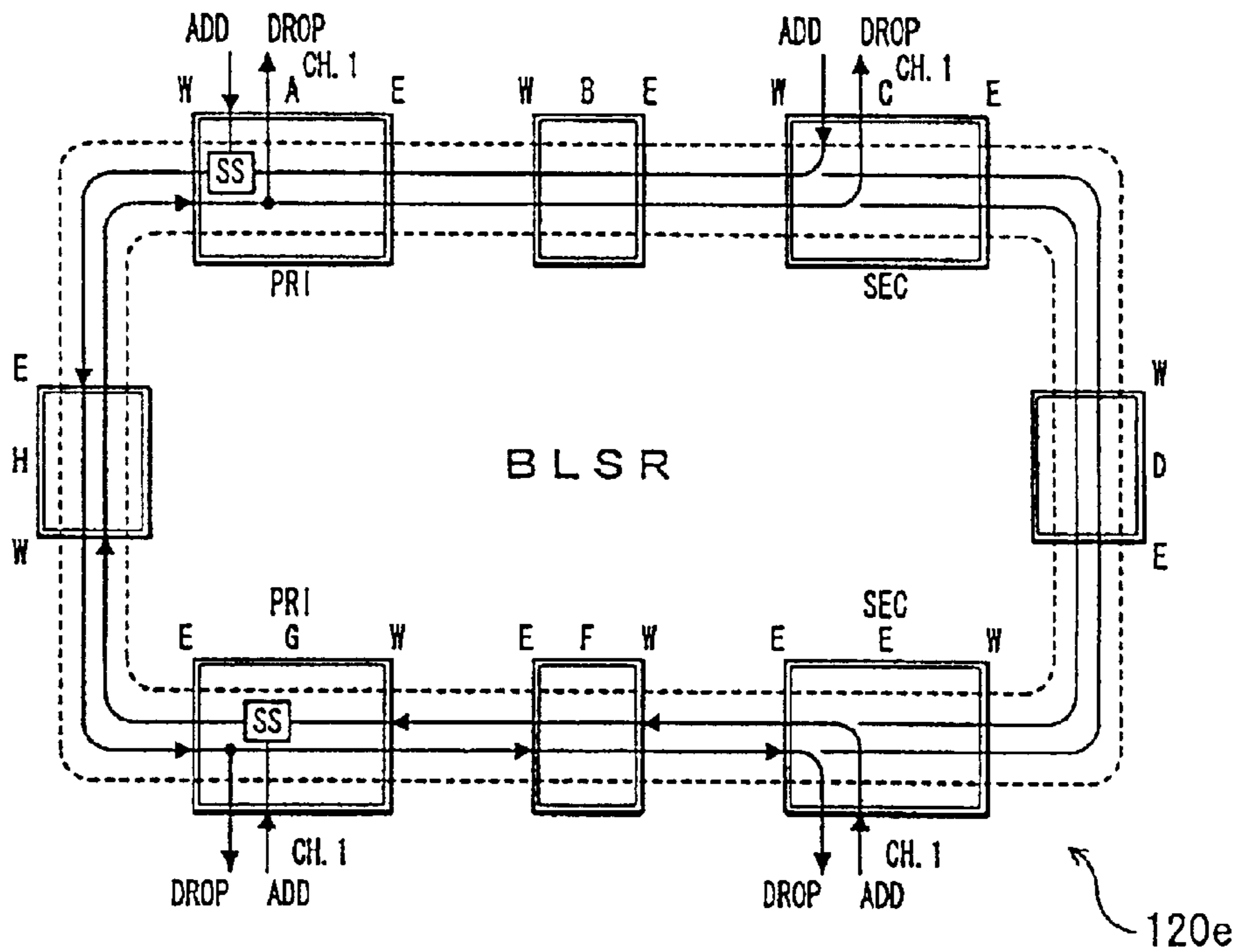
NETWORK STRUCTURE[G] CH. 1
