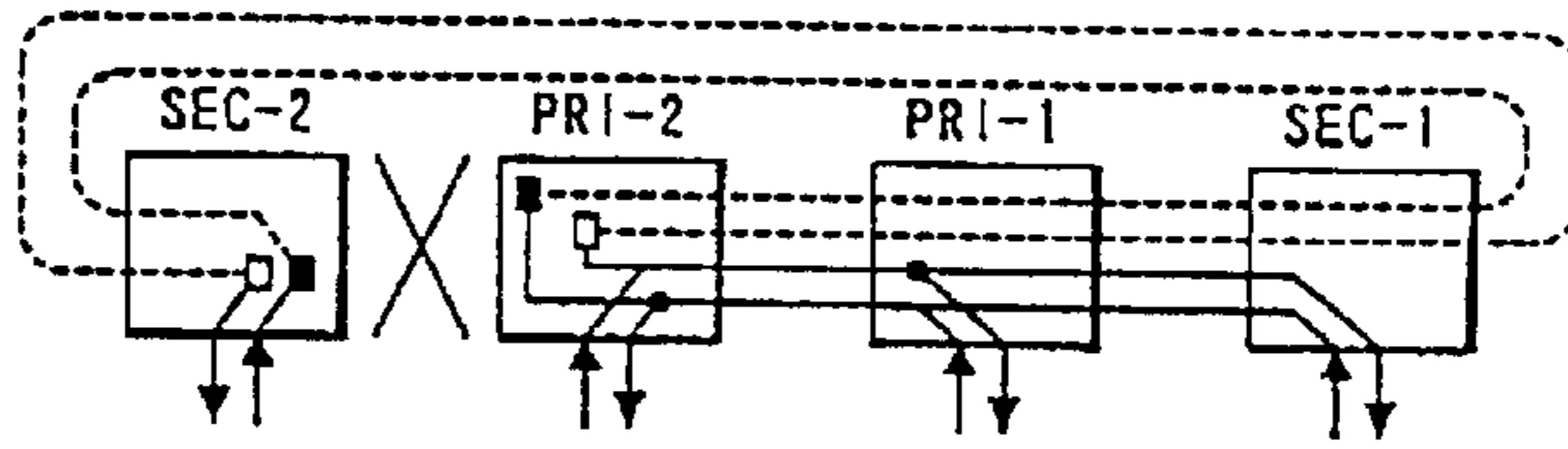
FIG. 34(h) FAILURE POSITION LOOKED FROM SEC-1 N3-R2 FAILURE POSITION LOOKED FROM PRI-1 N3-R2
