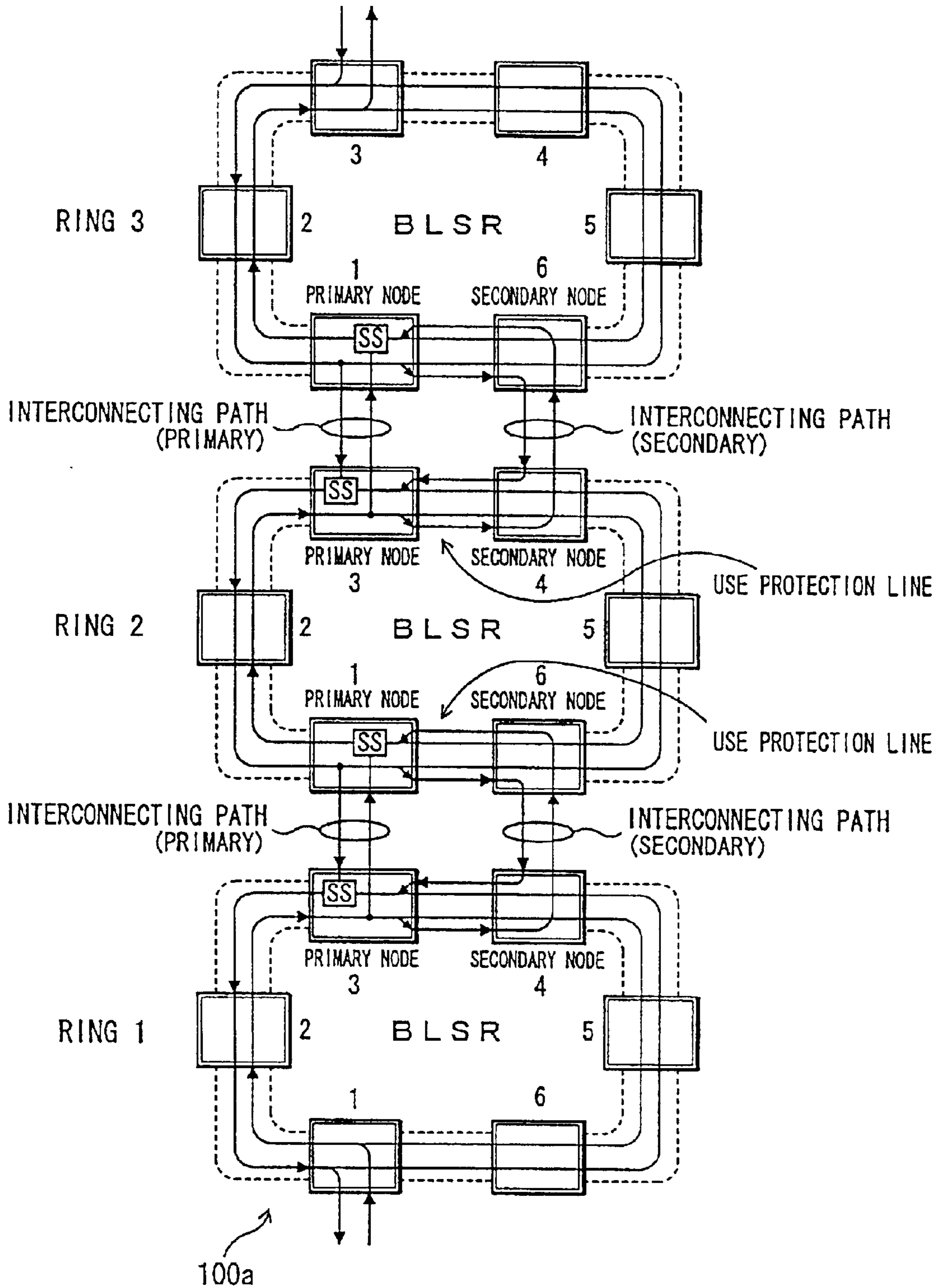
DCP-DCP (DOUBLE-SIDED DCP) STRUCTURE
