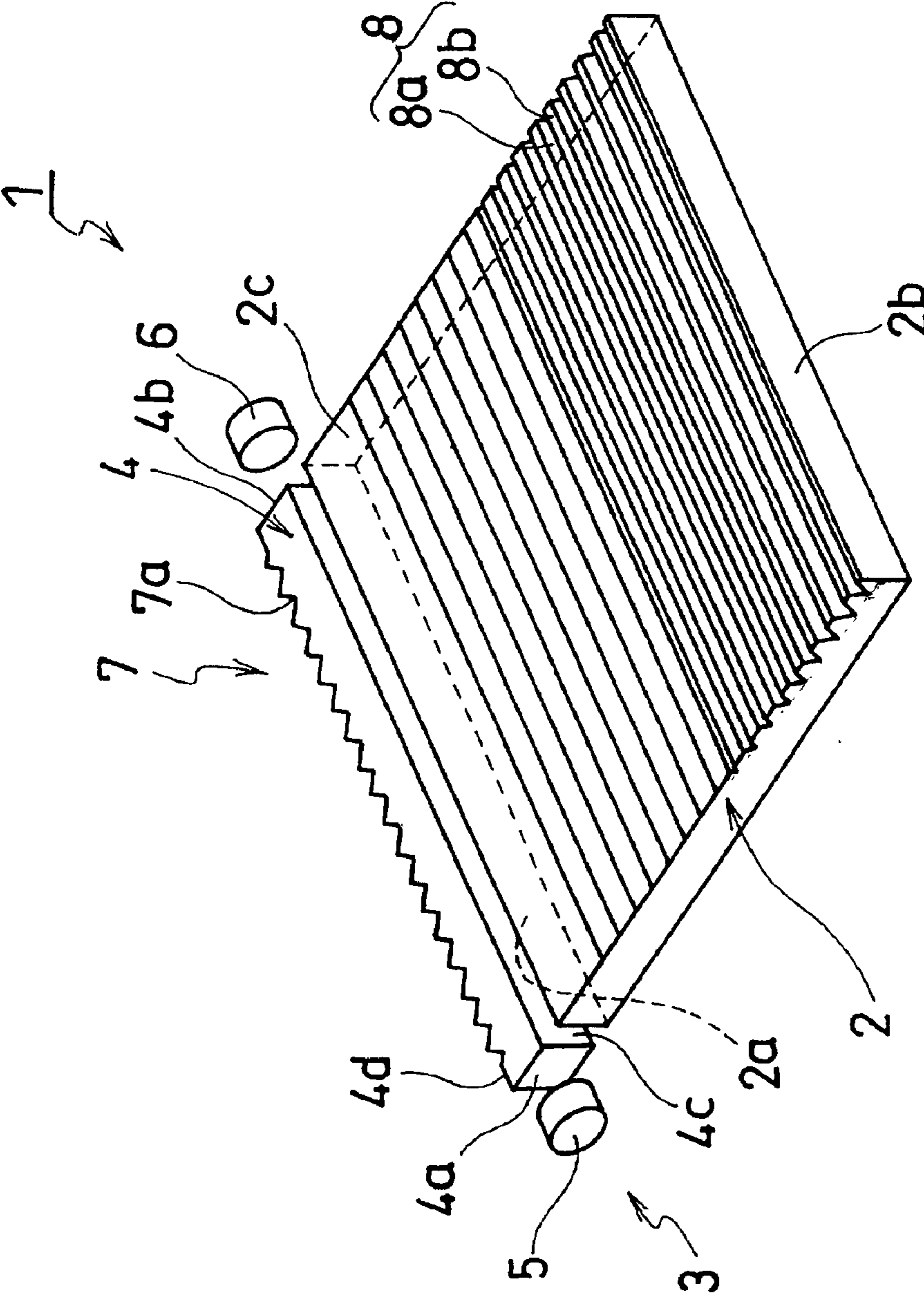
Fig. 6 Prior Art
