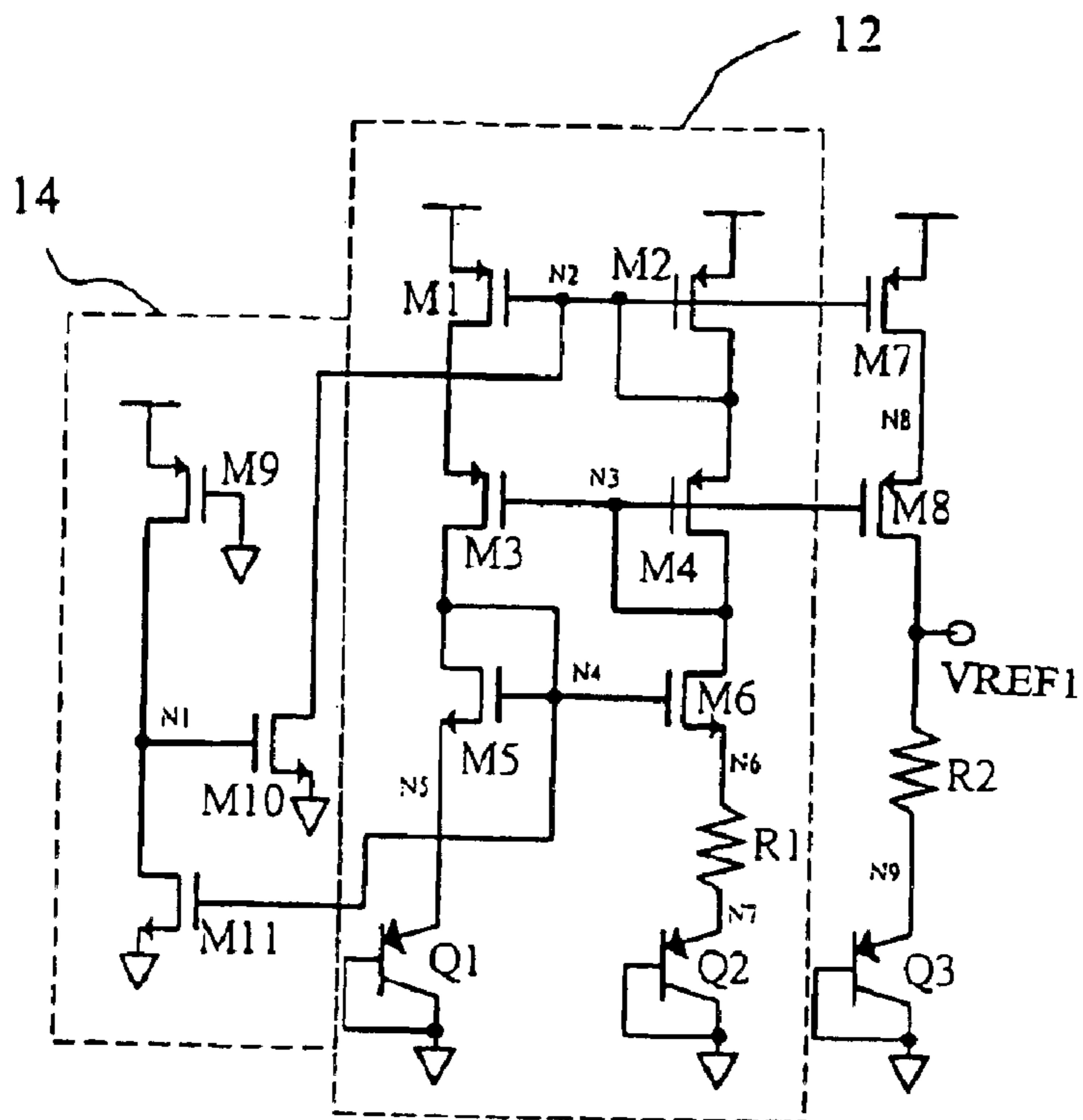
Fig 1 (Prior art)
