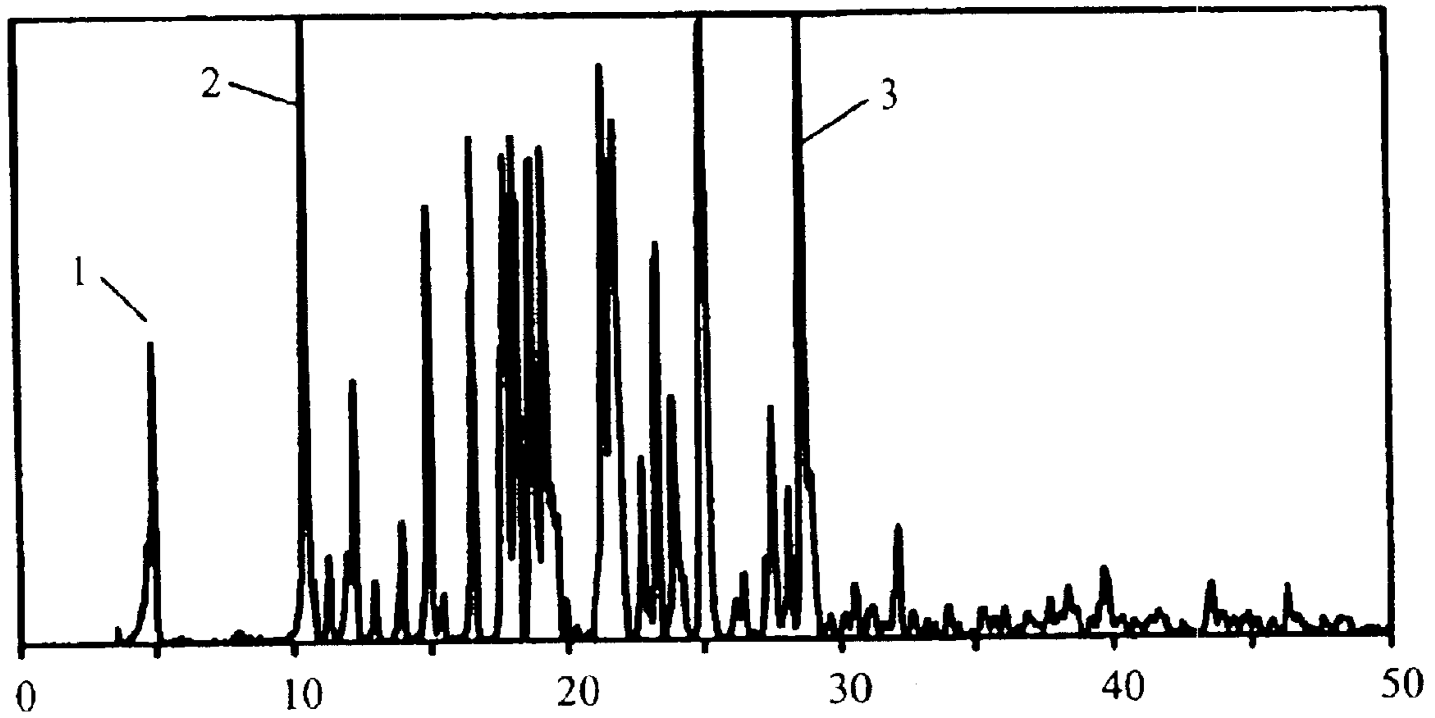
Figure 1 (alpha form)
