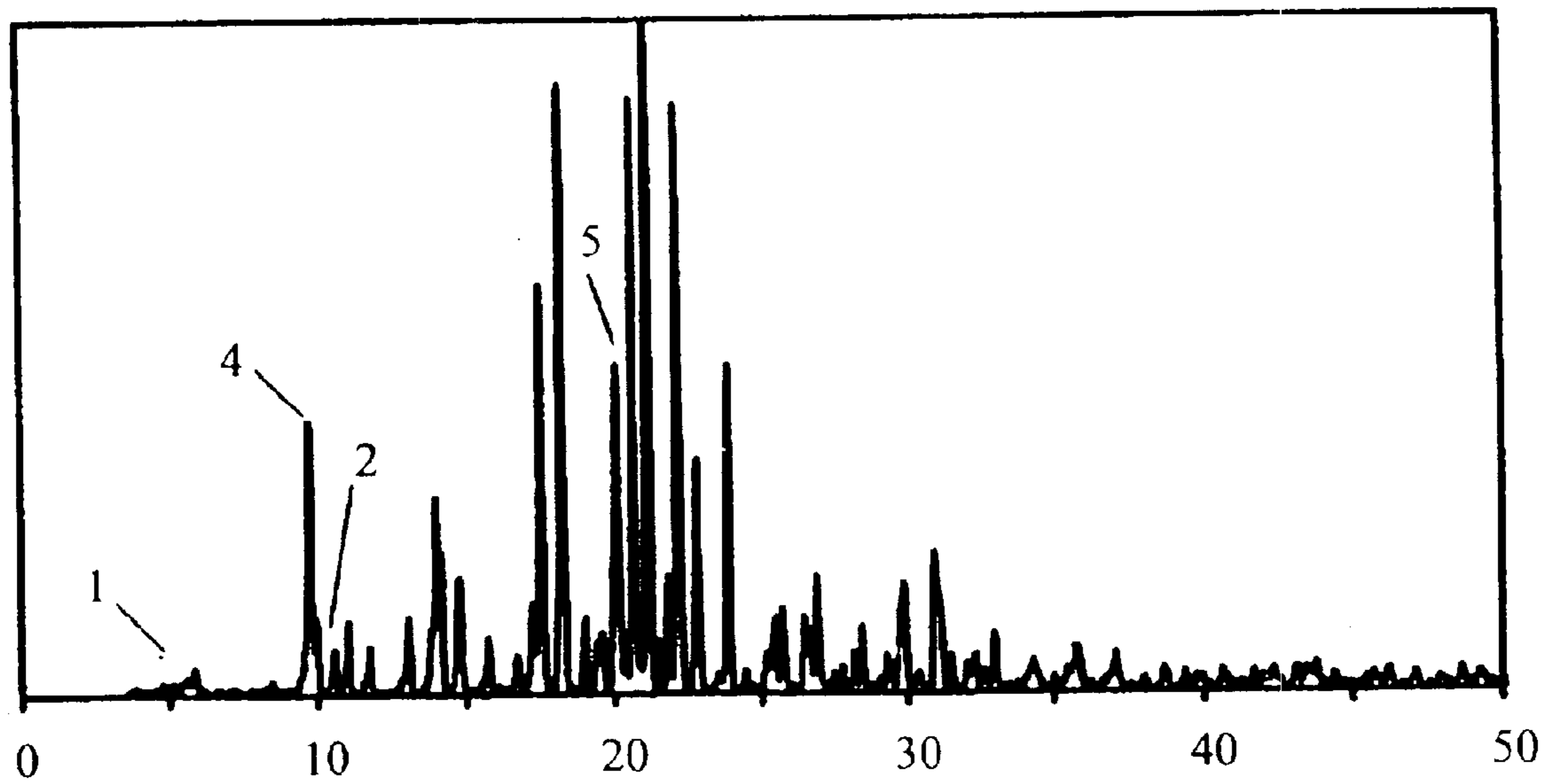
Figure 2 (beta form)
