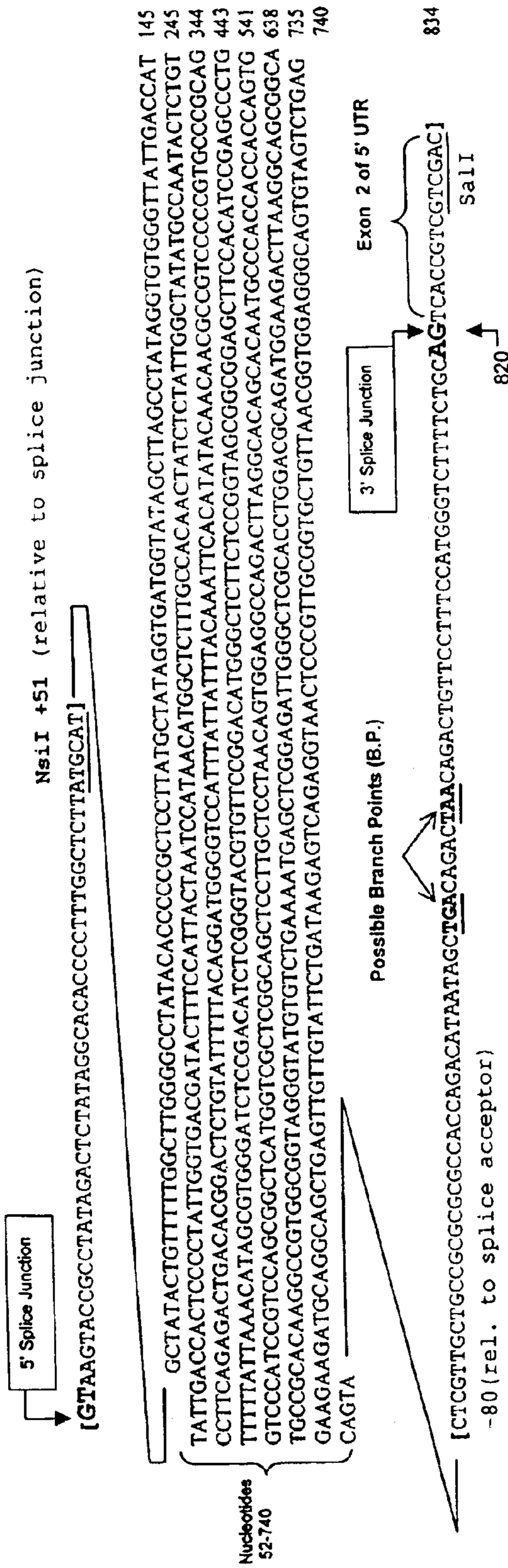
FIG. 1A : Full length Intron A = 820 bp
