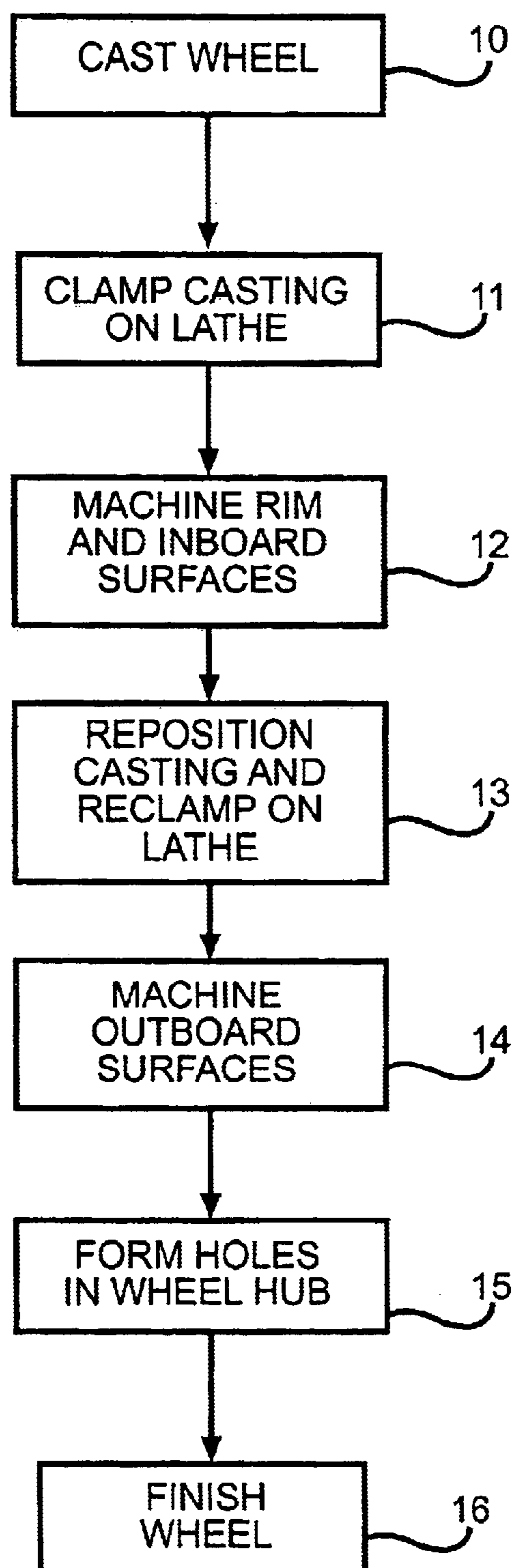
FIG.1 (PRIOR ART)
