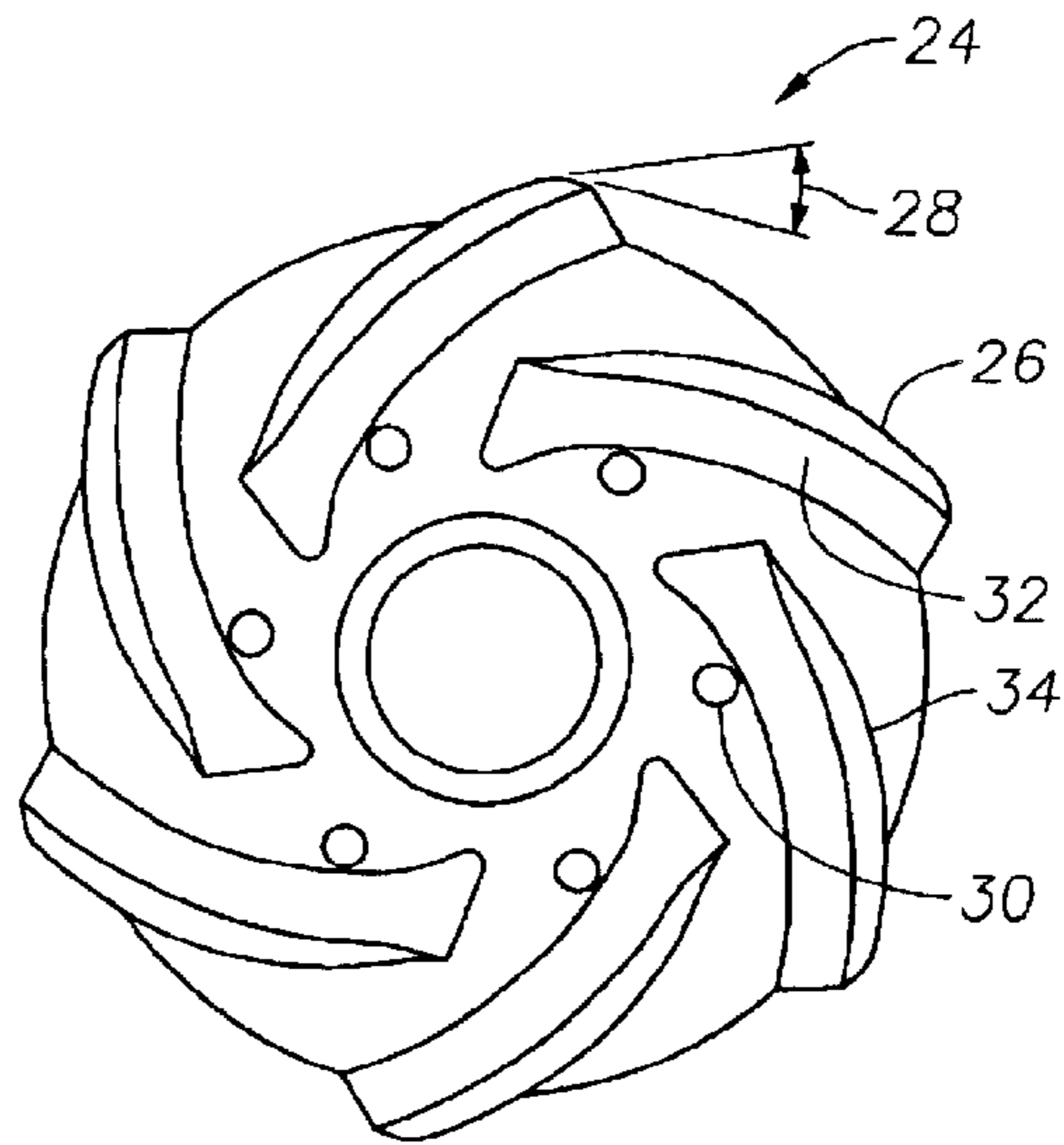
Fig. 2 (Prior Art)
