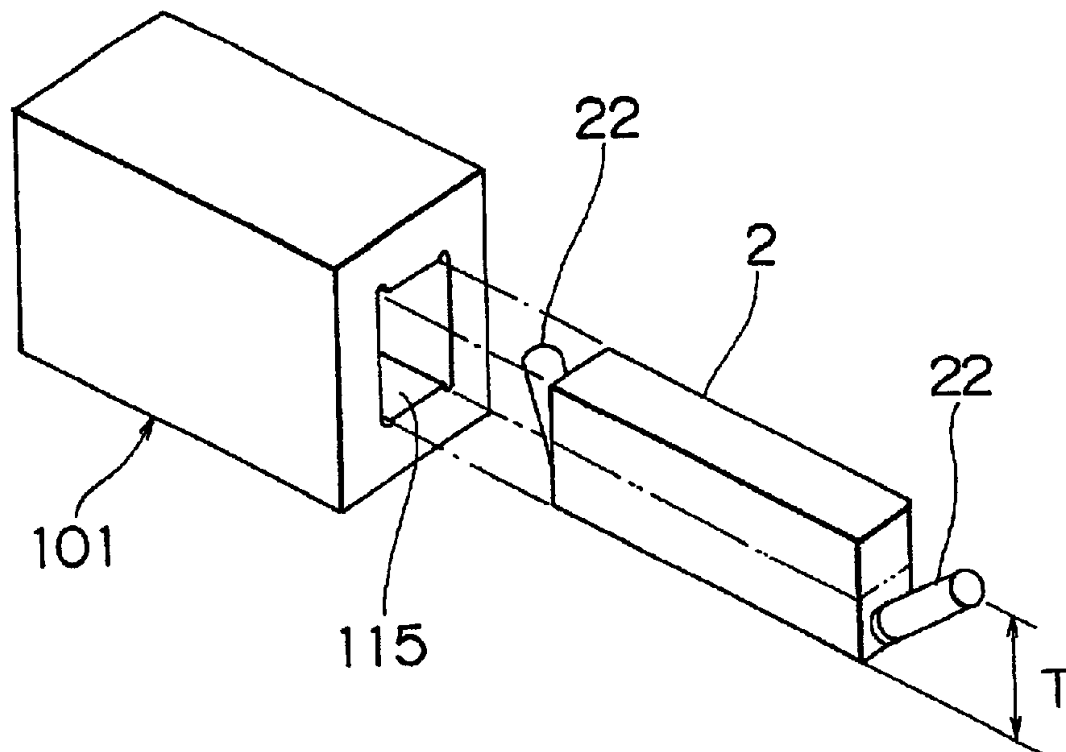
FIG. 36 RELATED ART
