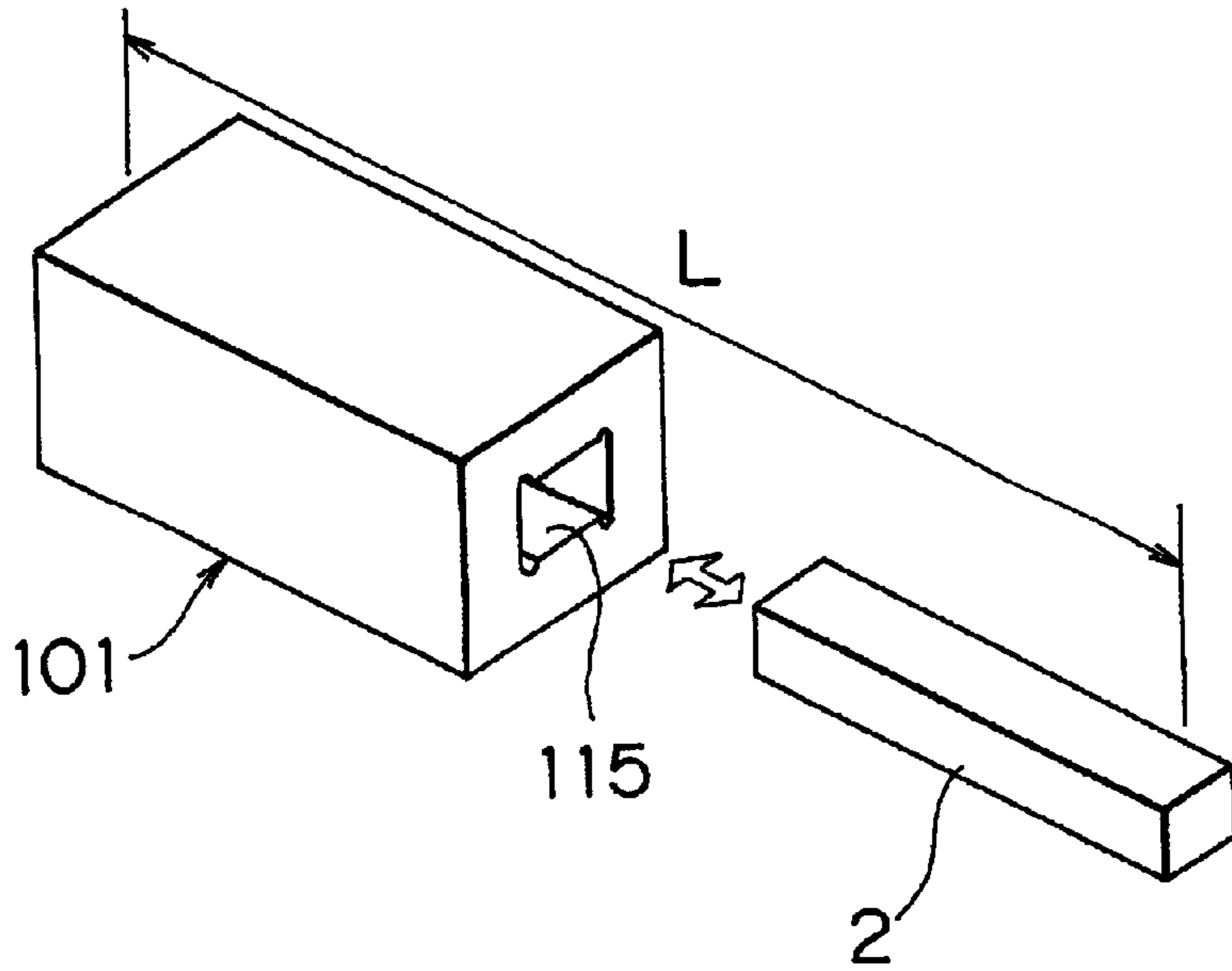
FIG. 35 RELATED ART
