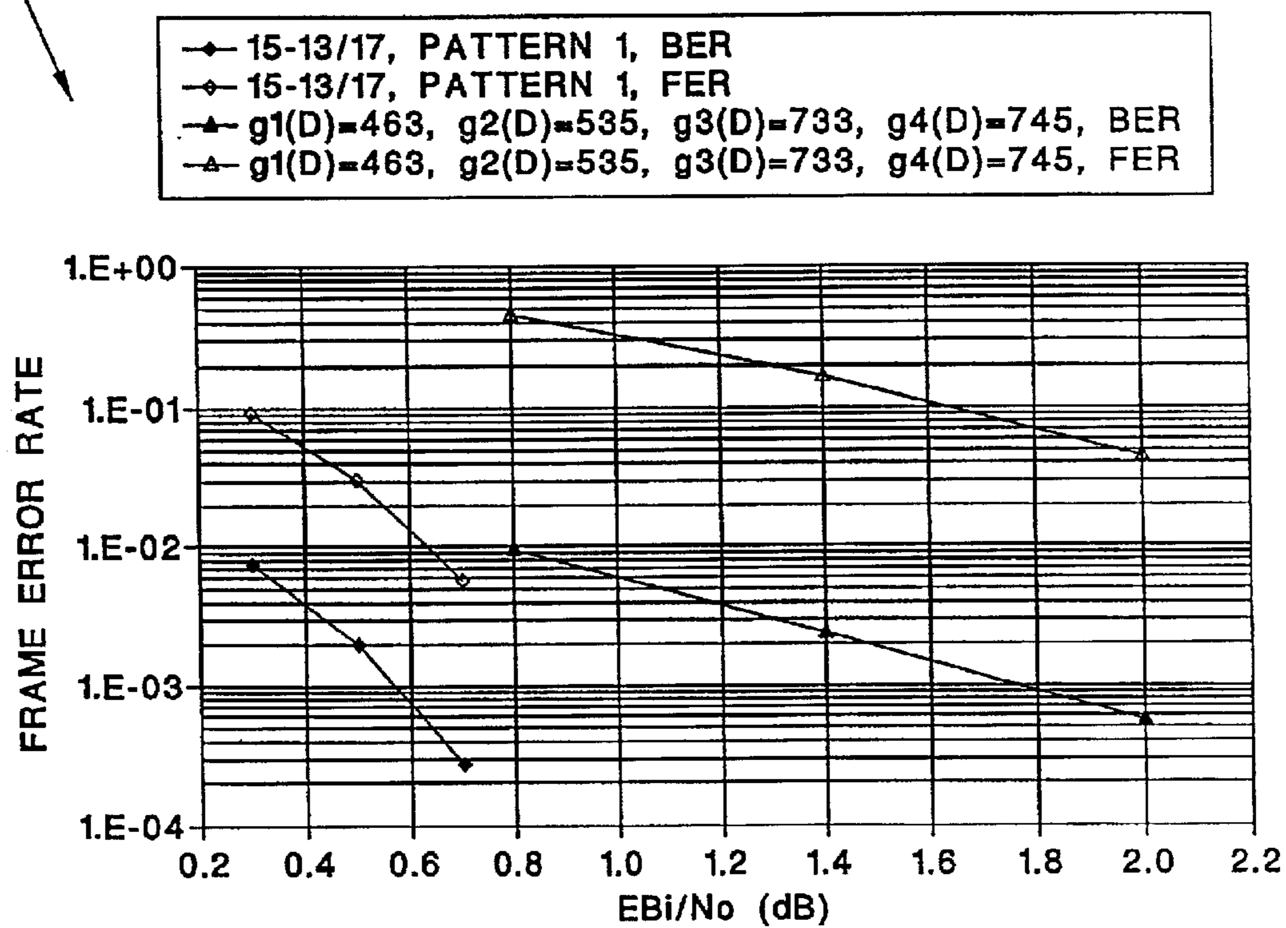
FIG. 32 COMPARISON OF RATE 1/4 FER-OPTIMIZED TURBO CODE VS CONVOLUTIONAL CODE, FRAME SIZE=512
