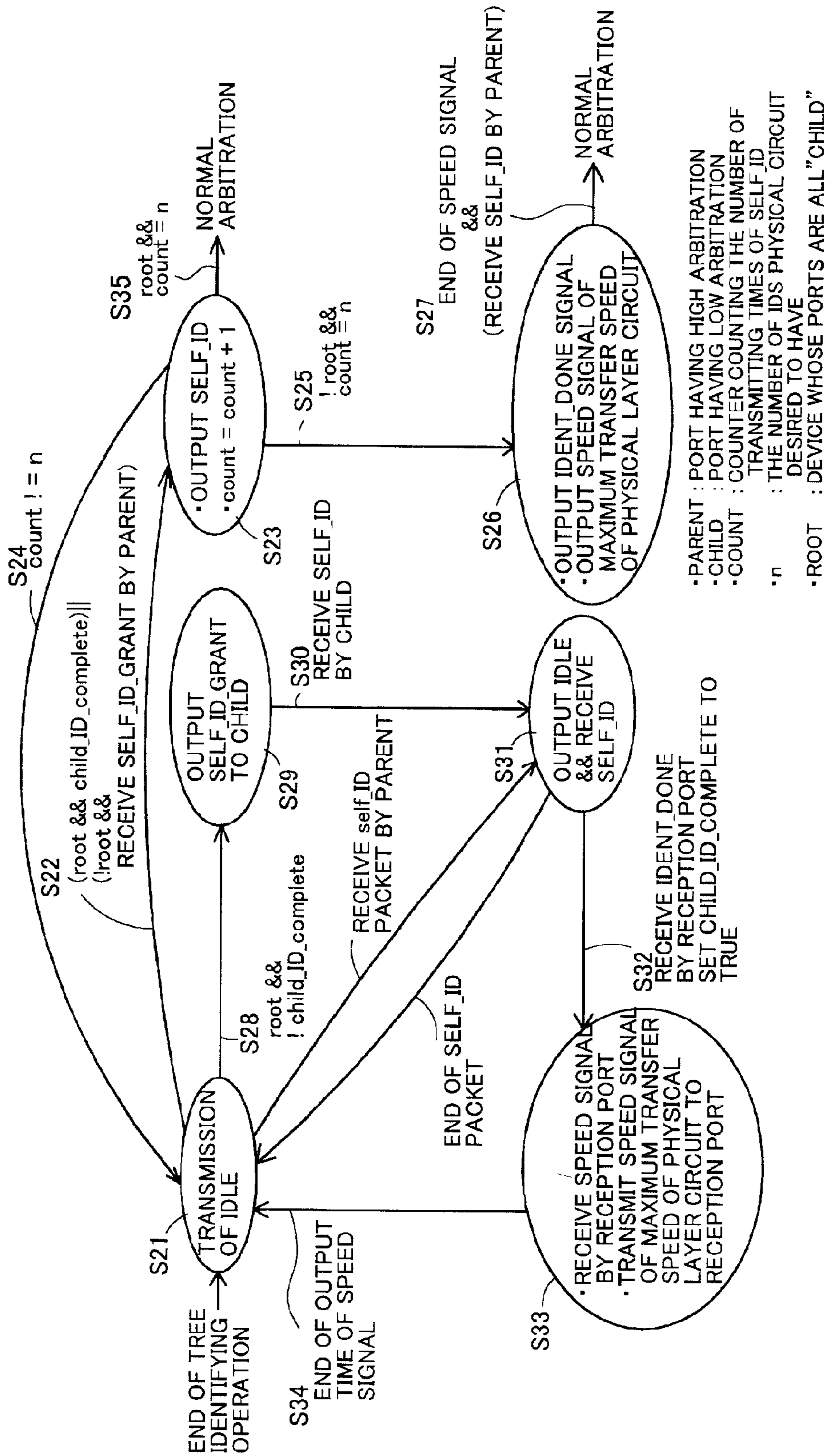
FIG. 16 STATE TRANSITION DIAGRAM SHOWING SELF-IDENTIFYING OPERATION IN FIRST CONSTRUCTION EXAMPLE OF SECOND EMBODIMENT
