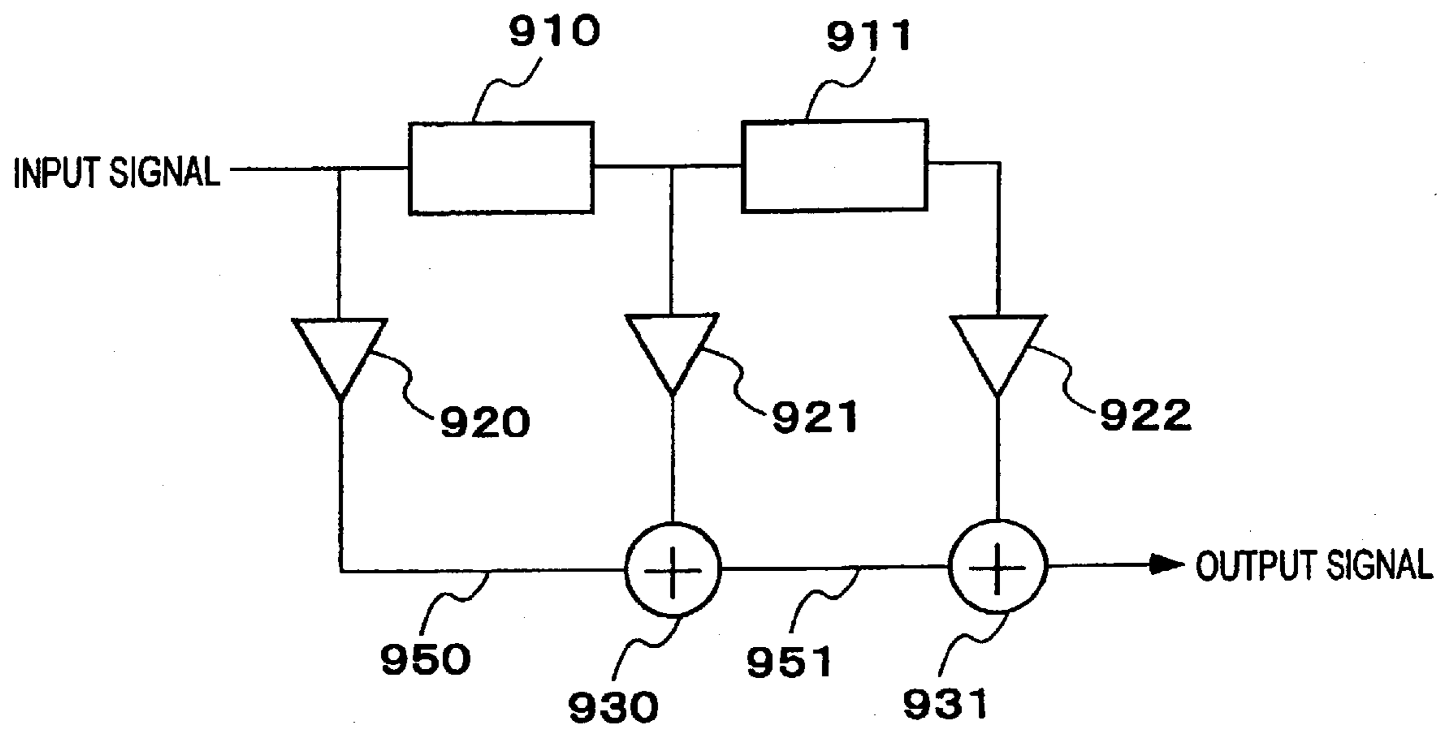
FIG.9 (PRIOR ART)
