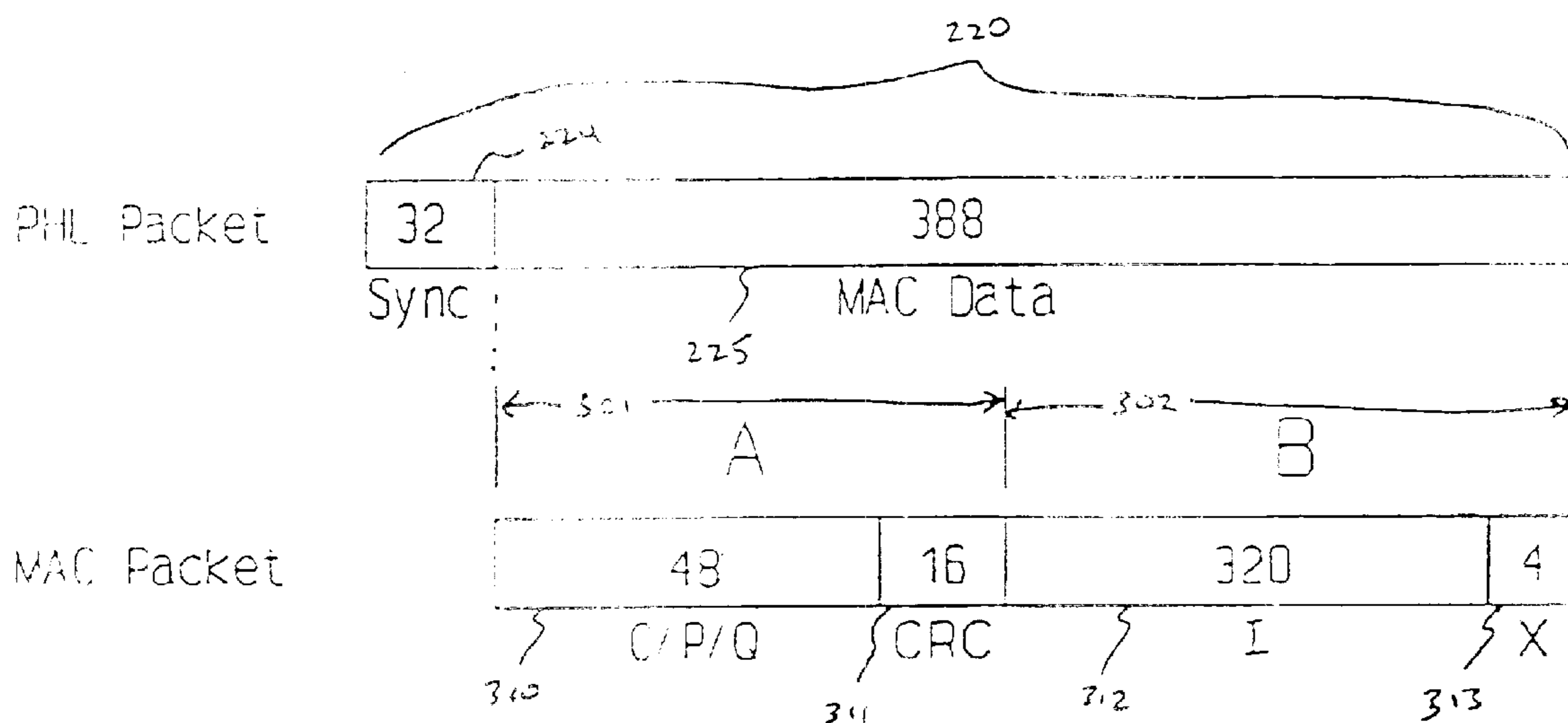
Fig. 3 DECT Medium Access Control, MAC
