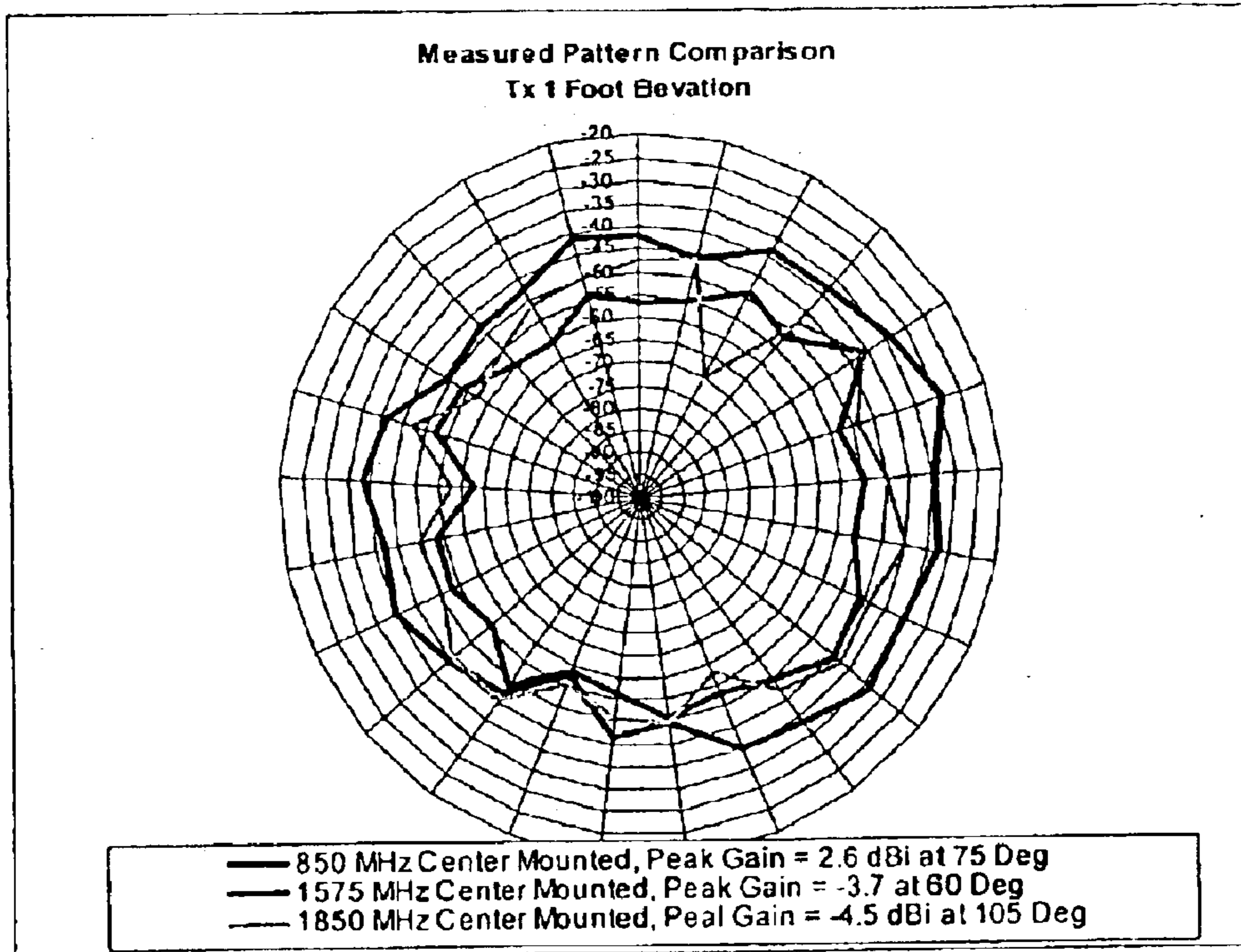
FIG 22 Patterns and Absolute Gain
