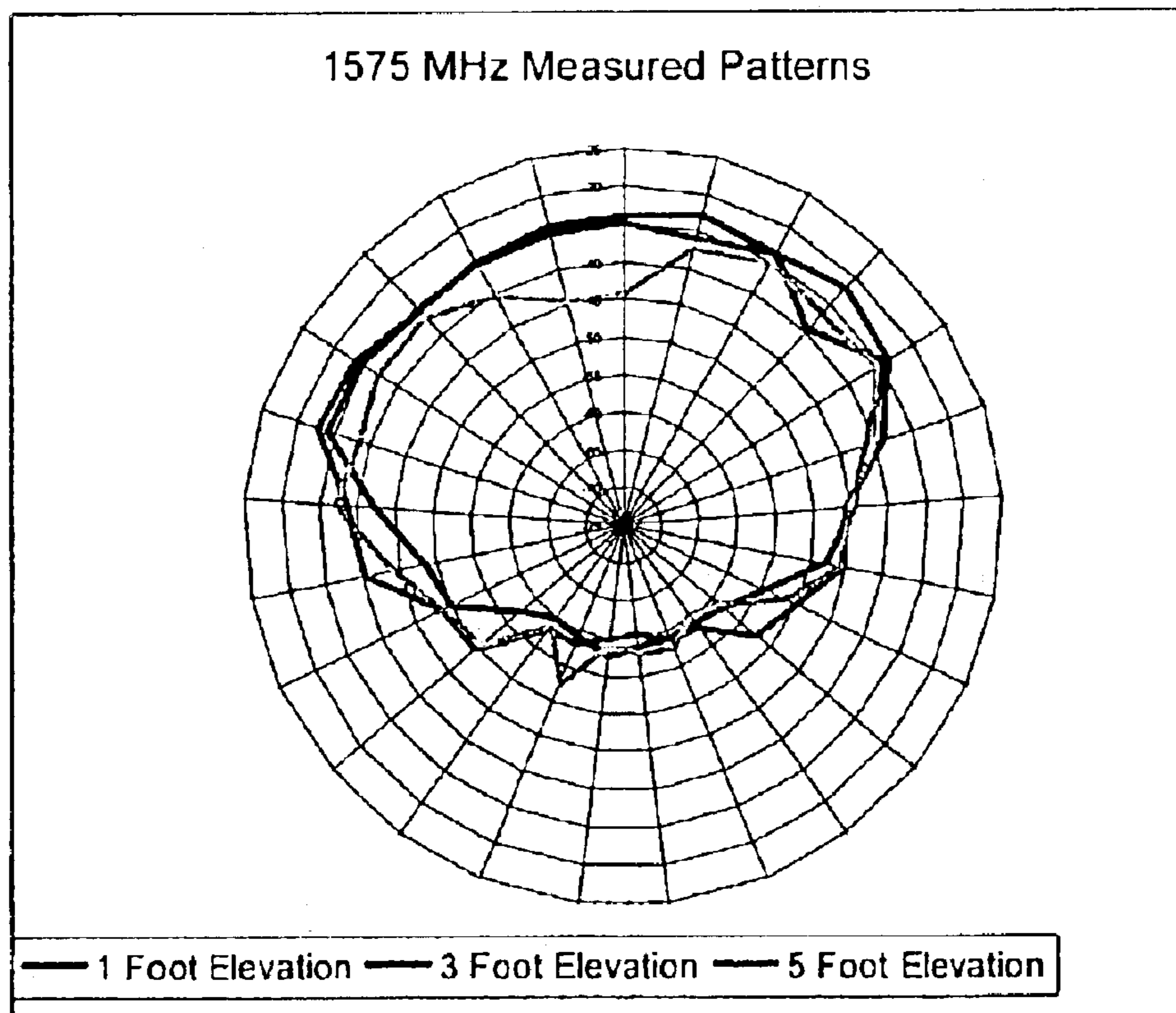
FIG 15 Patterns at 1575 MHz
