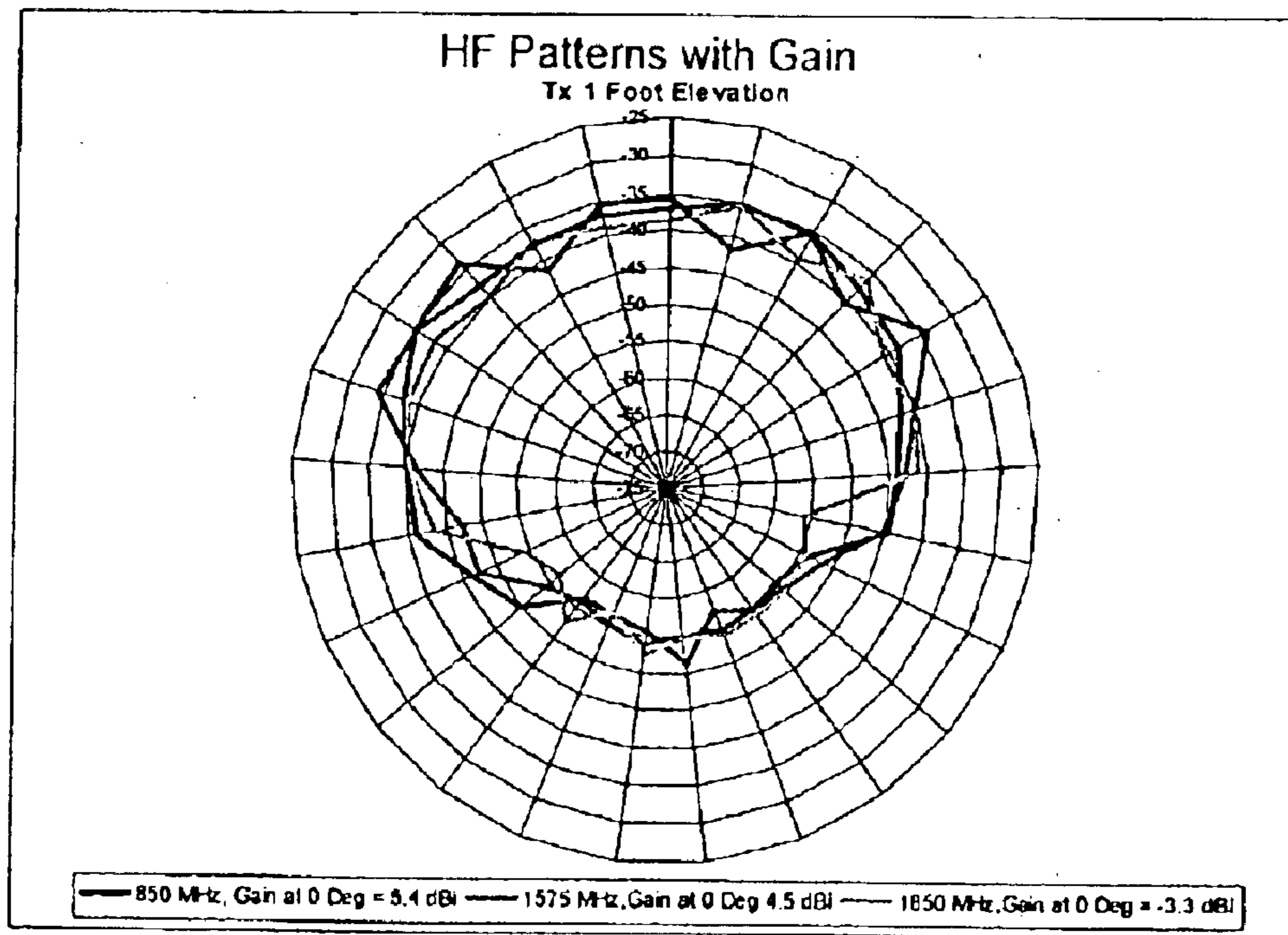
FIG 17 Measured Patterns with Gain
