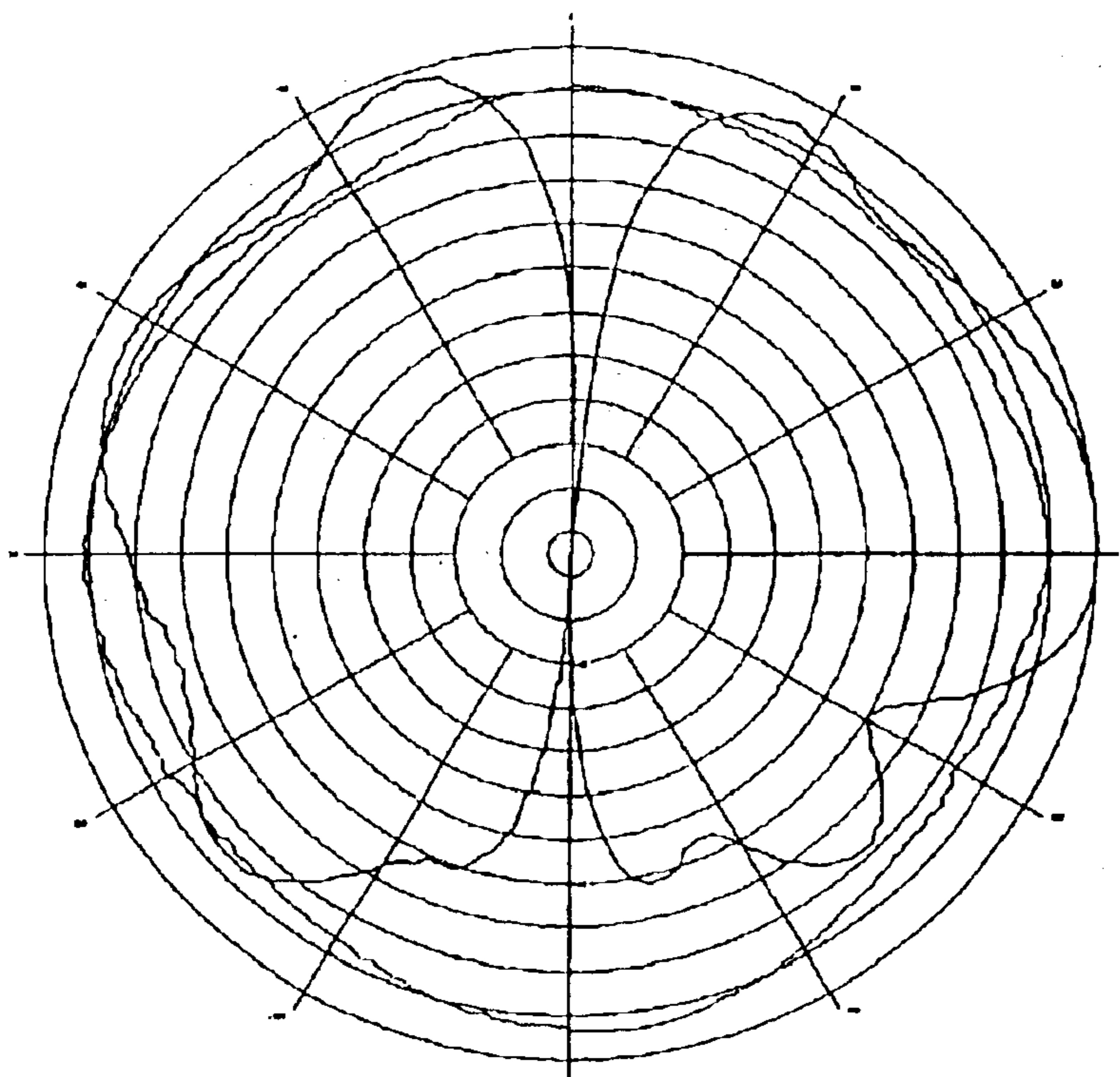
FIG 10 Azimuth and Elevation Pattern 1800 MHz
