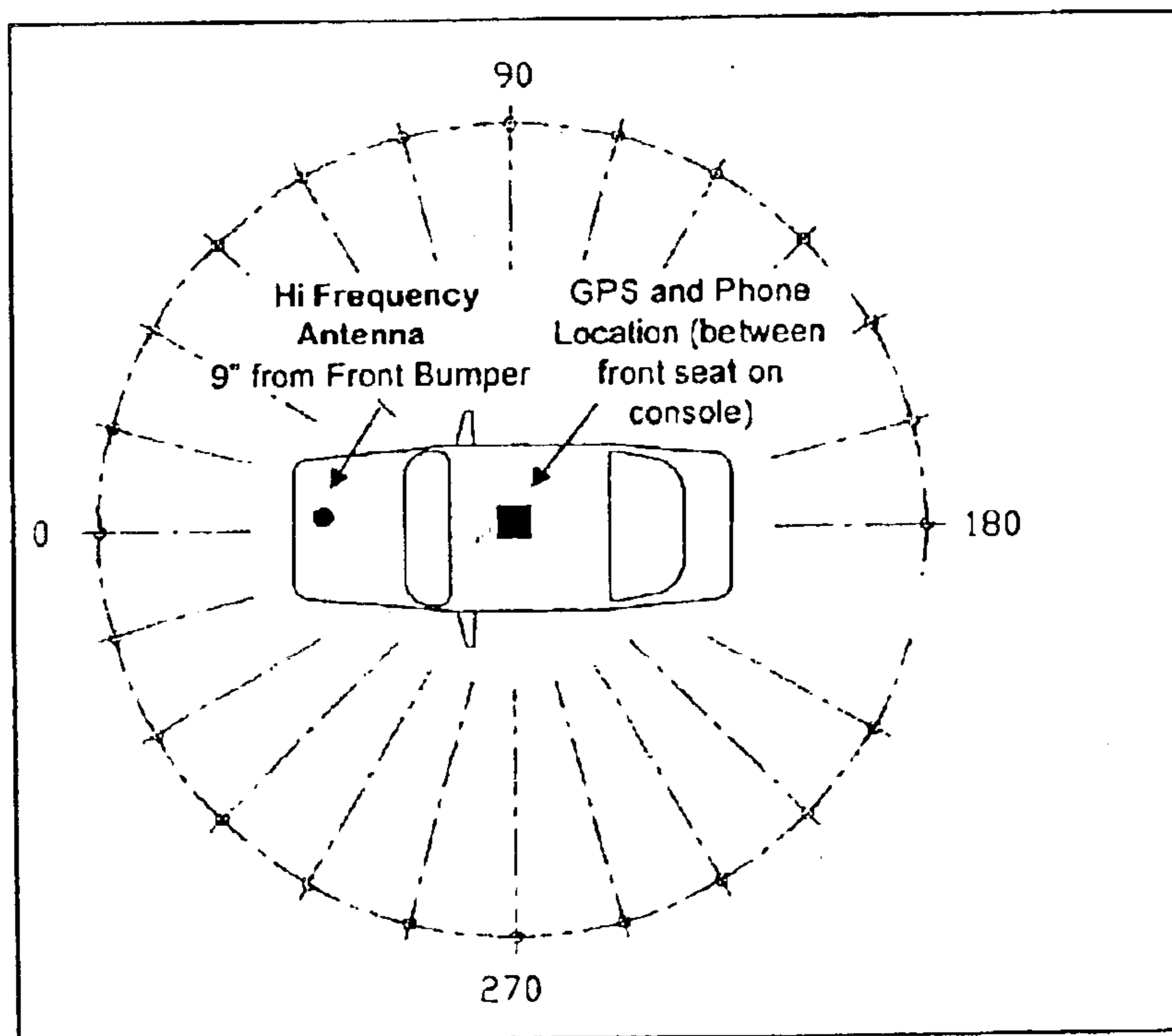
FIG 21 Test Range Setup
