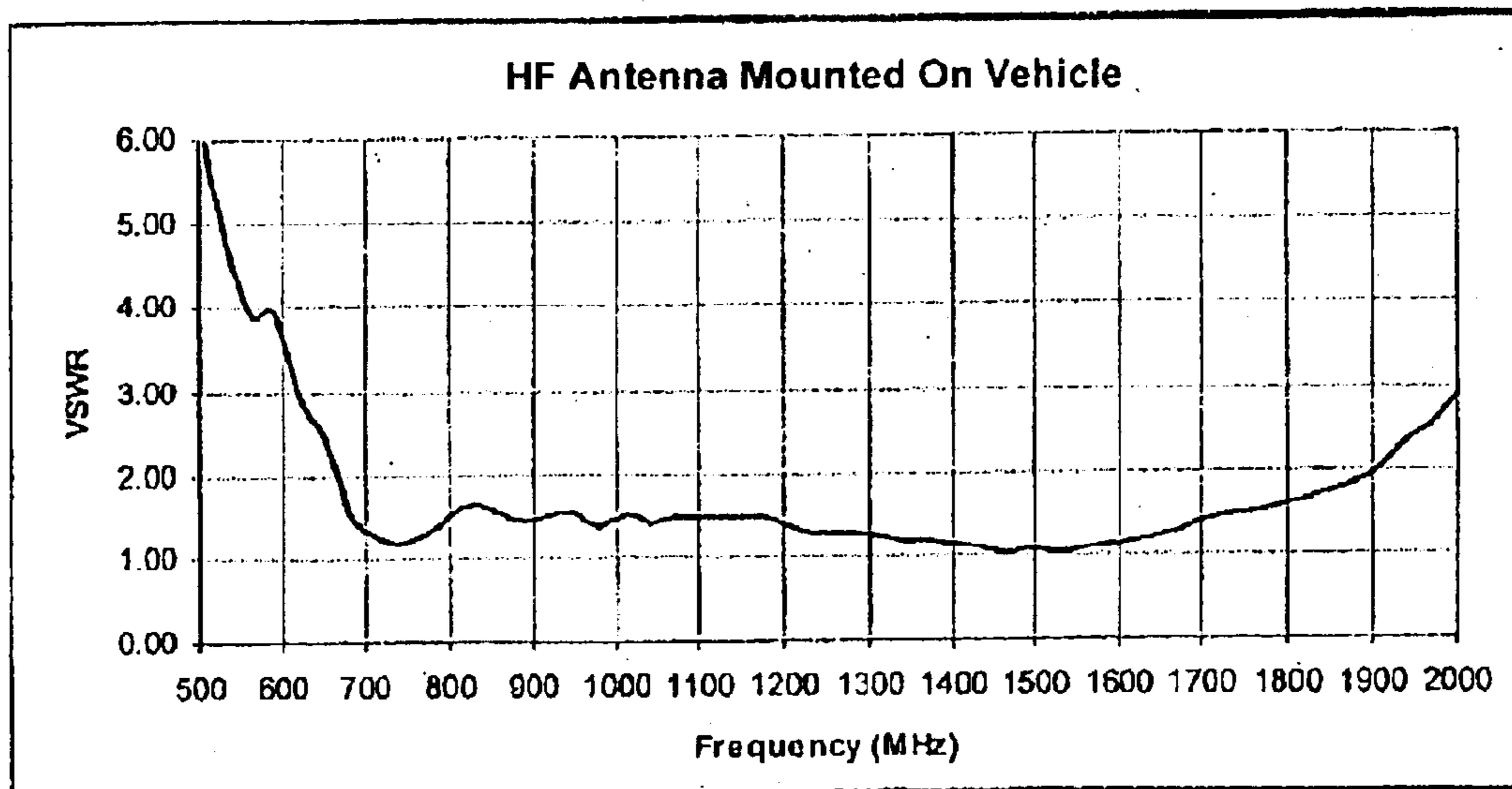
FIG13 Measured VSWR
