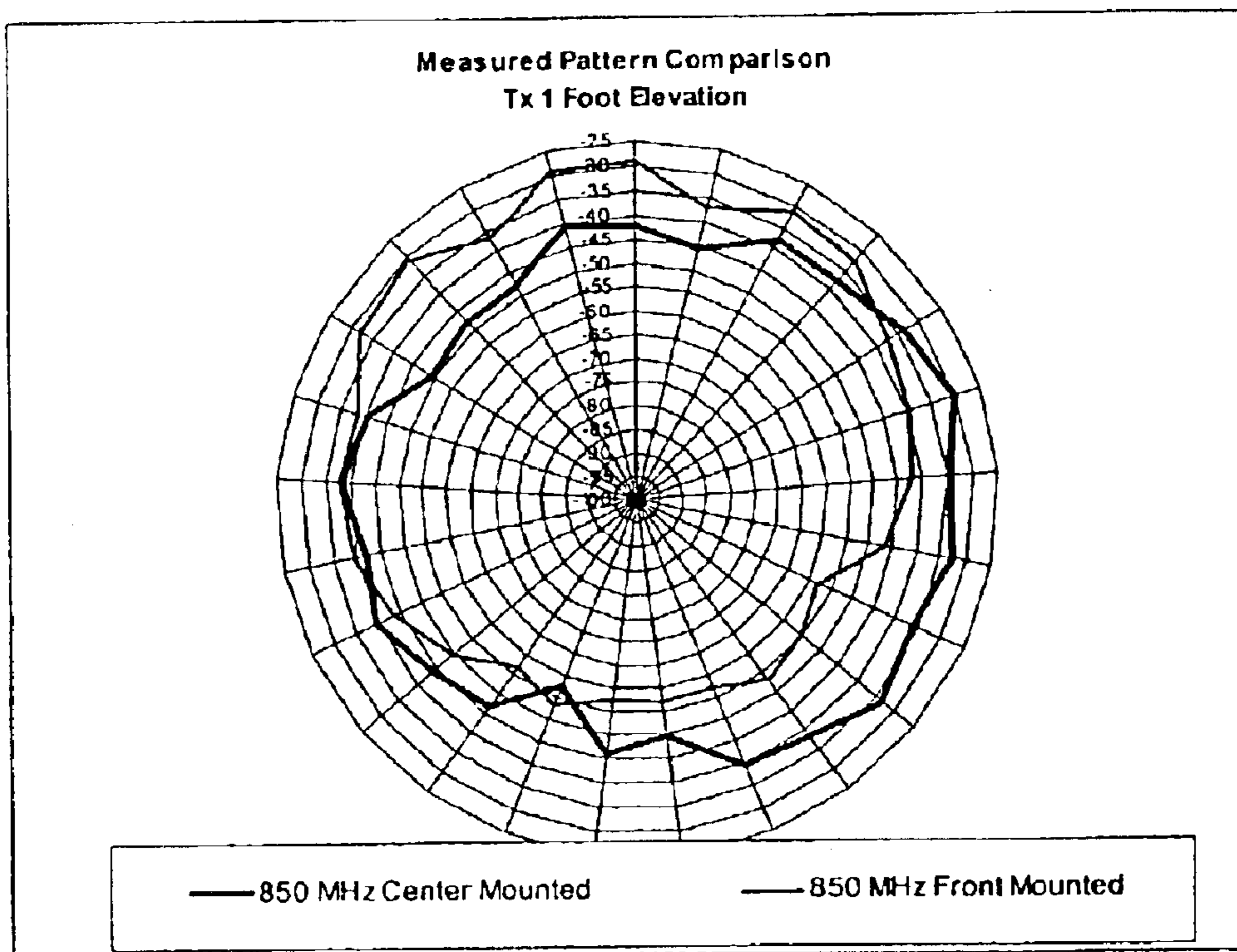
FIG 23 Comparison of Antenna Location at 850 MHz
