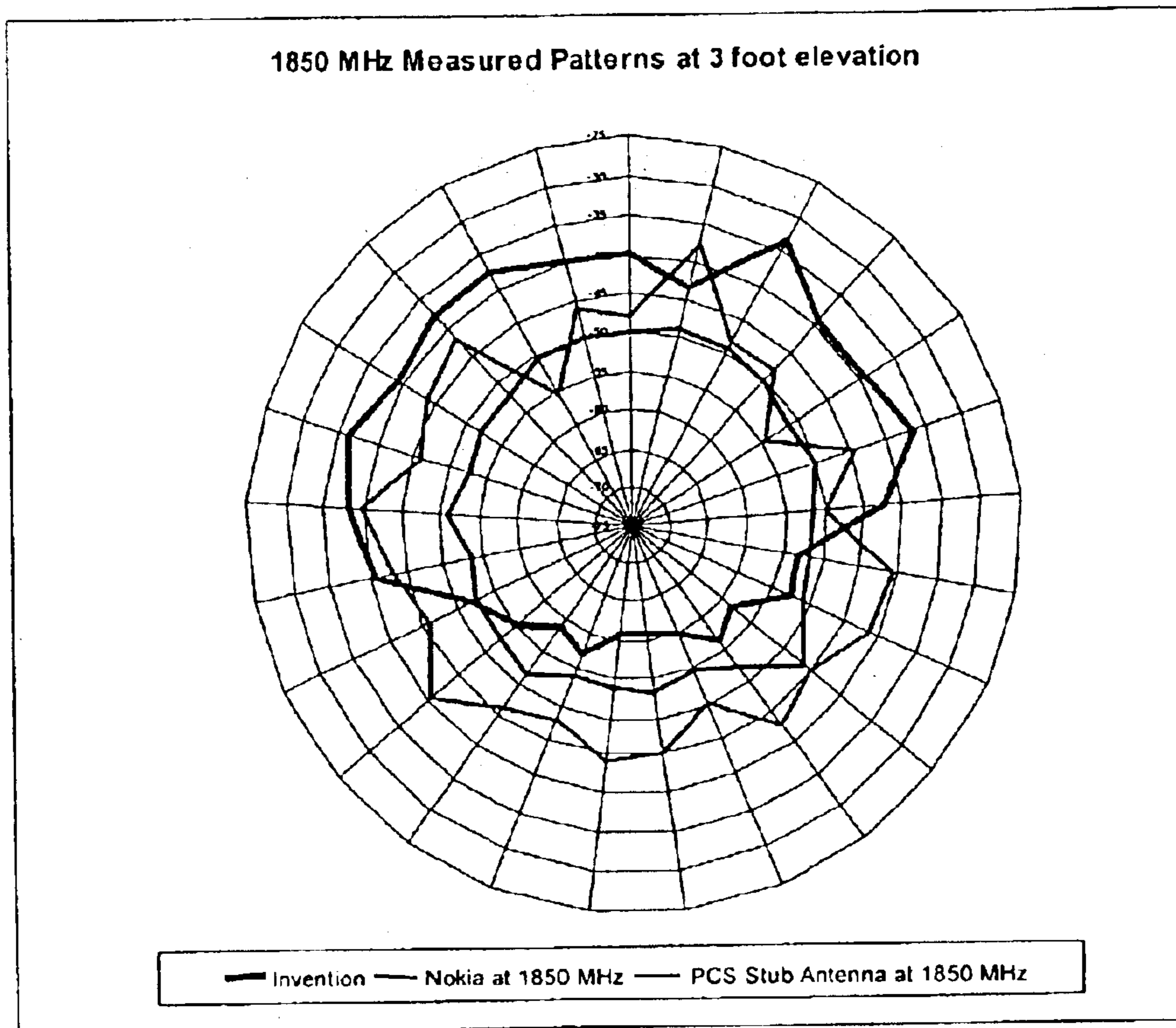
FIG 20 Data Comparison at 1850 MHz
