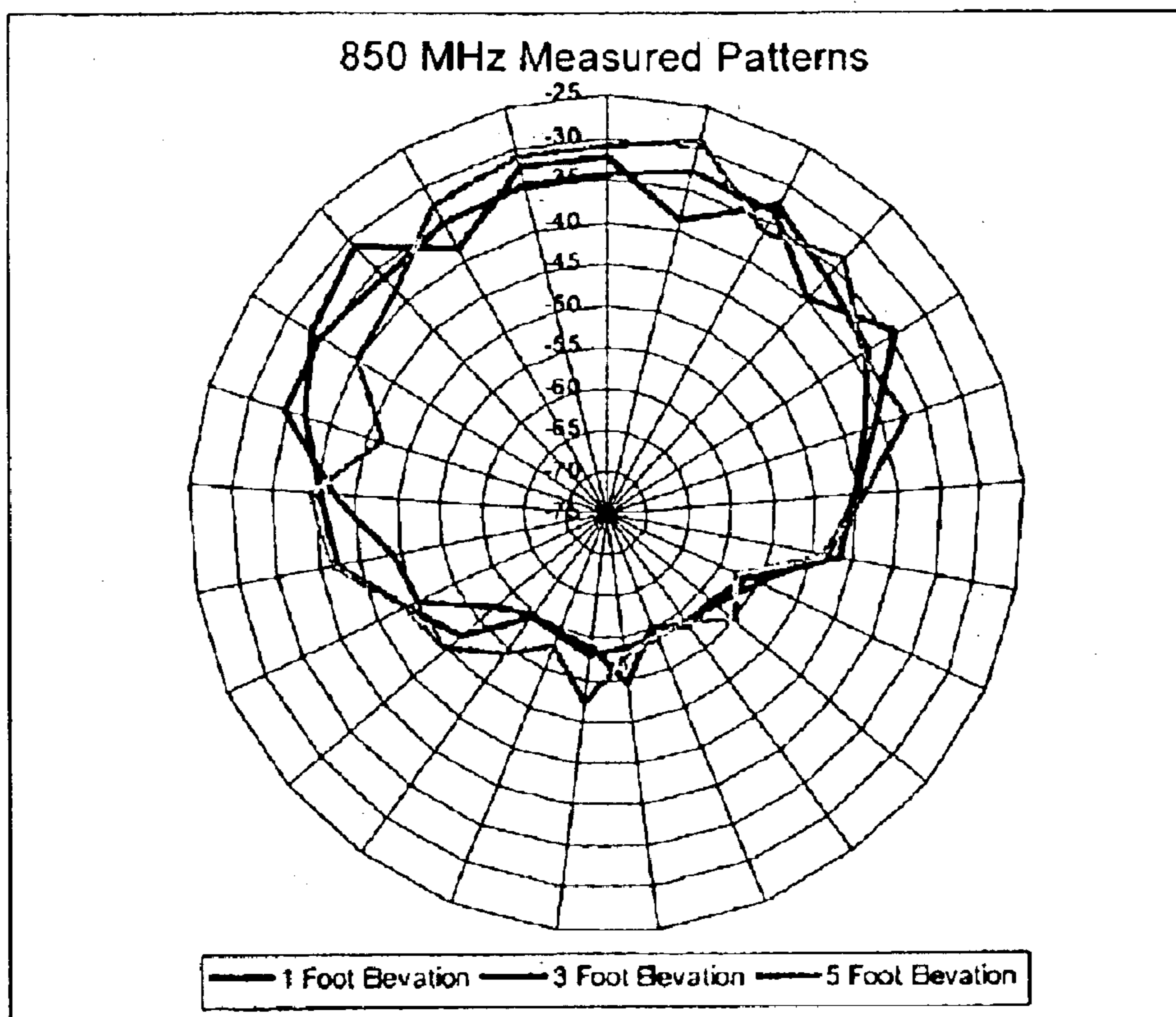
FIG 14 Patterns at 850 MHz
