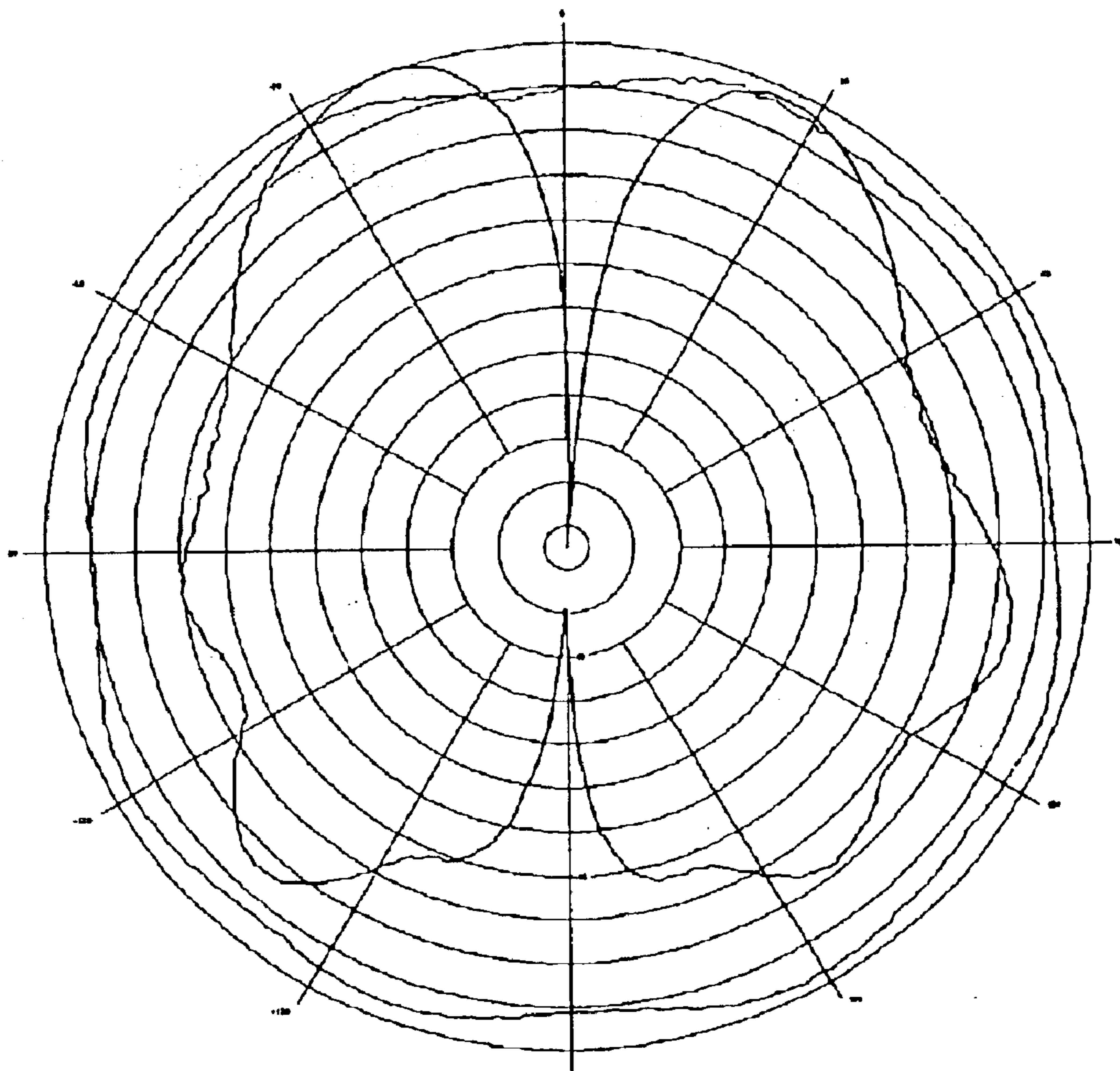
FIG 11 Azimuth and Elevation Pattern 1900 MHz
