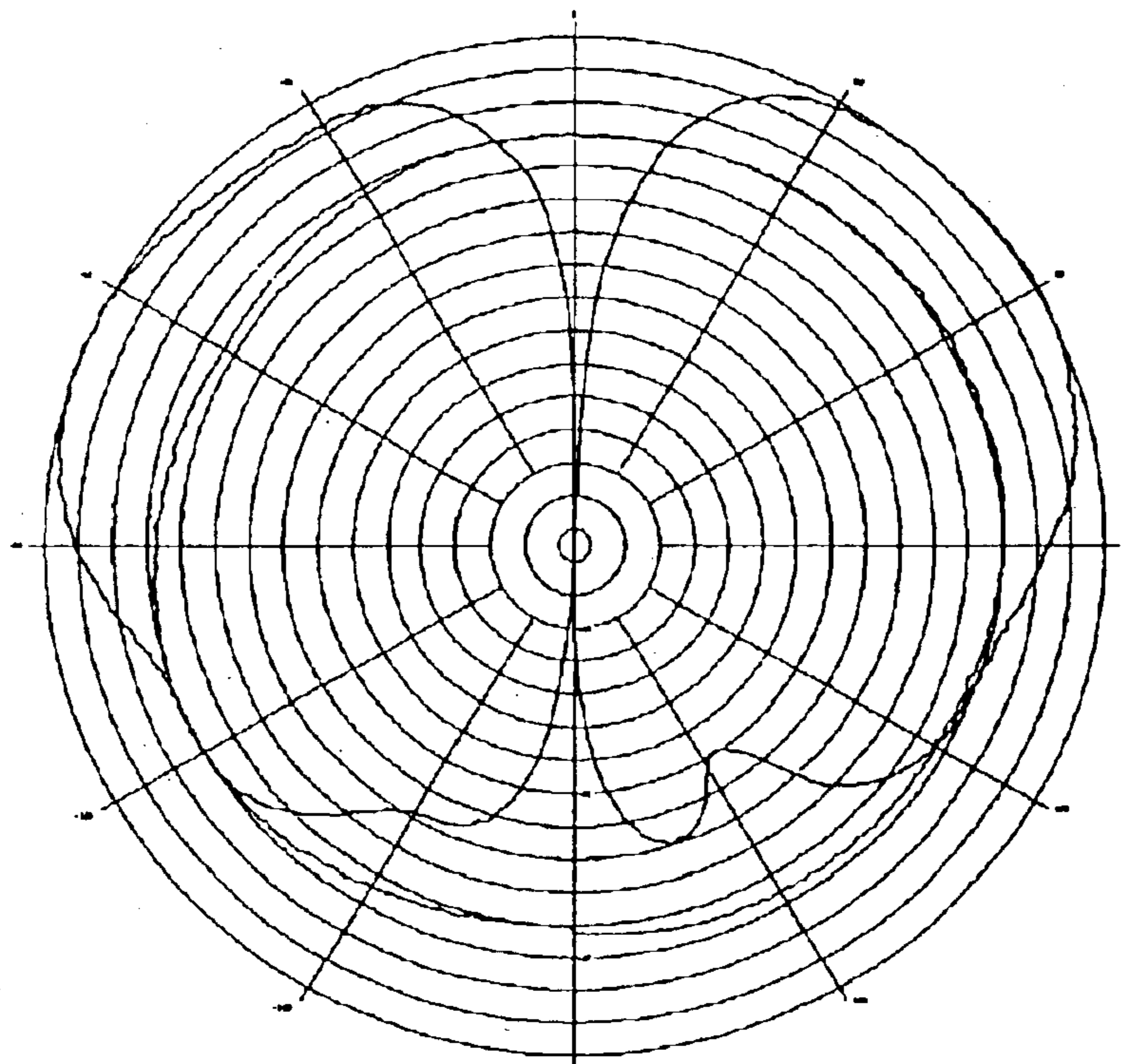
FIG 9 Azimuth and Elevation Pattern 1500 MHz
