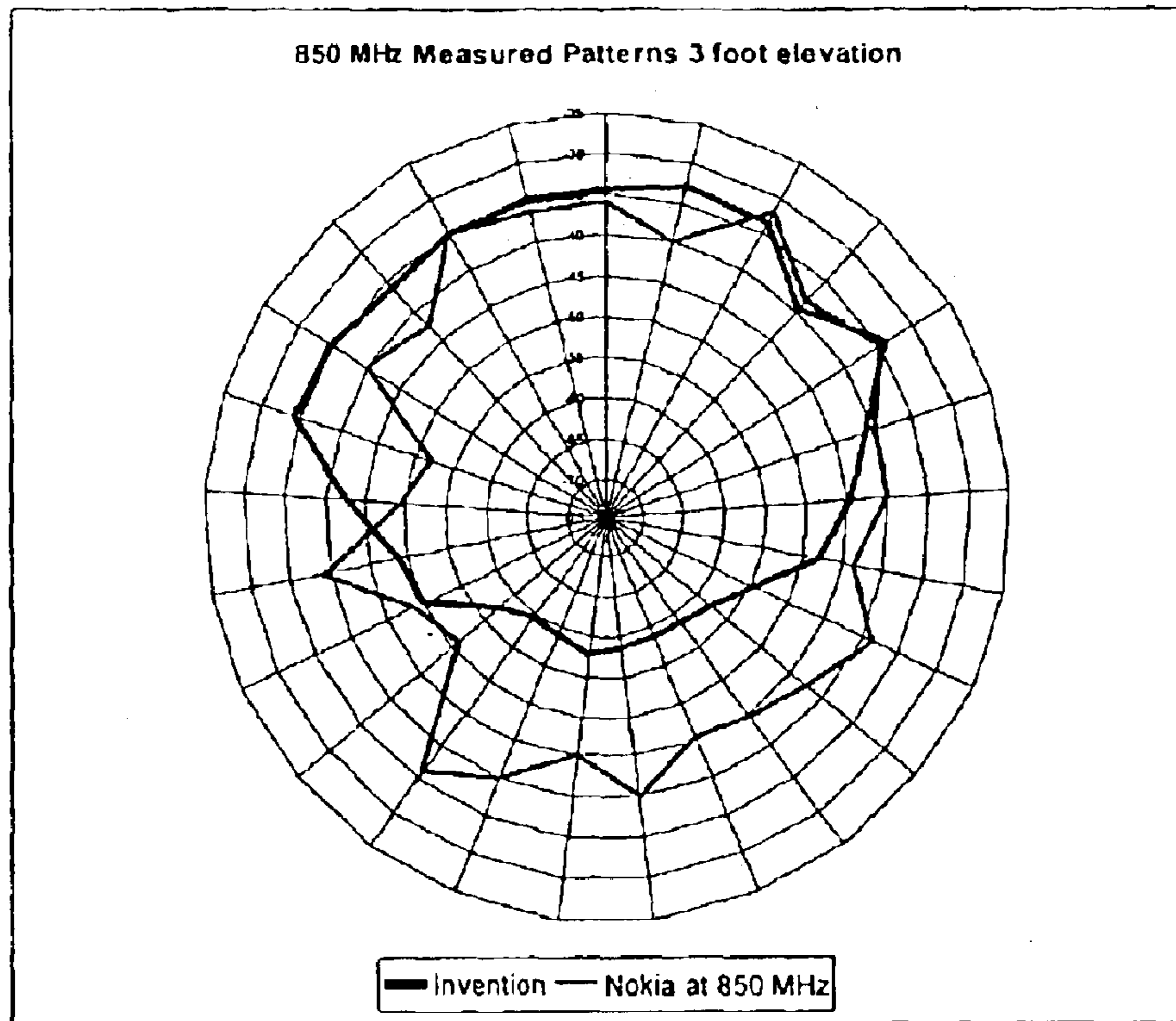
FIG 18 Data Comparison at 850 MHz
