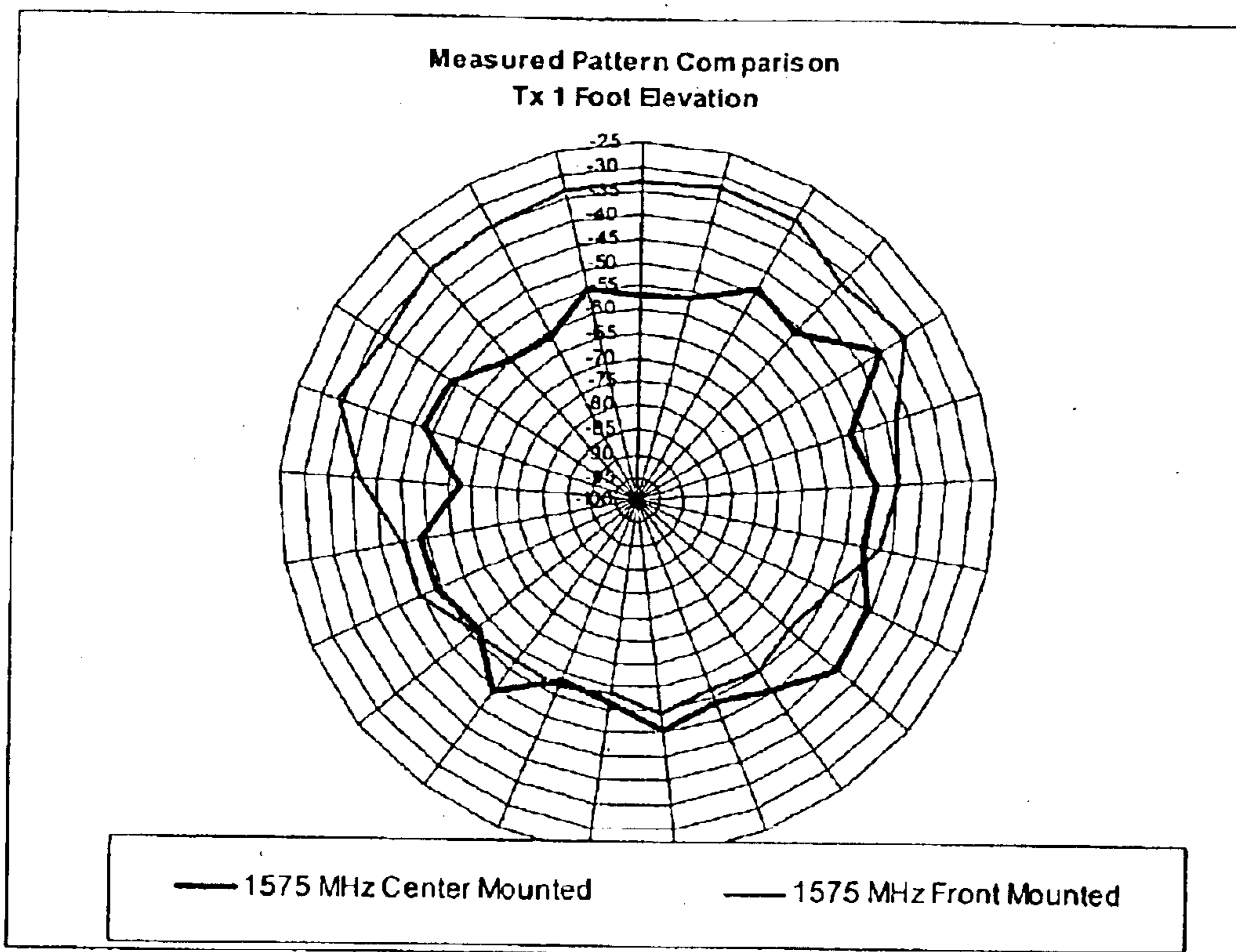
FIG 24 Comparison of Antenna Location at 1575 MHz
