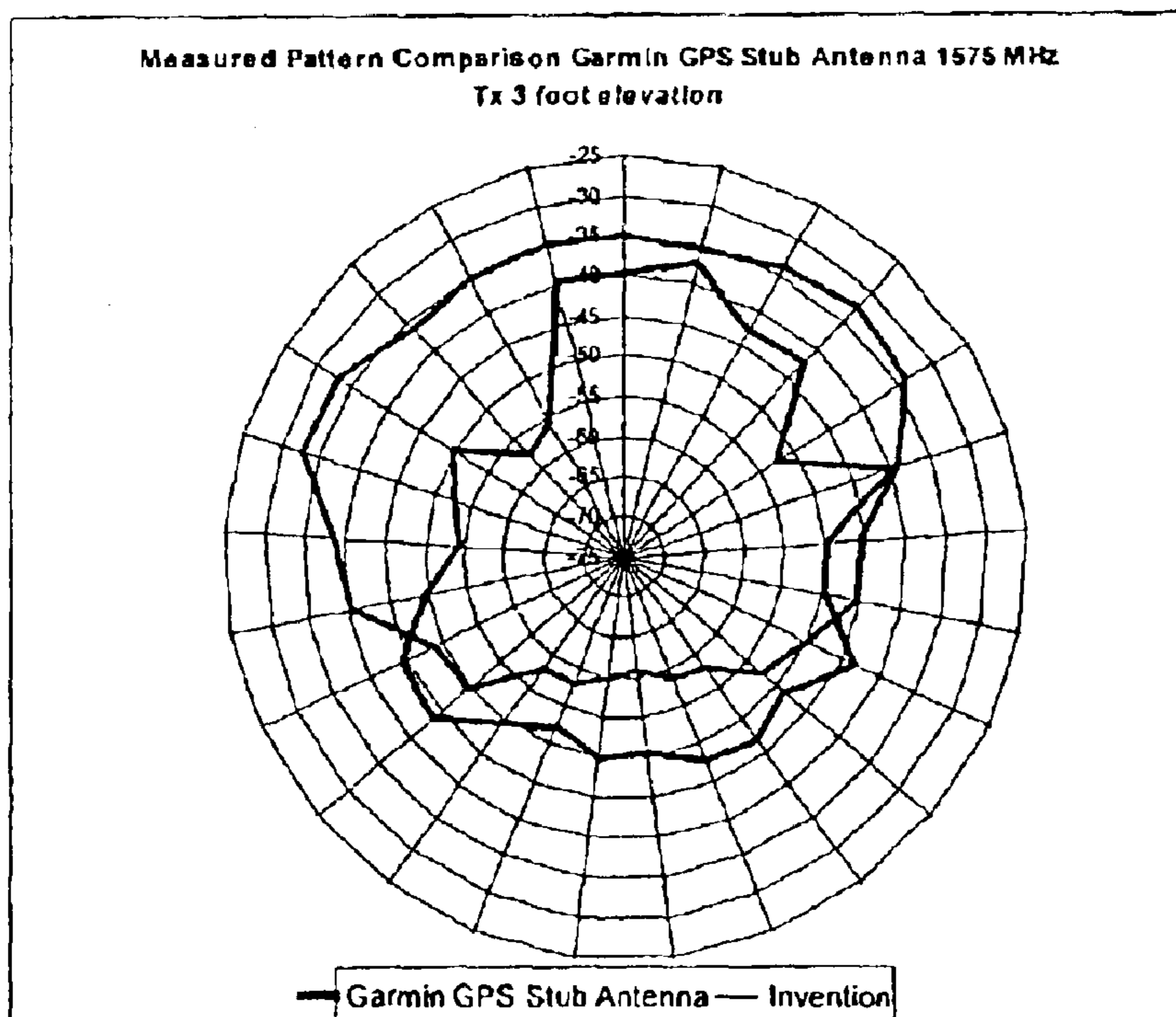
FIG 19 Data Comparison at 1575 MHz
