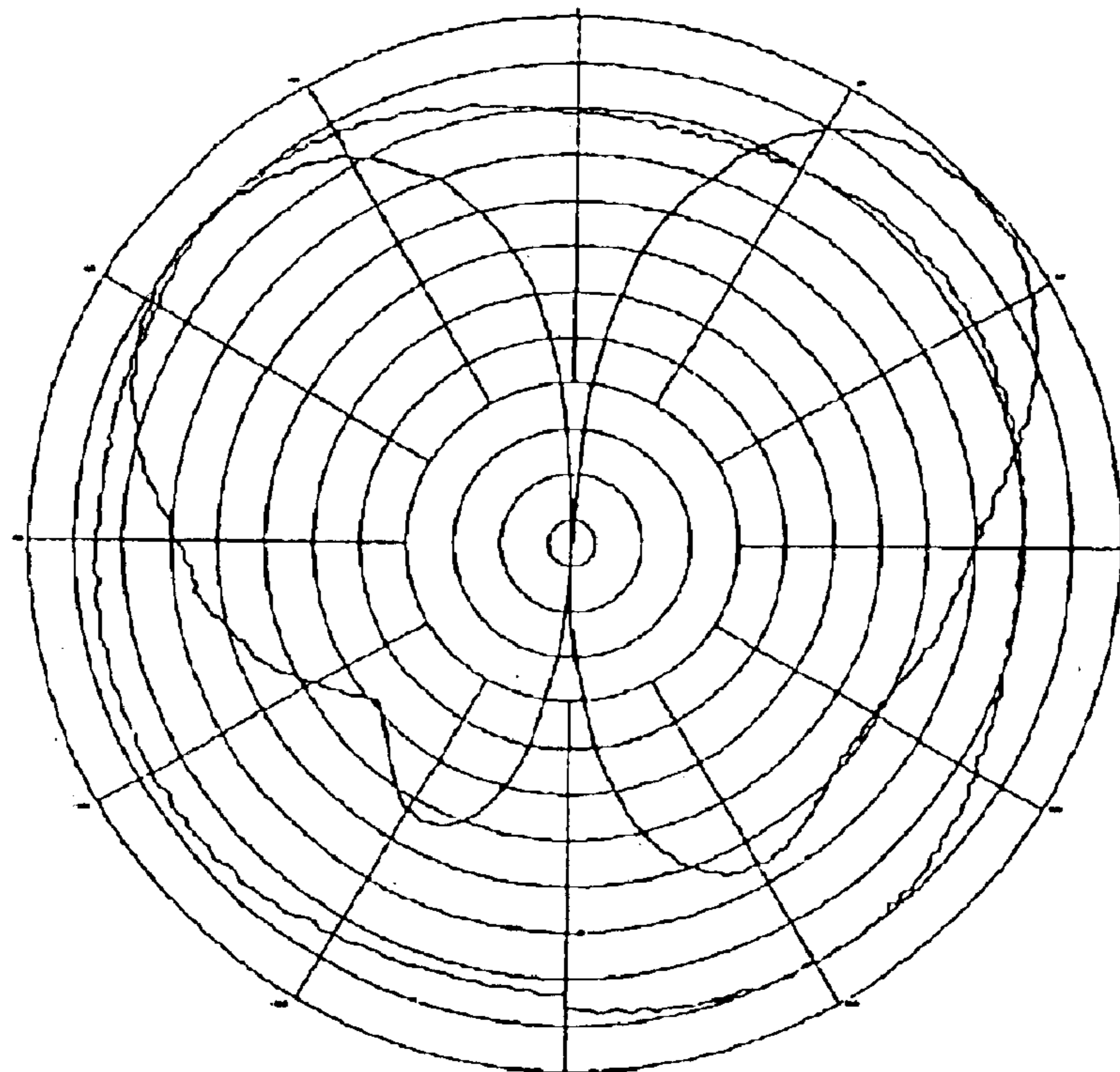
FIG 8 Azimuth and Elevation Pattern 900 MHz
