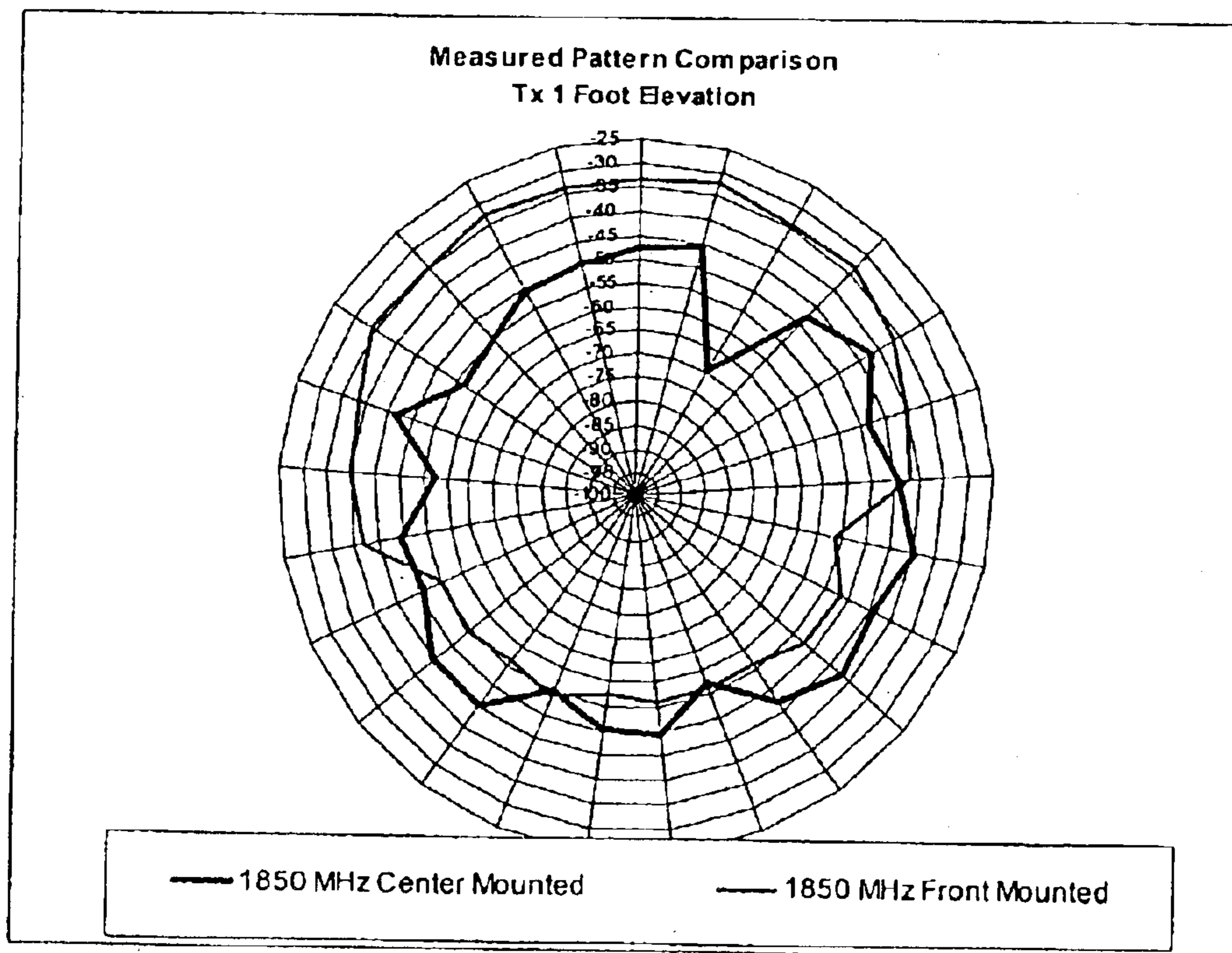
FIG 25 Comparison of Antenna Location at 1850 MHz
