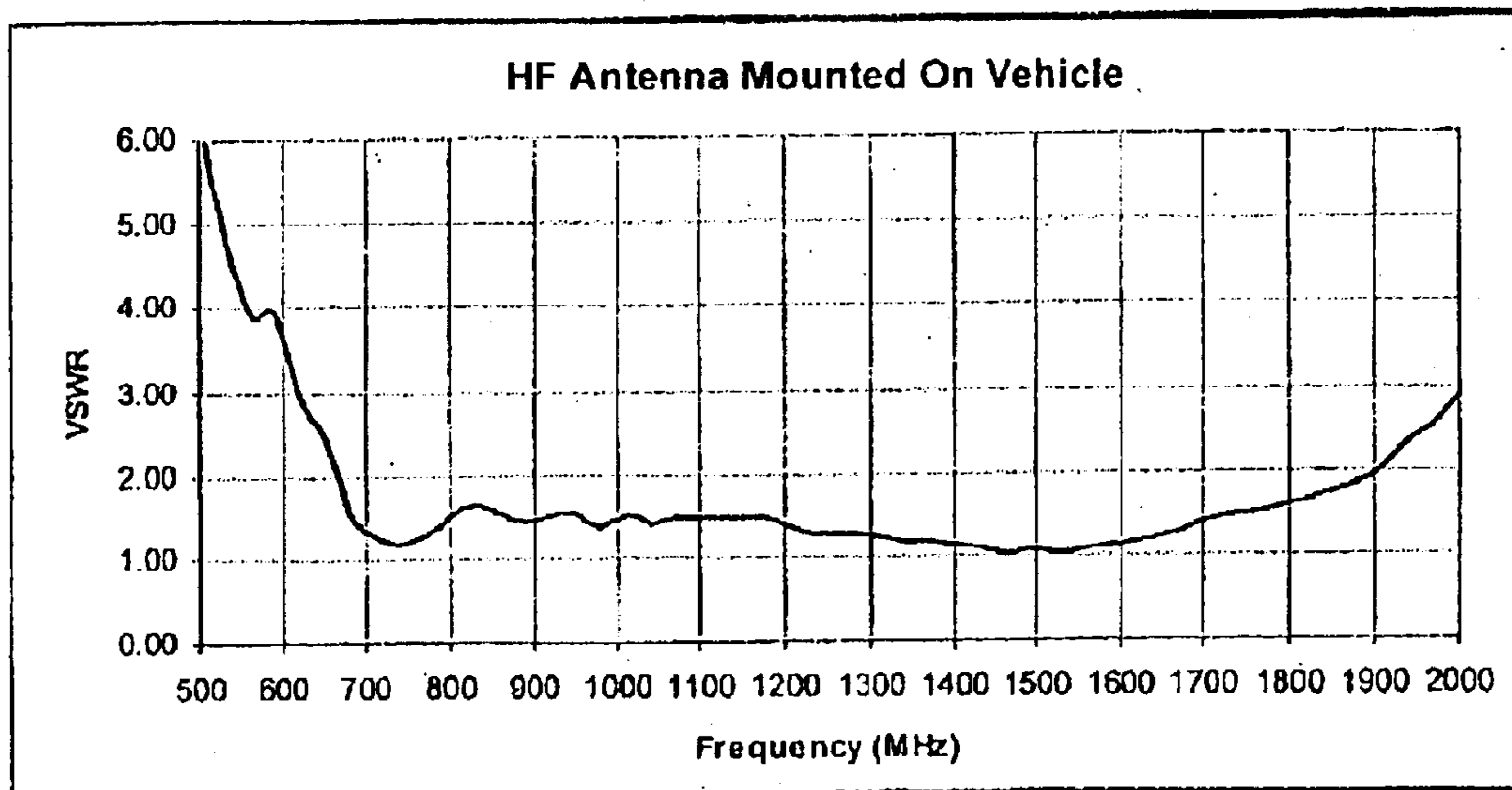
FIG13 Measured VSWR
