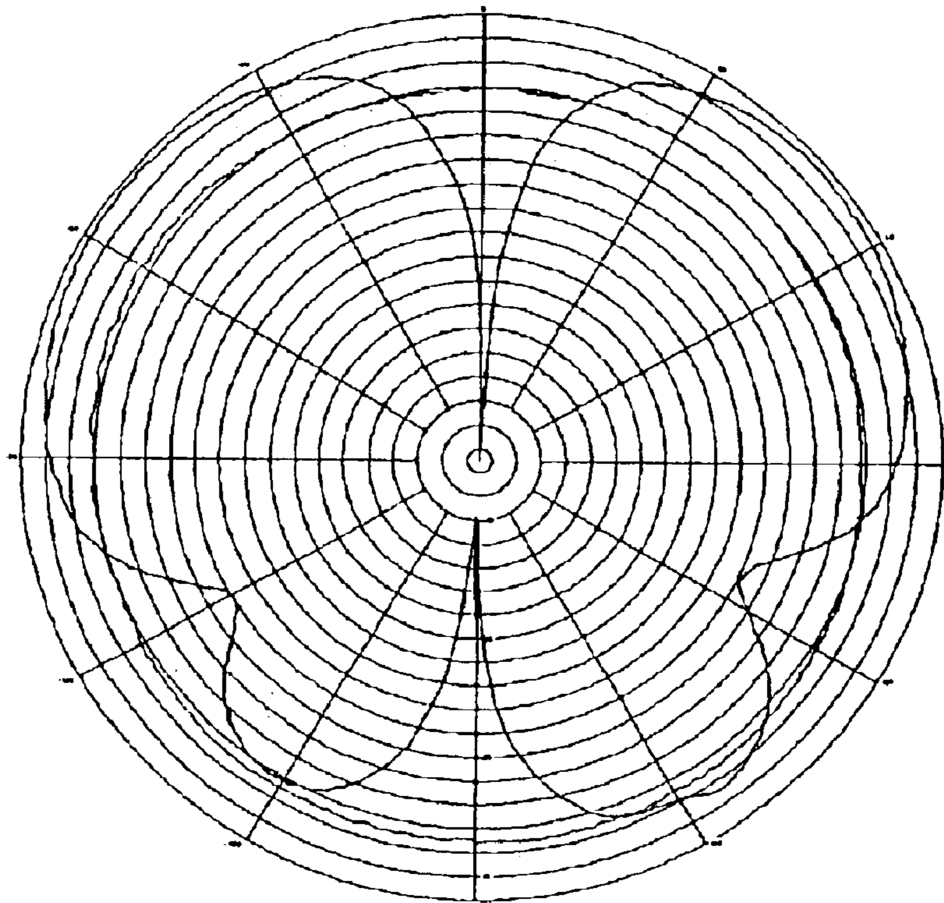
FIG 7 Azimuth and Elevation Pattern 800 MHz
