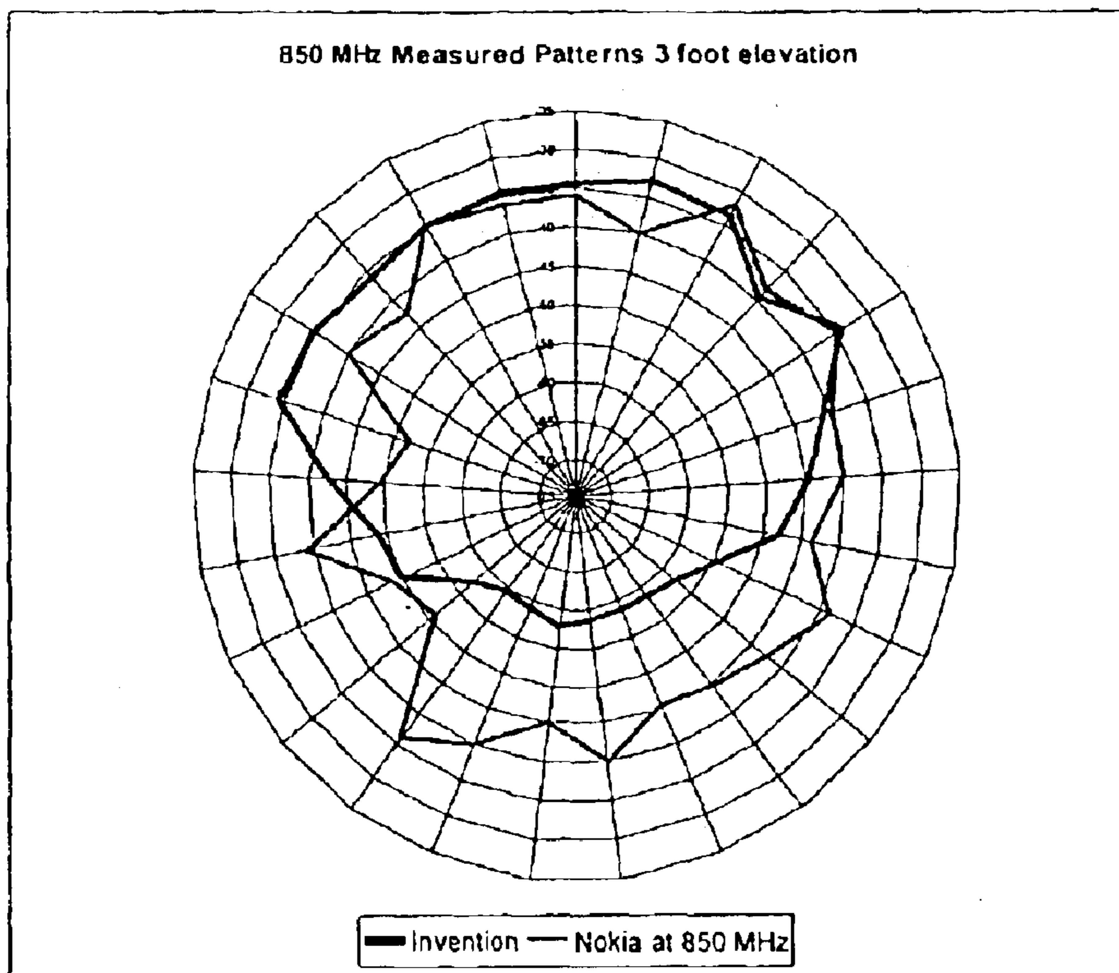
FIG 18 Data Comparison at 850 MHz
