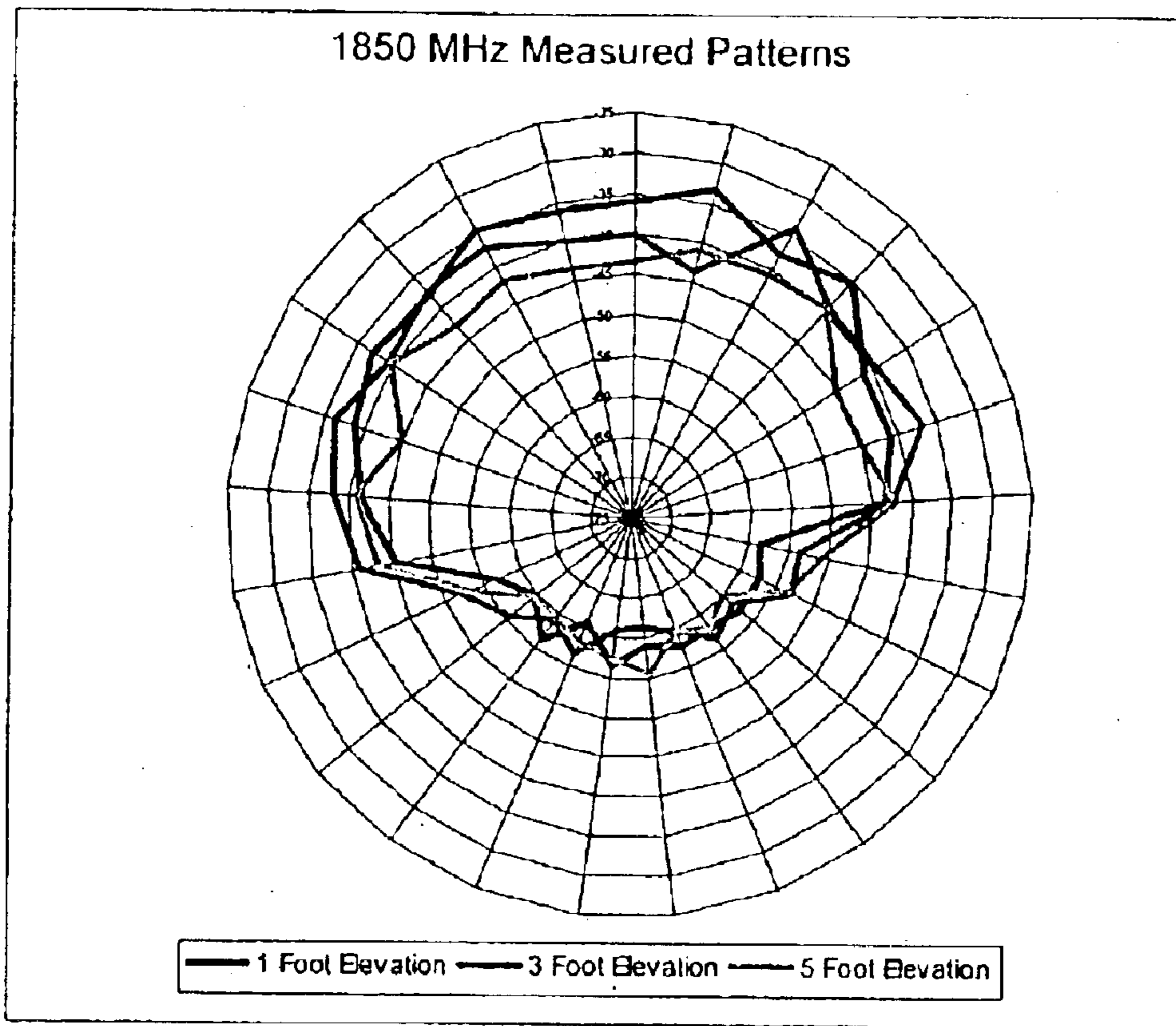
FIG 16 Patterns at 1850 MHz
