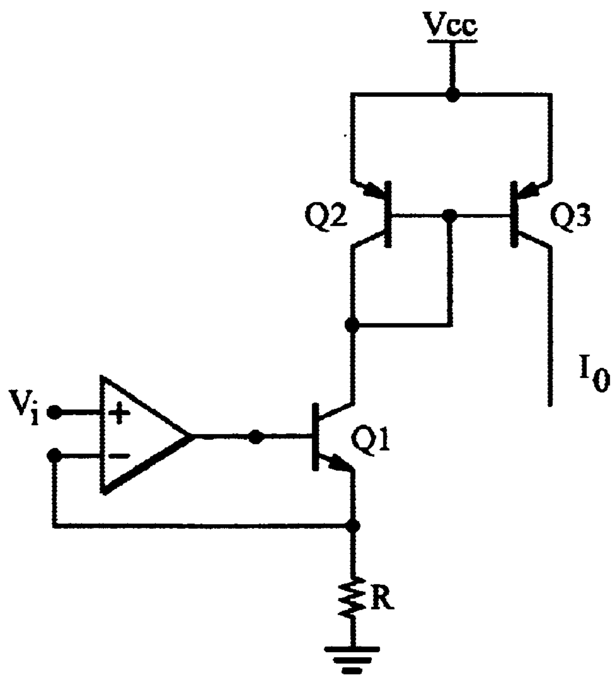
Figure 1A Prior Art - Voltage to Current Converter
