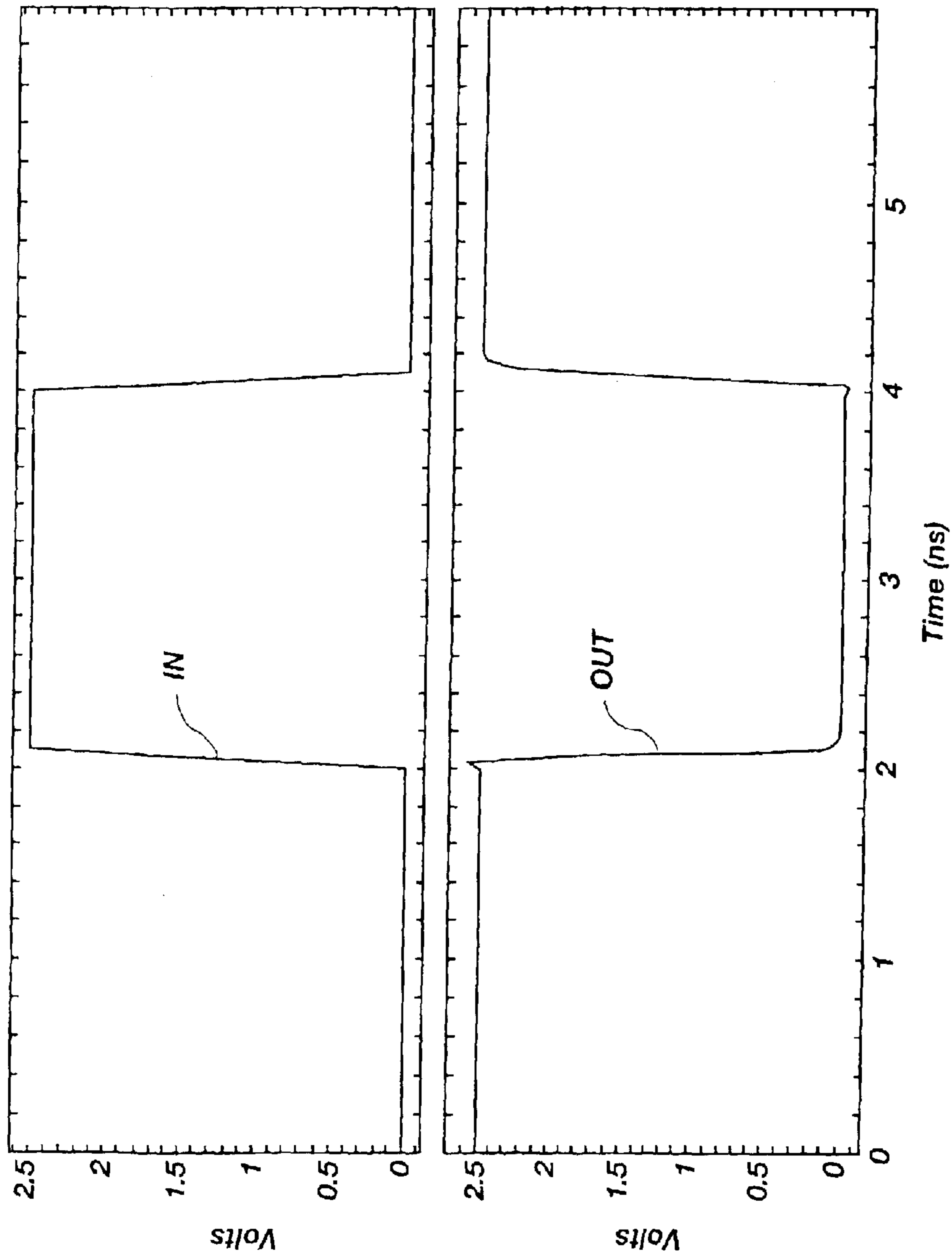
Fig. 2 (PRIOR ART)
