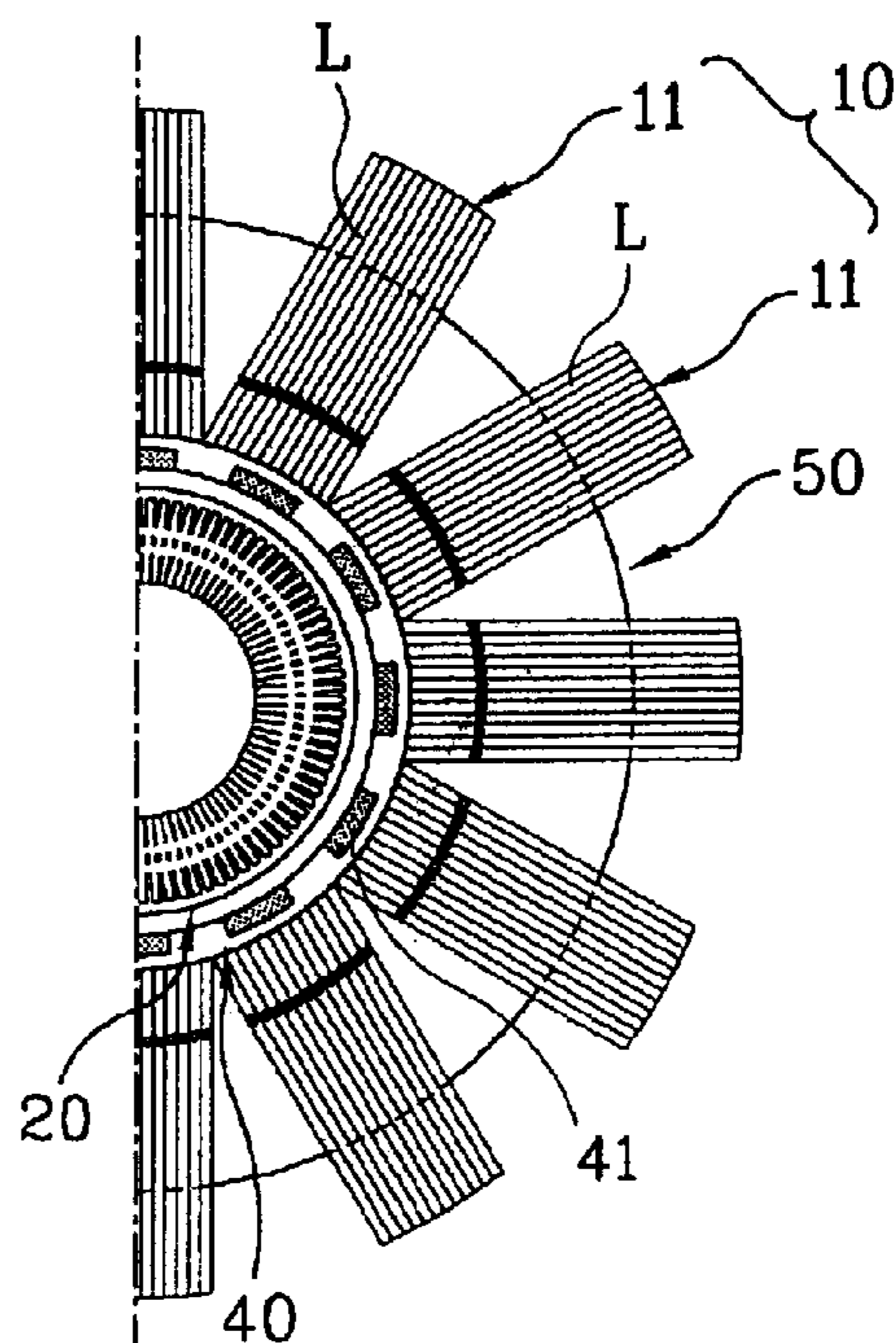
FIG. 2 CONVENTIONAL ART
