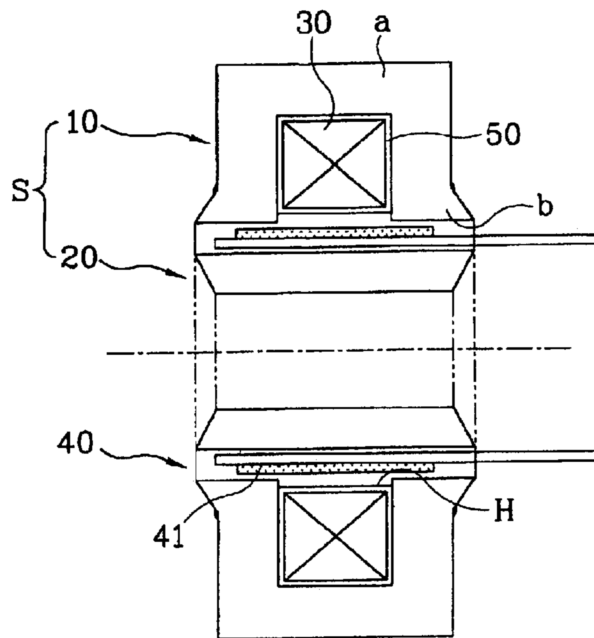
FIG. 1 CONVENTIONAL ART
