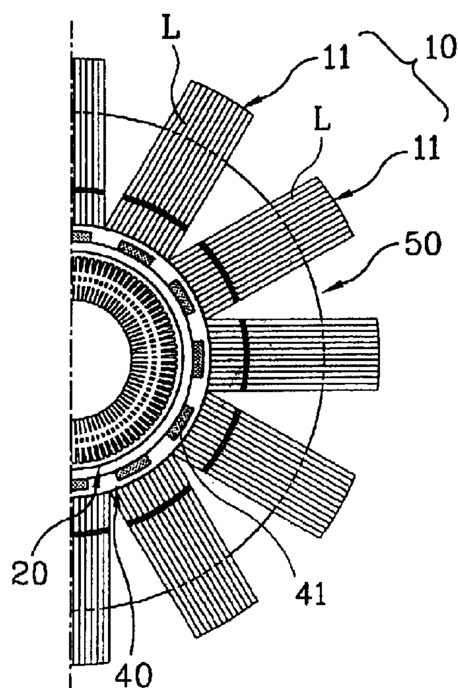
FIG. 2 CONVENTIONAL ART
