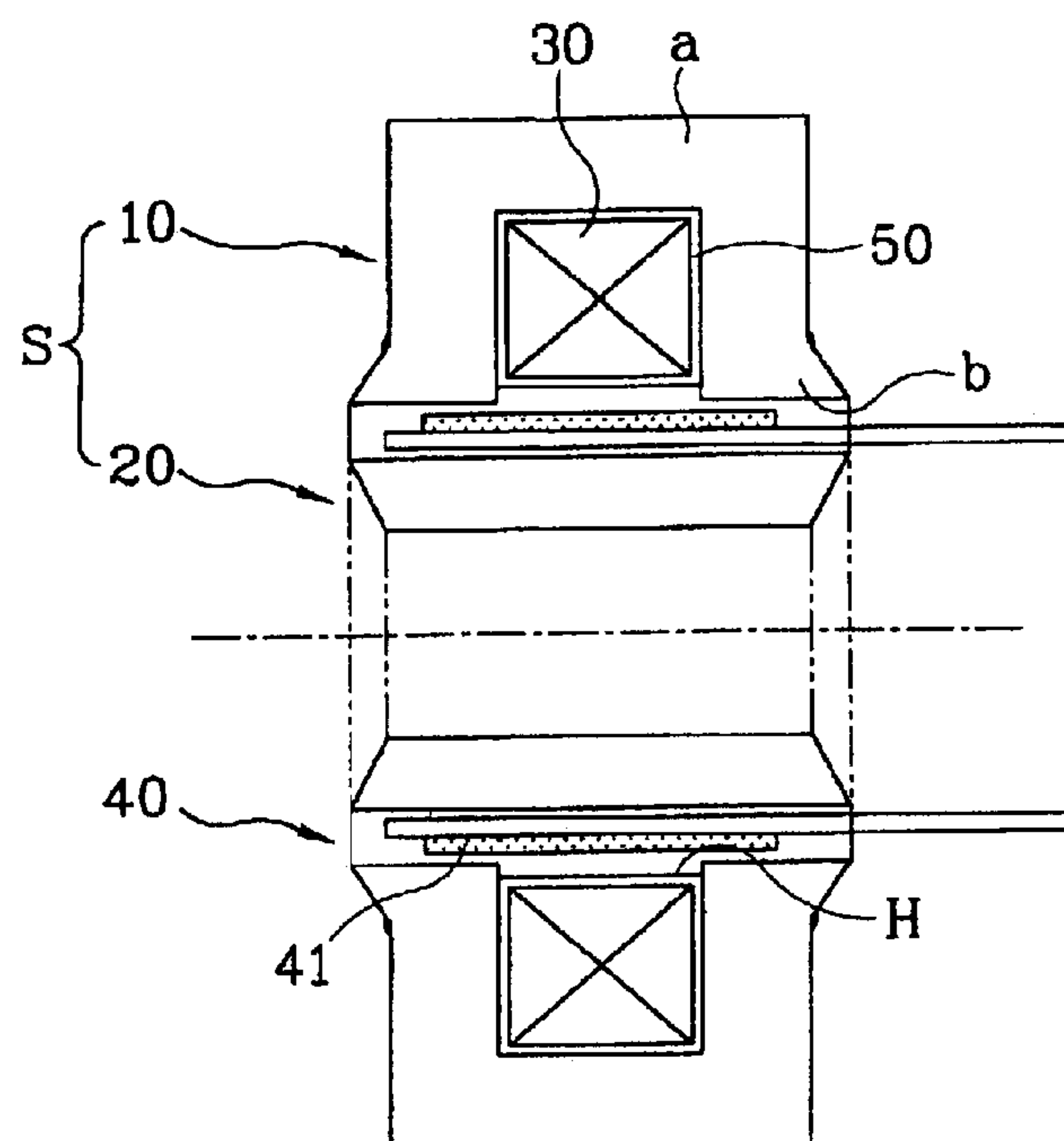
FIG. 1 CONVENTIONAL ART
