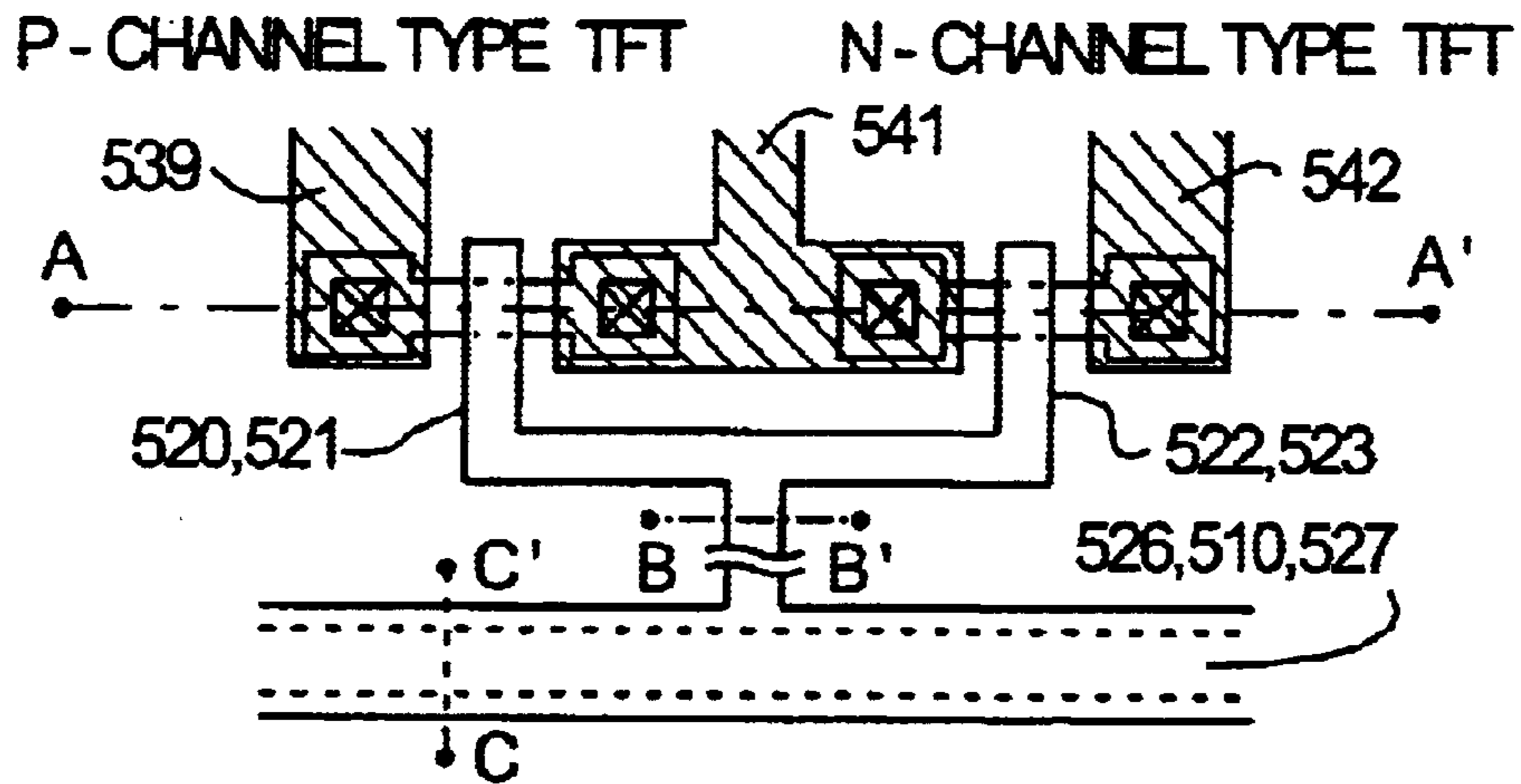
TOP VIEW OF CMOS CIRCUIT
