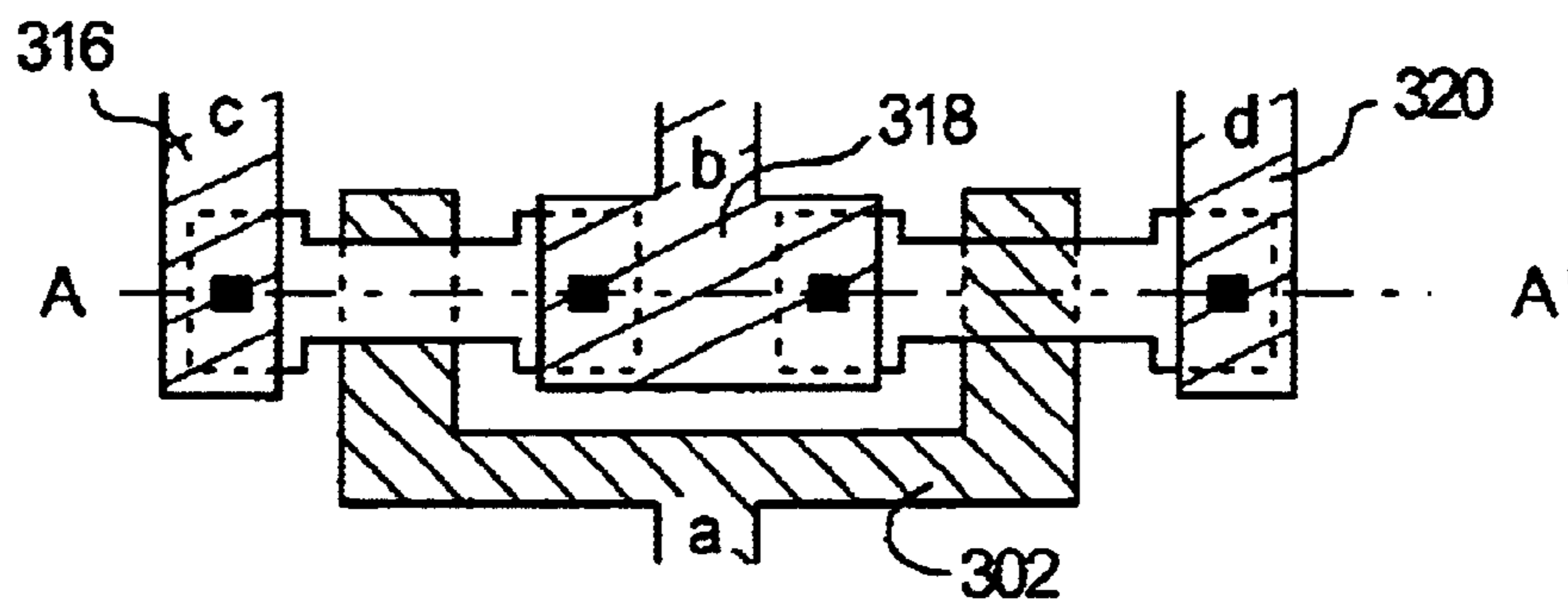
TOP VIEW OF CMOS CIRCUIT
