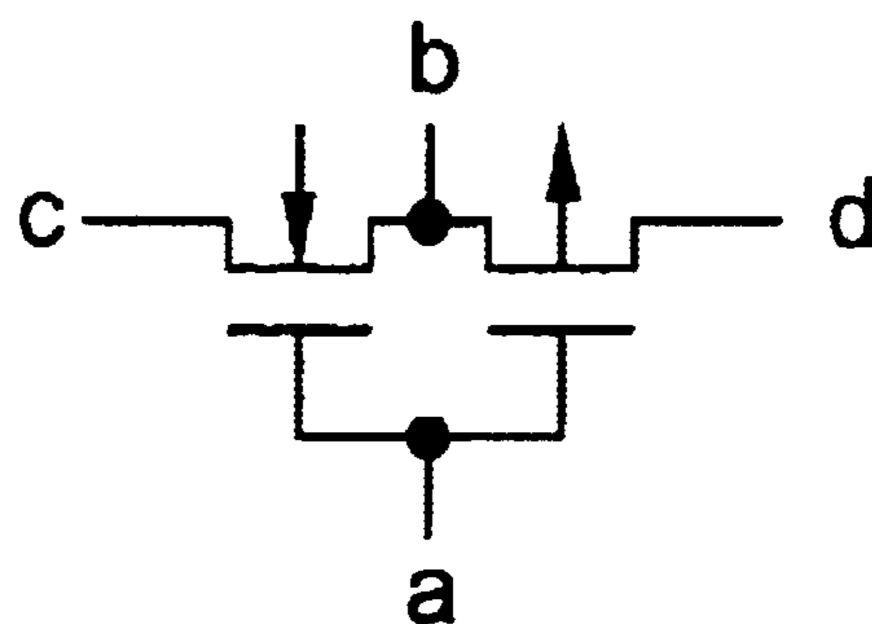
CIRCUIT DIAGRAM OF CMOS
