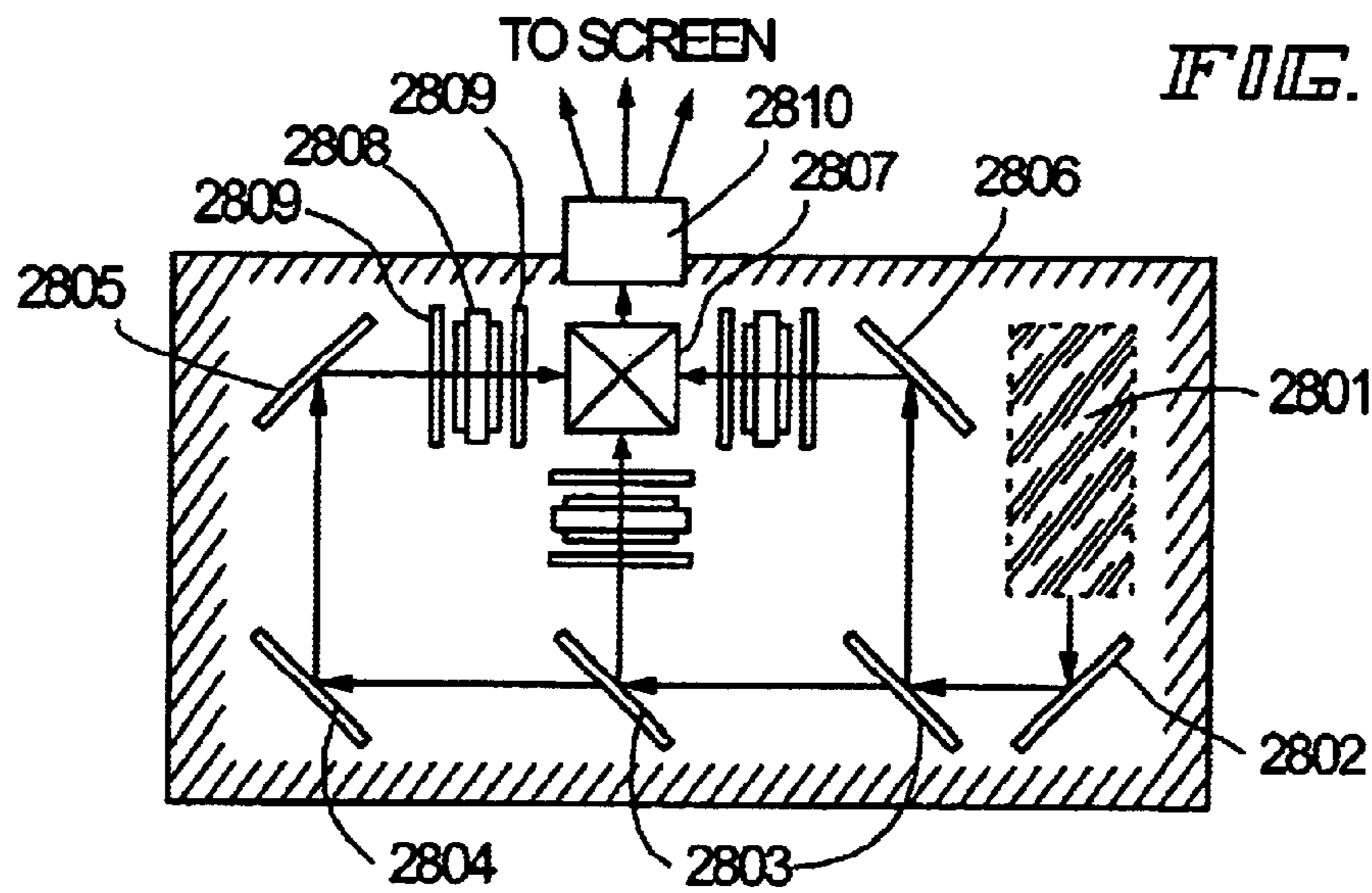
PROJECTION DEVICE (THREE PLATE TYPE)
