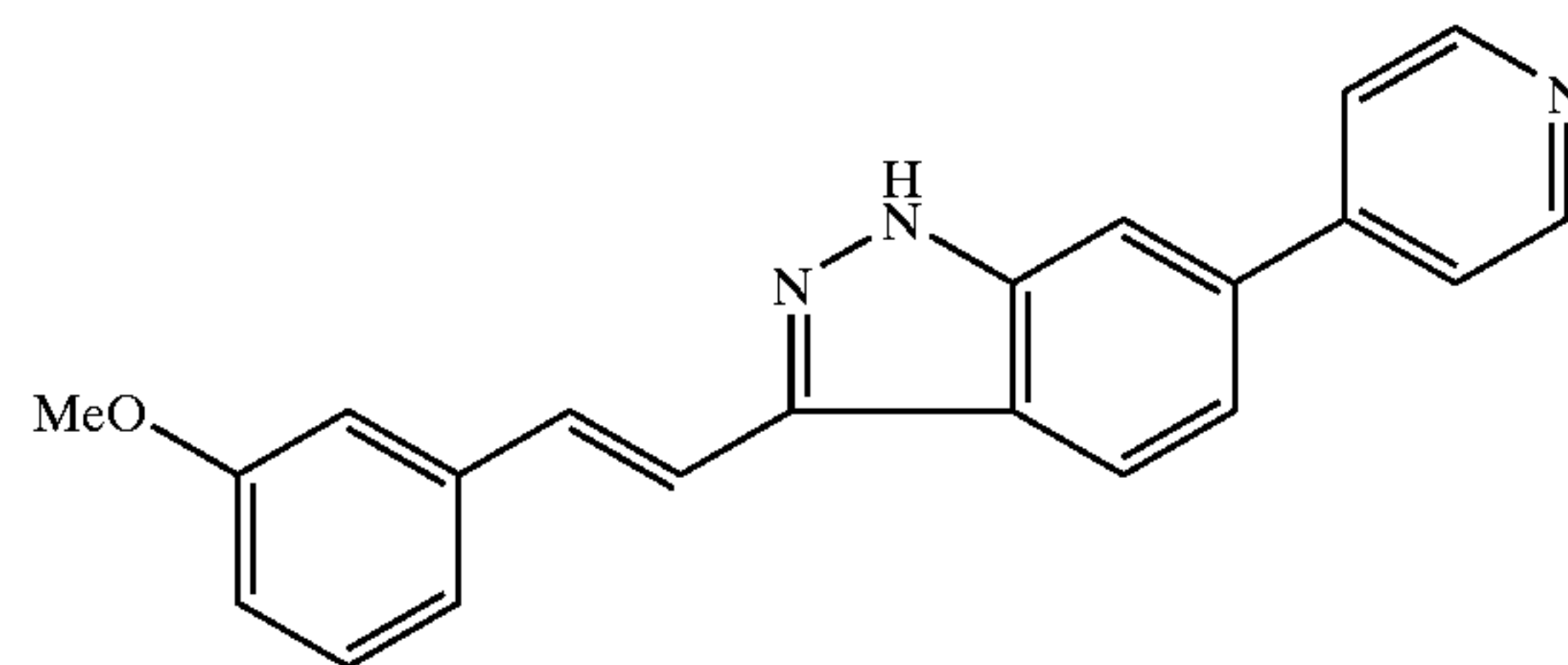
6-pyrid-4-yl-3-E-[2-(3-methoxyphenyl)ethenyl]-1H-indazole
