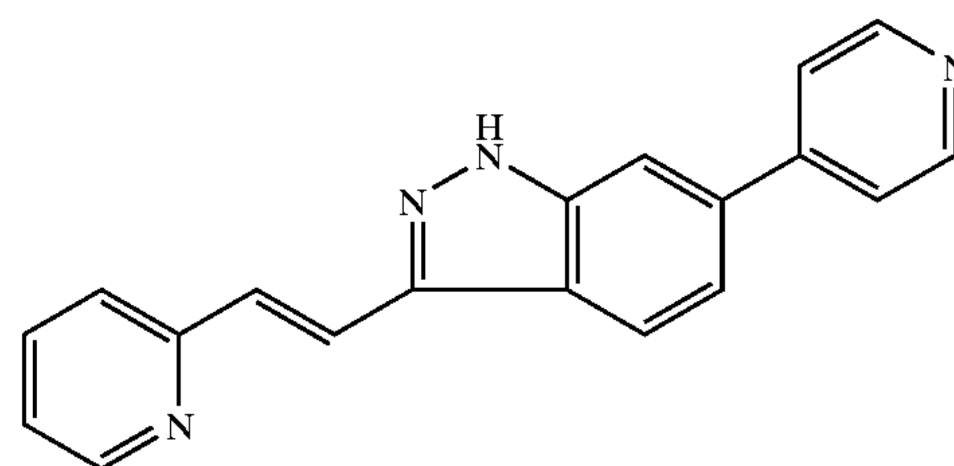
6-pyrid-4-yl-3-E-[2-(pyrid-2-yl)ethenyl]-1H-indazole
