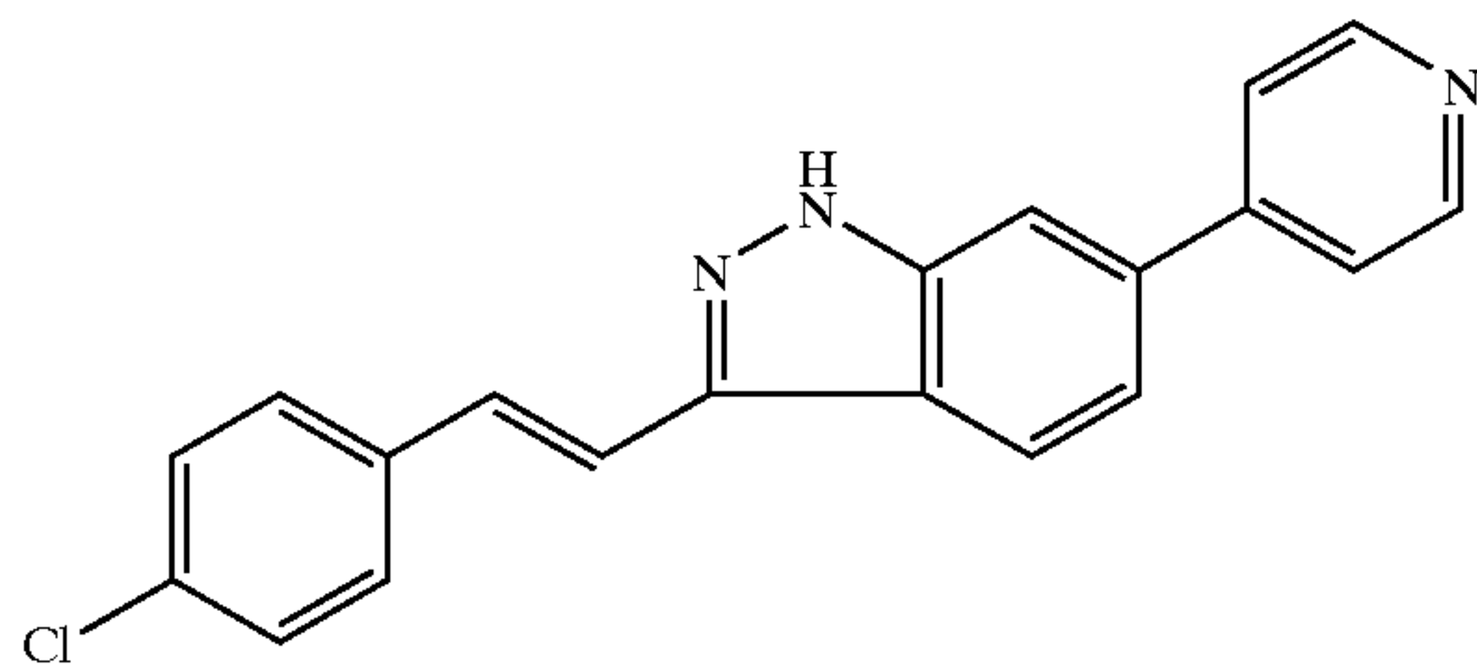
6-pyrid-4-yl-3-E-[2-(4-chlorophenyl)ethenyl]-1H-indazole
