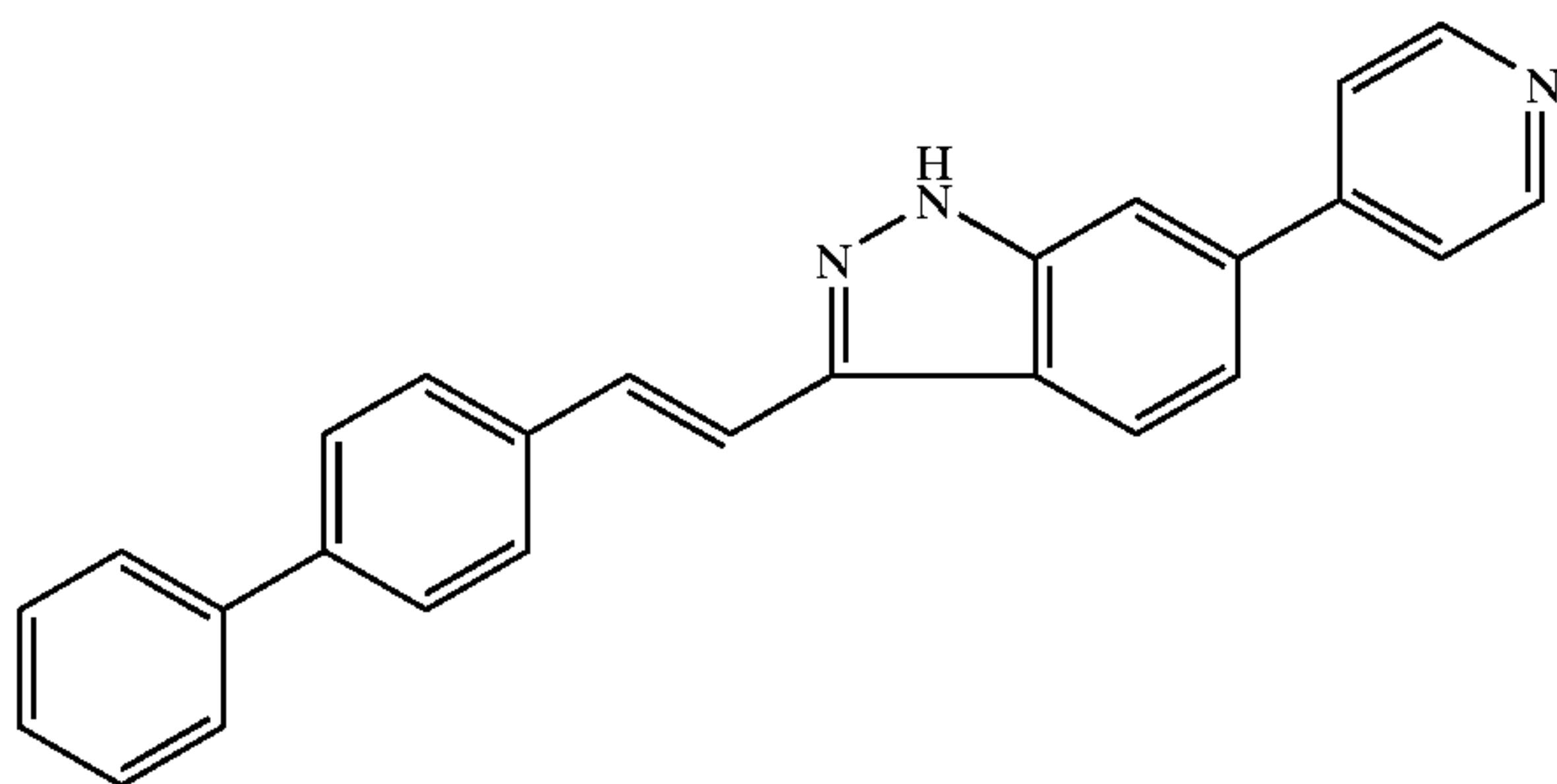
6-pyridyl-3-E-[2-(biphenyl-4-yl)ethenyl]-1H-indazole
