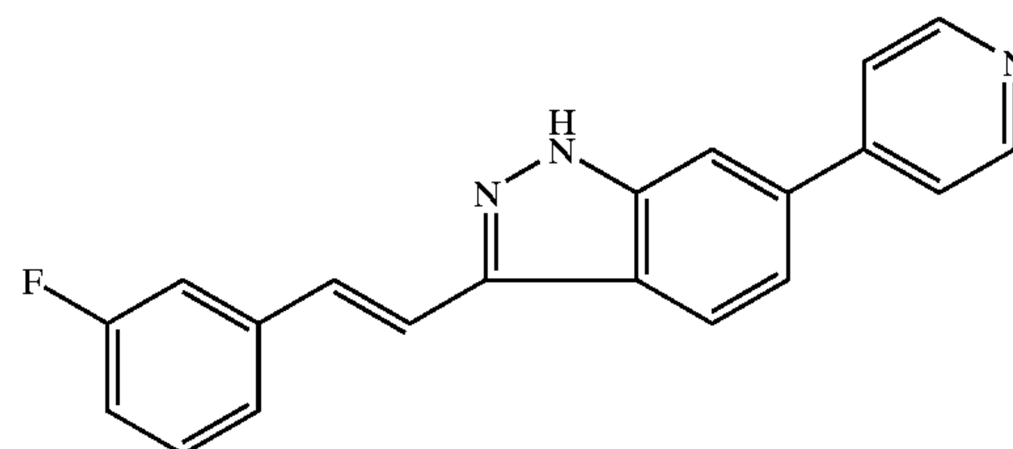
6-pyrid-4-yl-3-E-[2-(3-fluorophenyl)ethenyl]-1H-indazole
