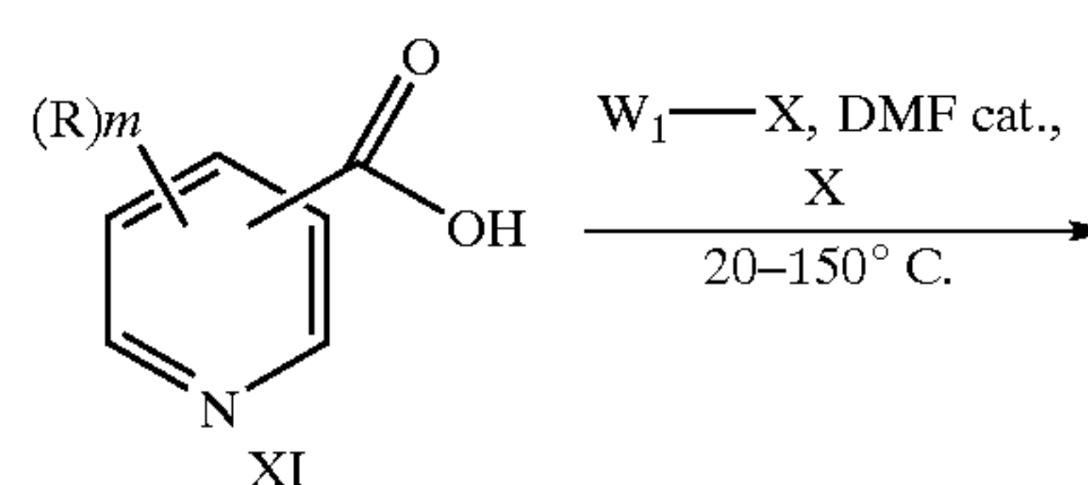
Reaction Scheme 3
