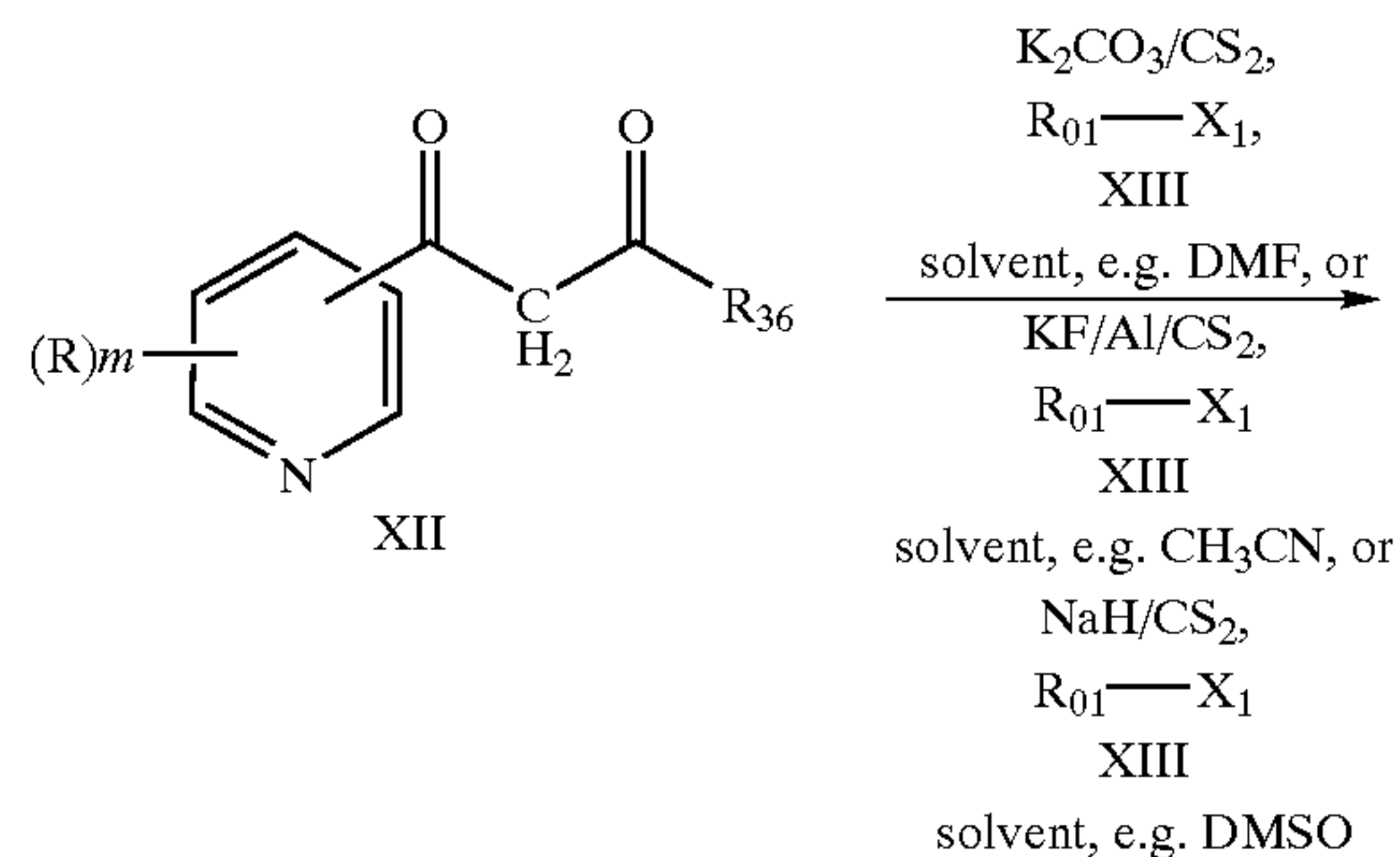
Reaction Scheme 2
