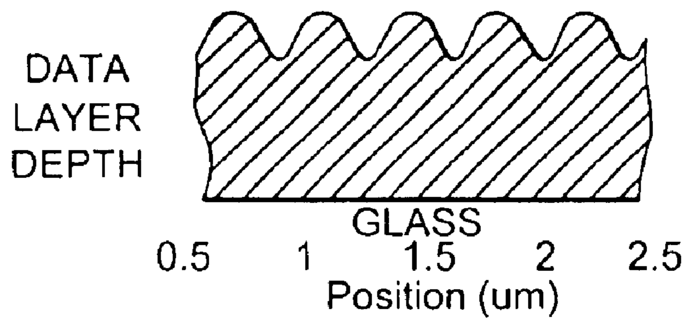
FIG. 1 PRIOR ART
