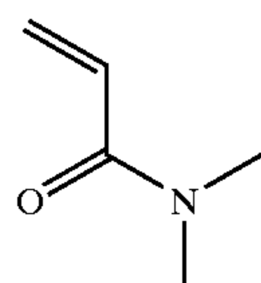
N,N-dimethylacrylamide (DMA)
