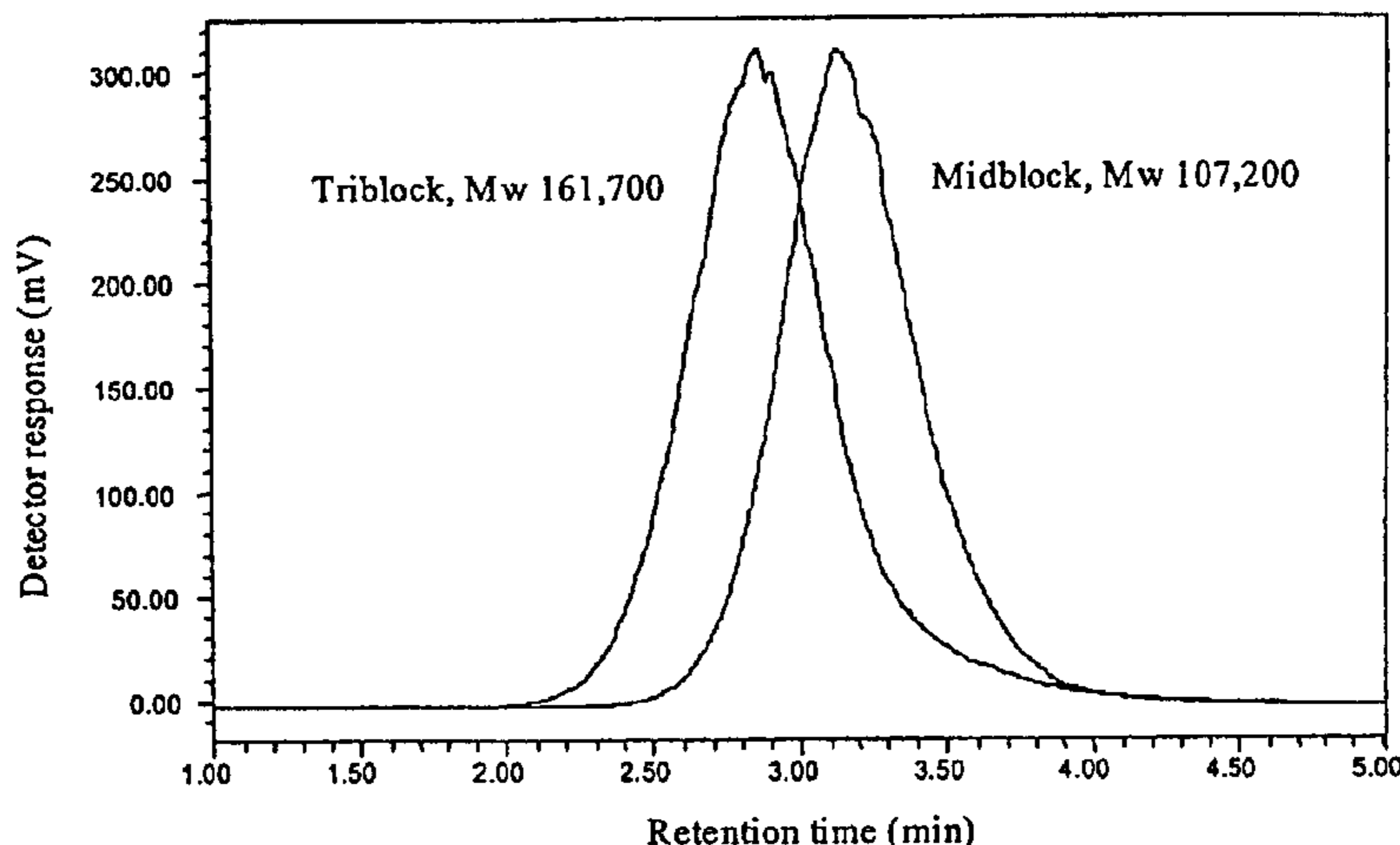
SEC traces of midblock and triblock polymers
