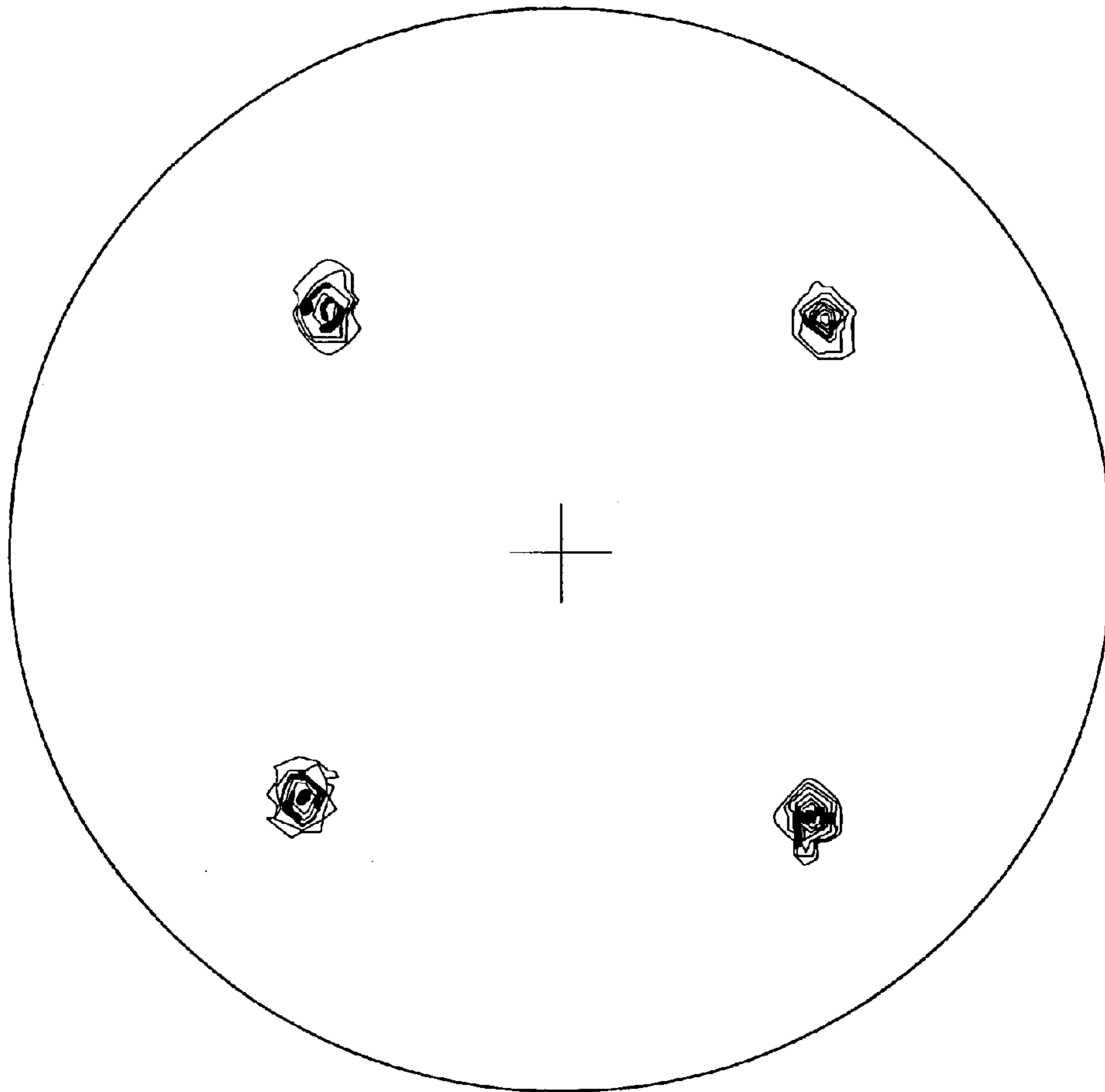
Ni-9at%W alloy Annealing Temperature = 1400°C
