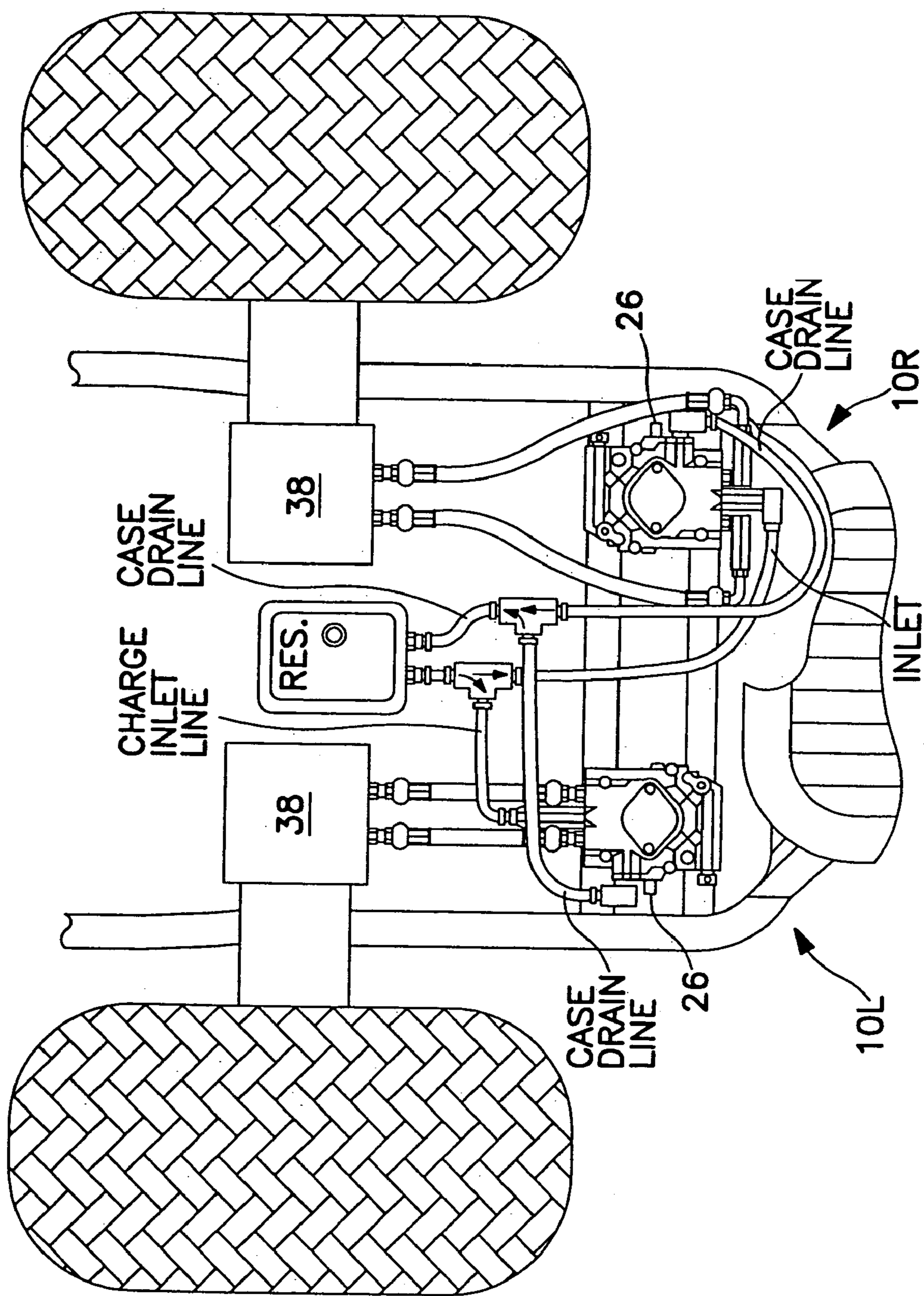
FIG. 2 PRIOR ART
