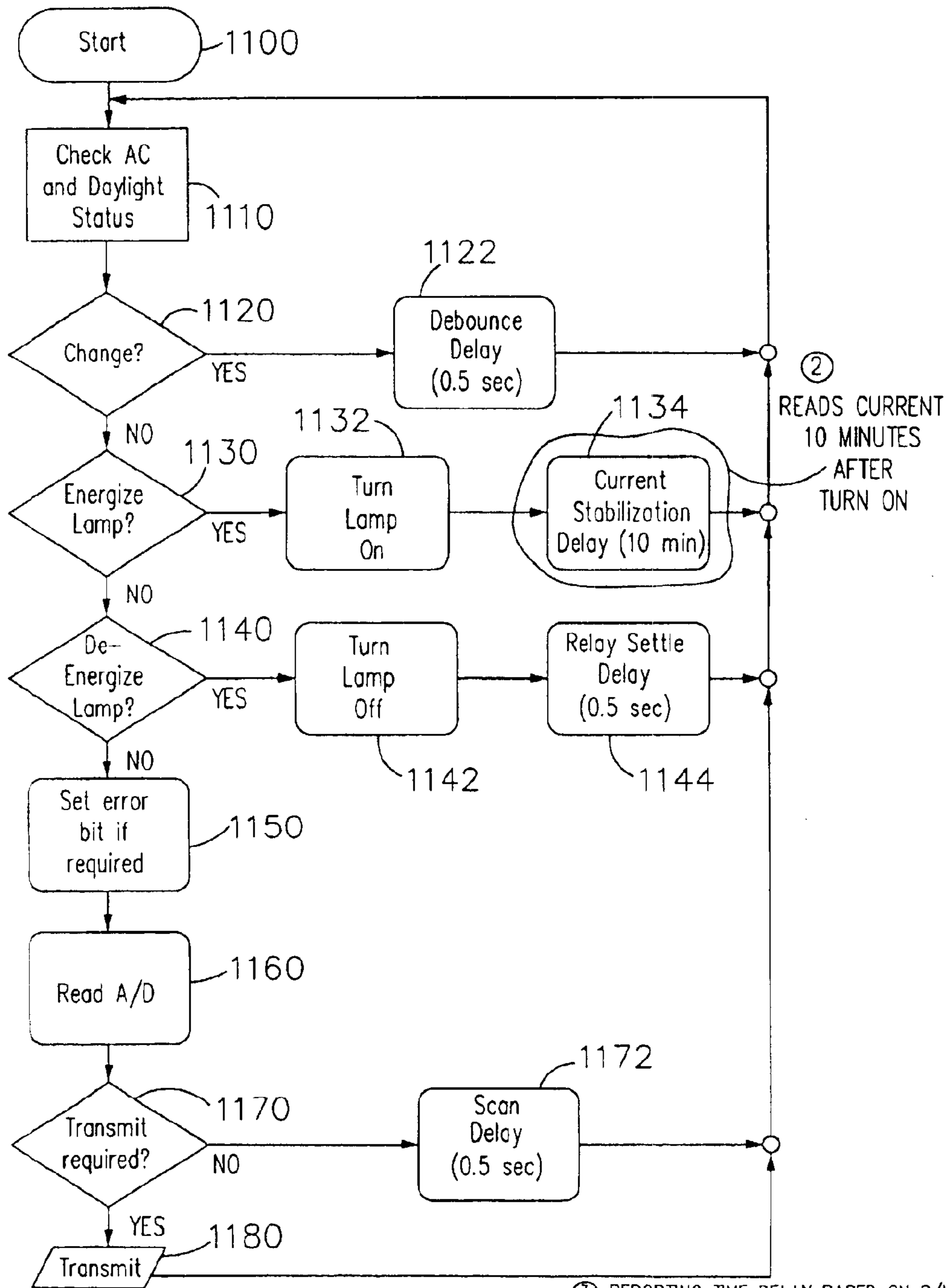
FIG. 11A (3) REPORTING TIME DELAY BASED ON S/N
