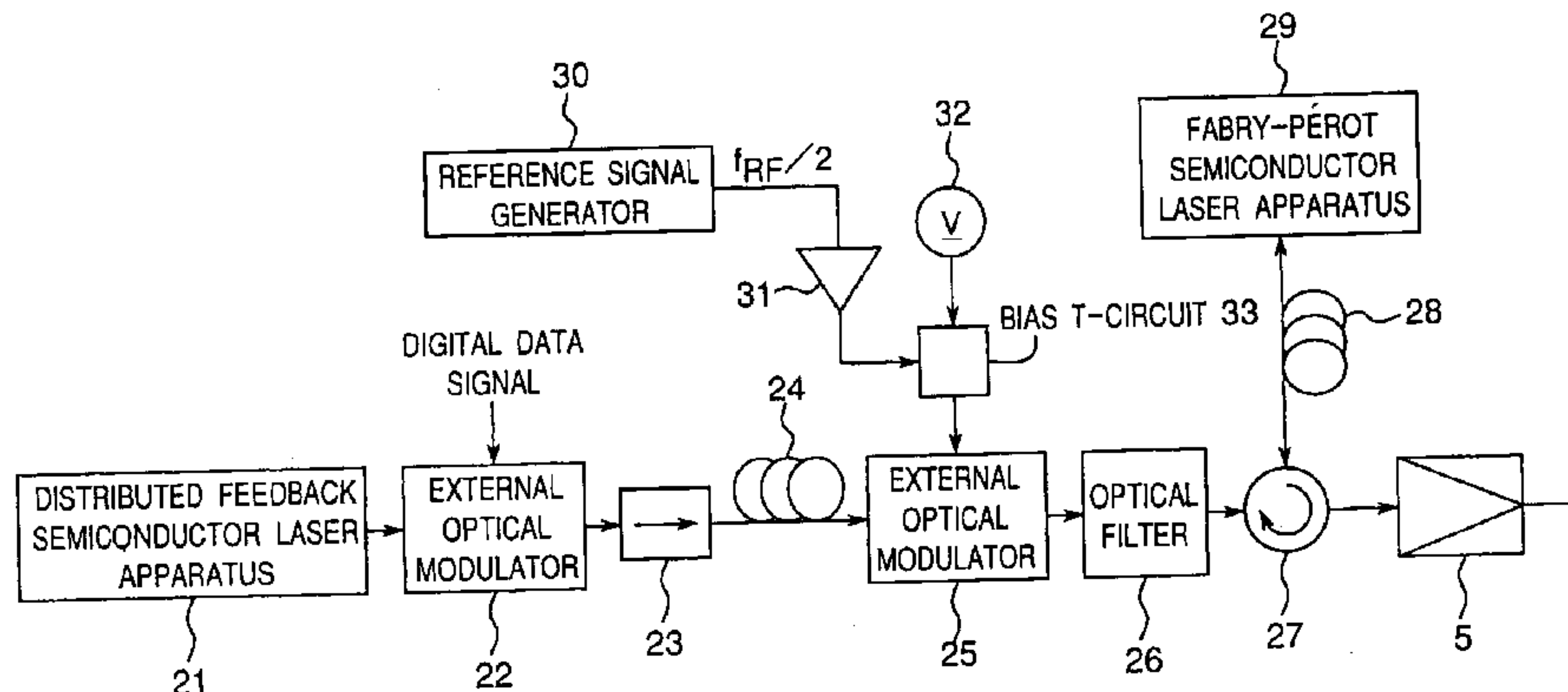
FIRST PREFERRED EMBODIMENT OPTICAL TRANSMITTER 101a
