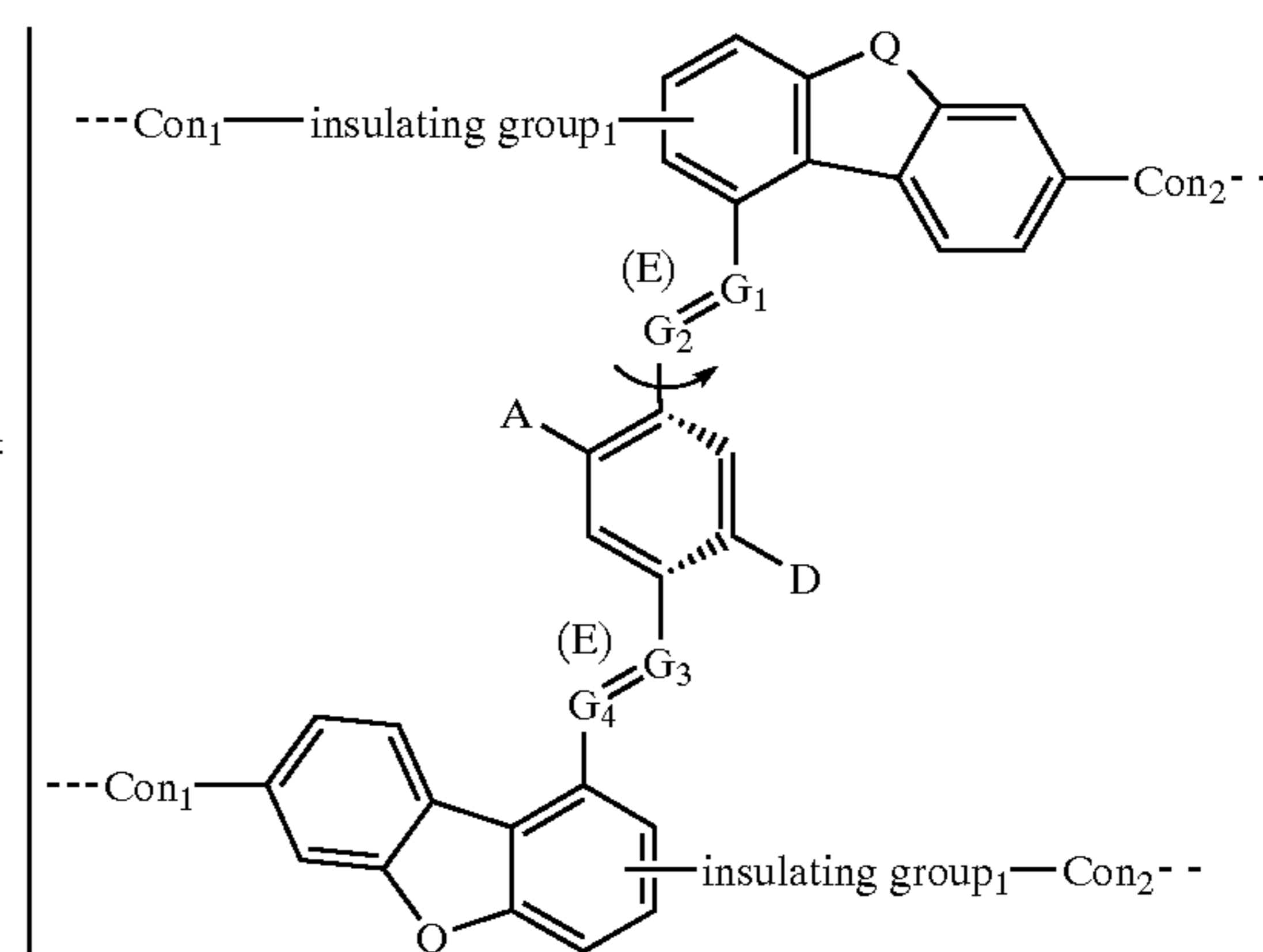
Transition State
