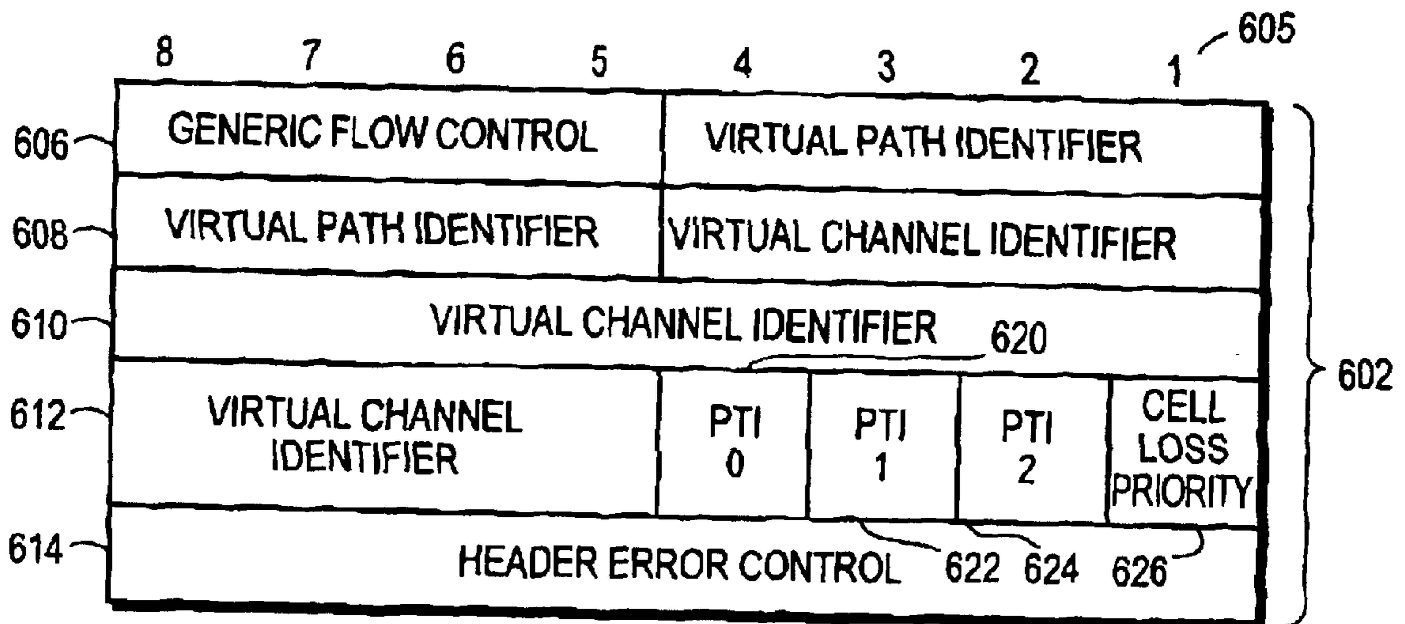
ATM CELL HEADER
