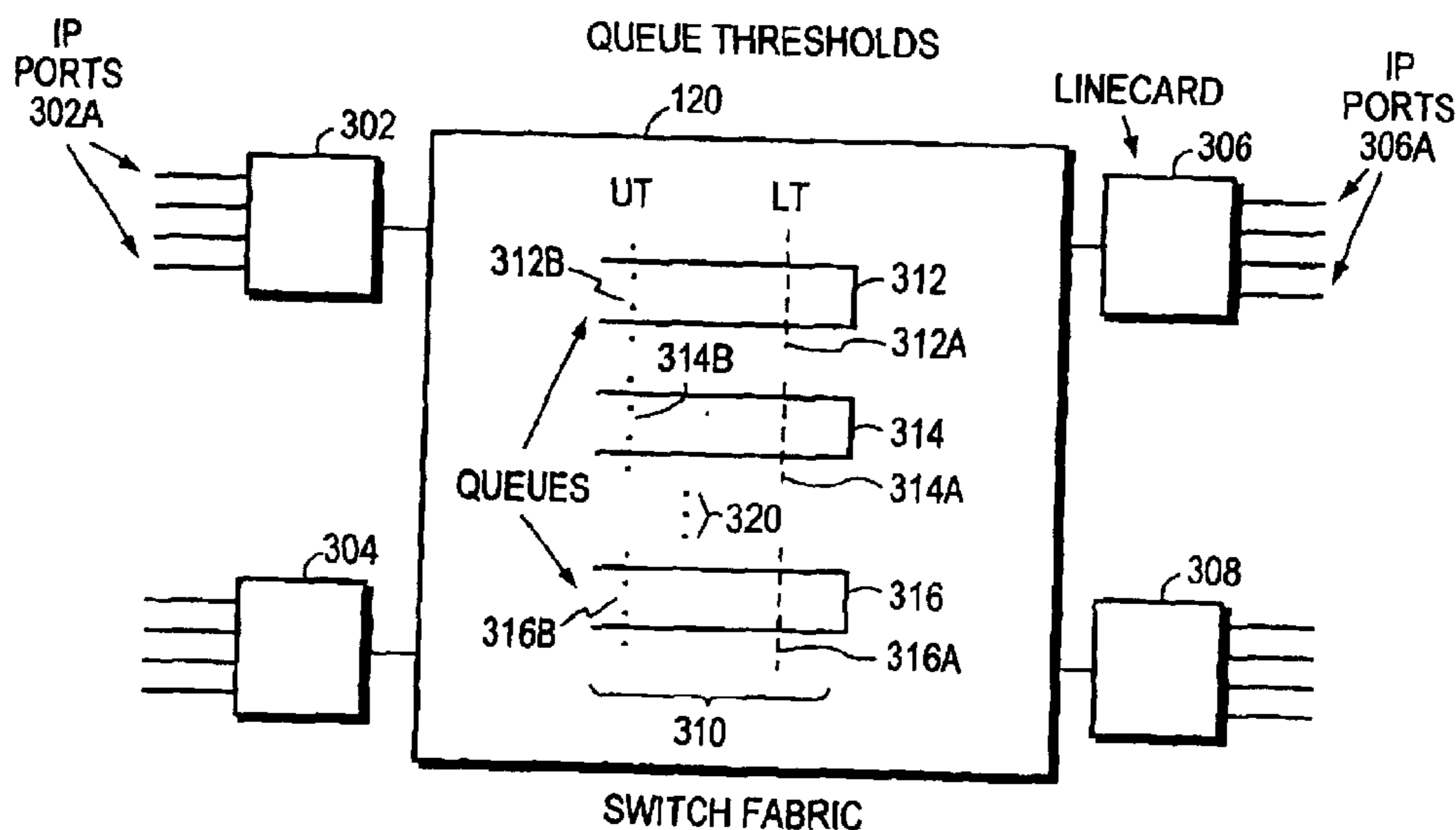
SWITCH FABRIC WITH LINECARDS, QUEUES AND THRESHOLDS
