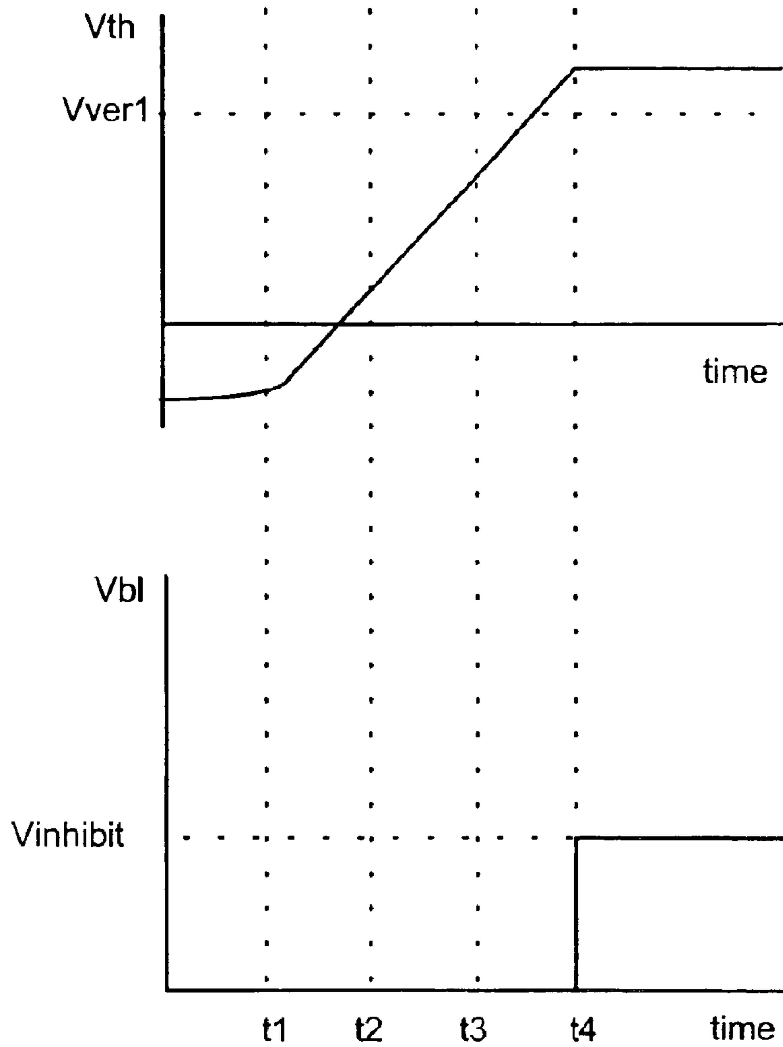
Fig. 2 (Prior Art)
