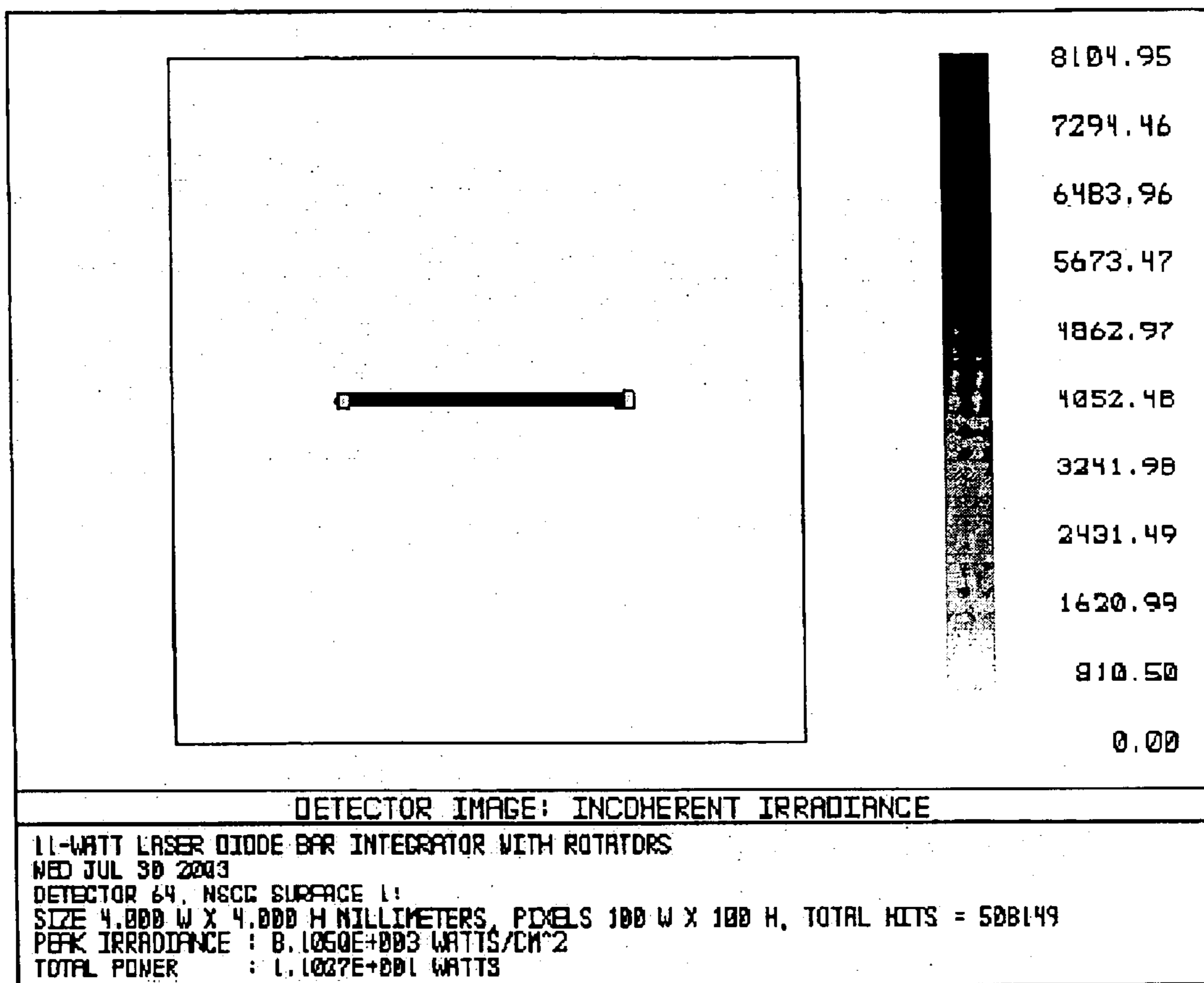
DETECTOR IMAGE: INCOHERENT IRRADIANCE
