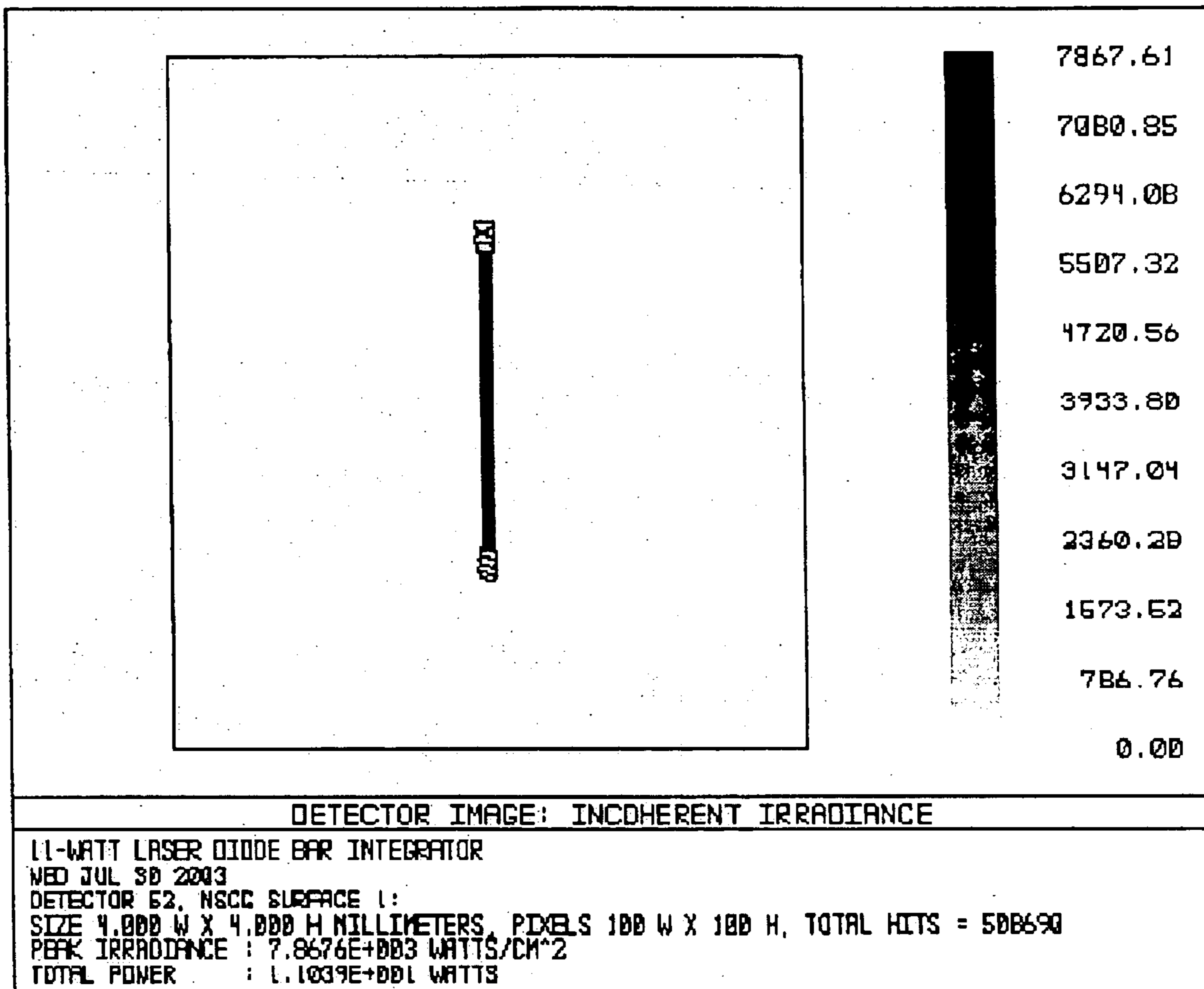
DETECTOR IMAGE: INCOHERENT IRRADIANCE
