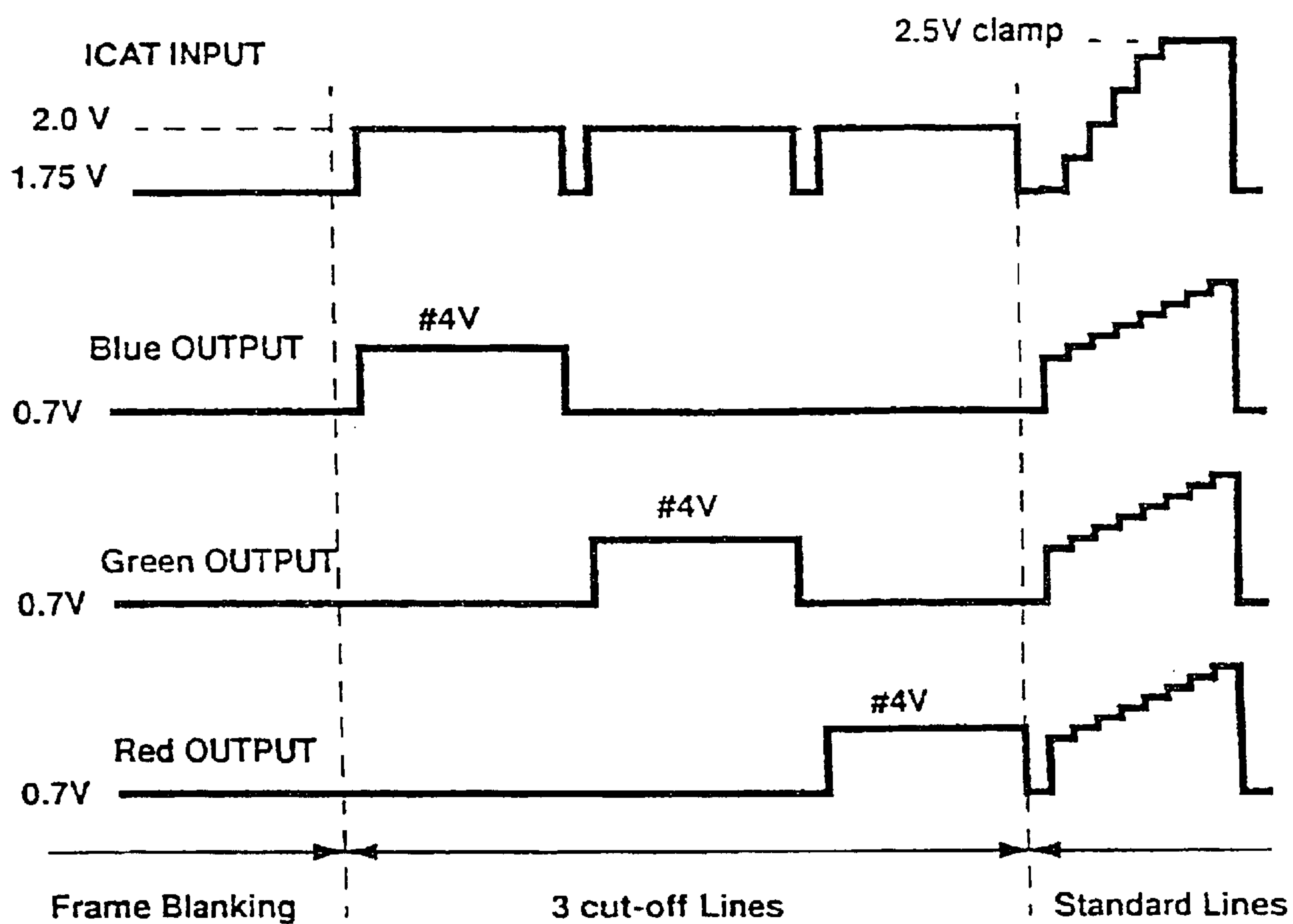
Fig 2: Waveforms at the RGB outputs and Icath input during the cut-off measurements lines
