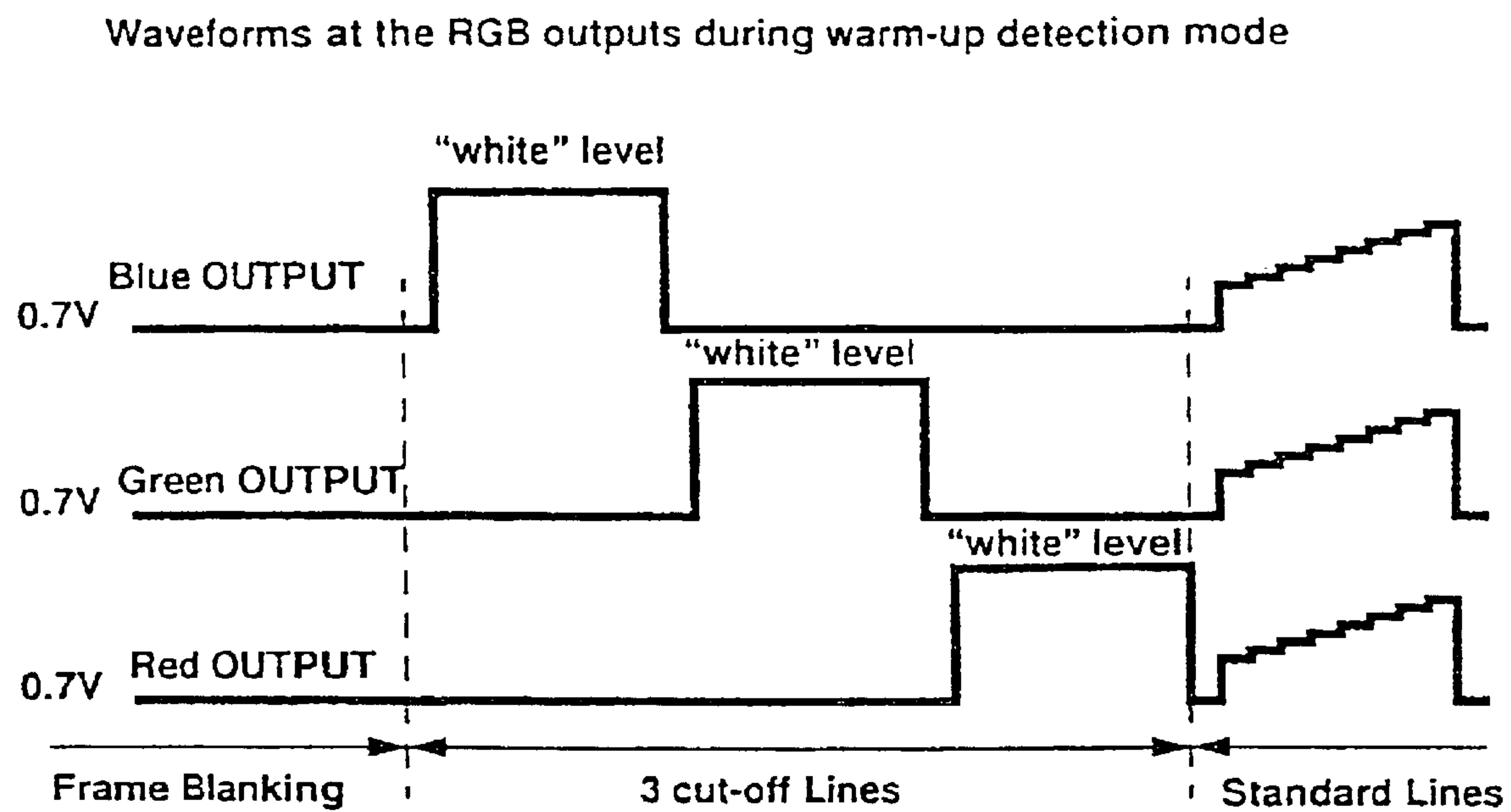
Fig 3: Waveforms at the RGB outputs during warm-up detection mode
