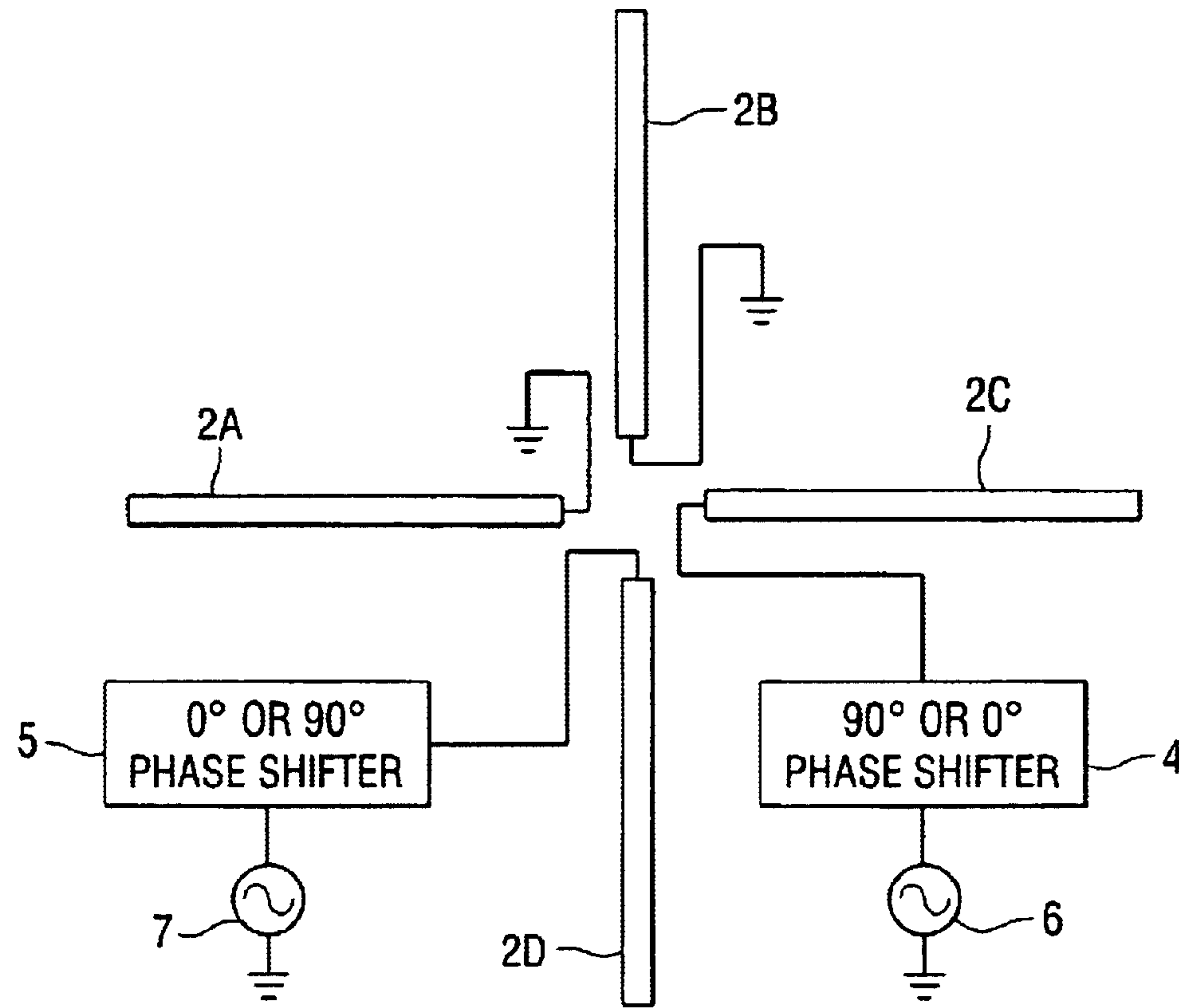
FIG. 1 PRIOR ART
