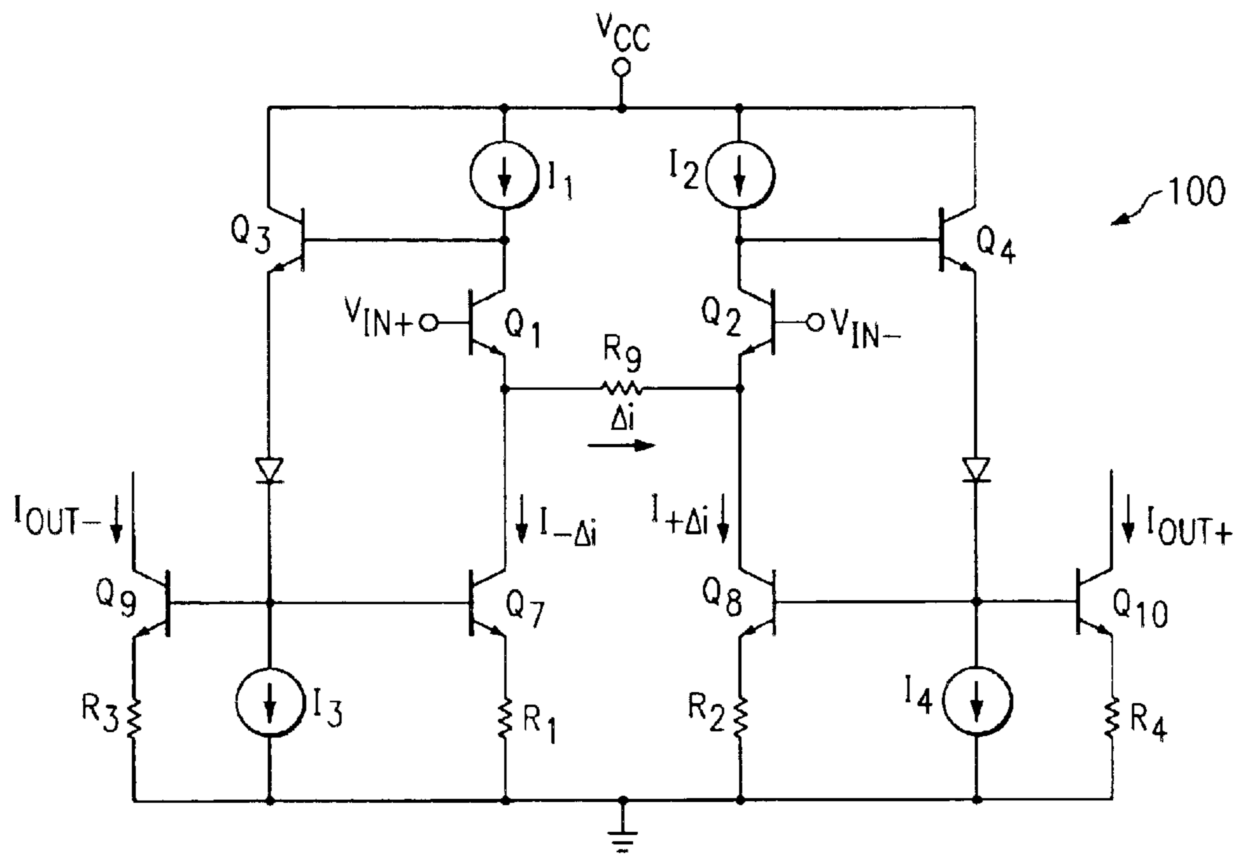
FIG. 1 (PRIOR ART)
