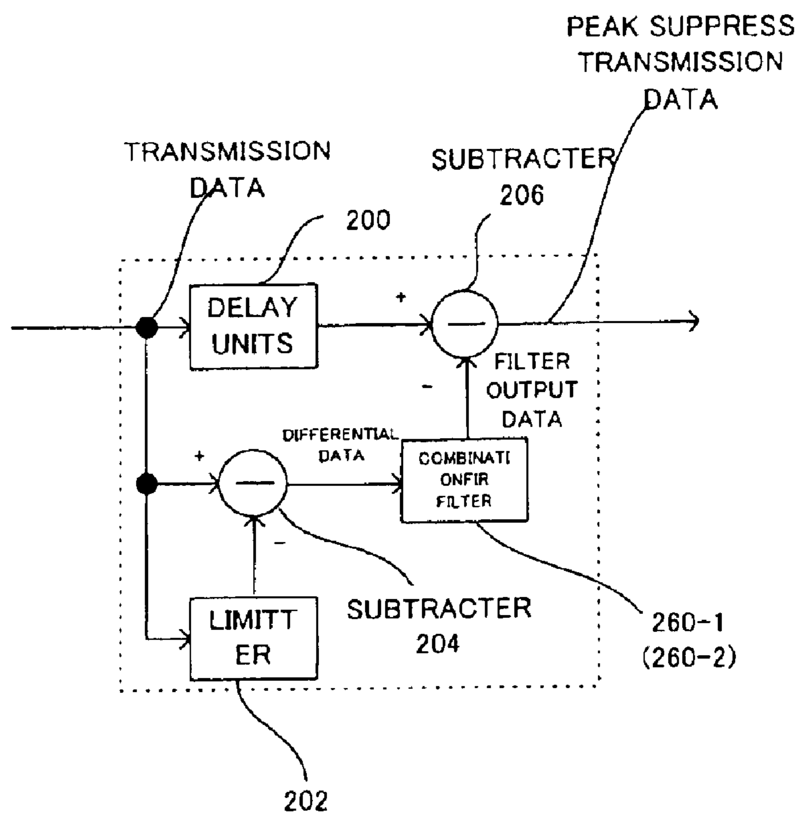
FOURTH PEAK SUPPRESSION UNIT 28-1(28-2)
