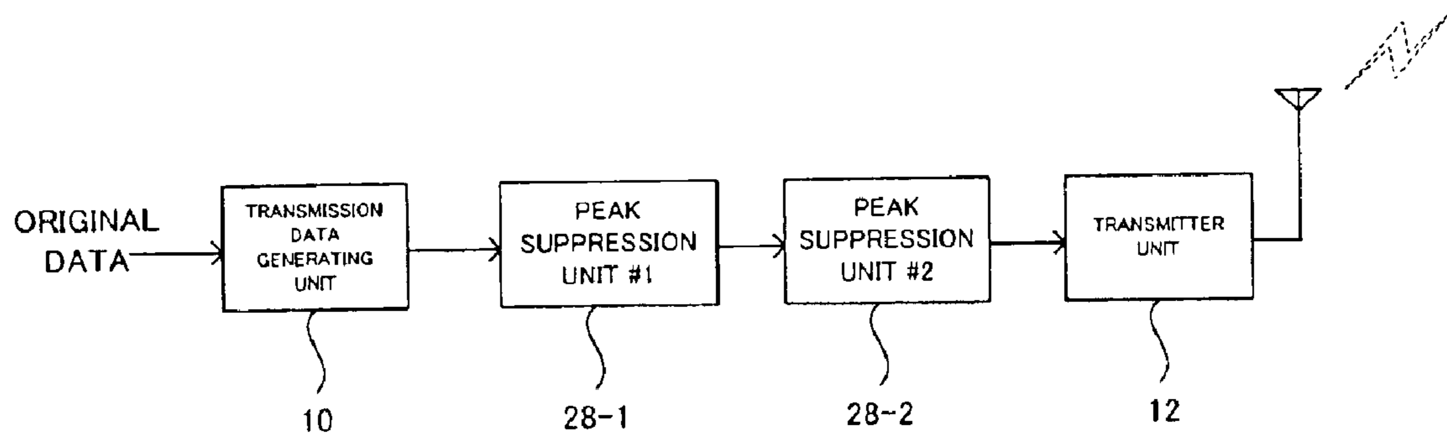
SIXTH OFDM TRANSMITTER 6
