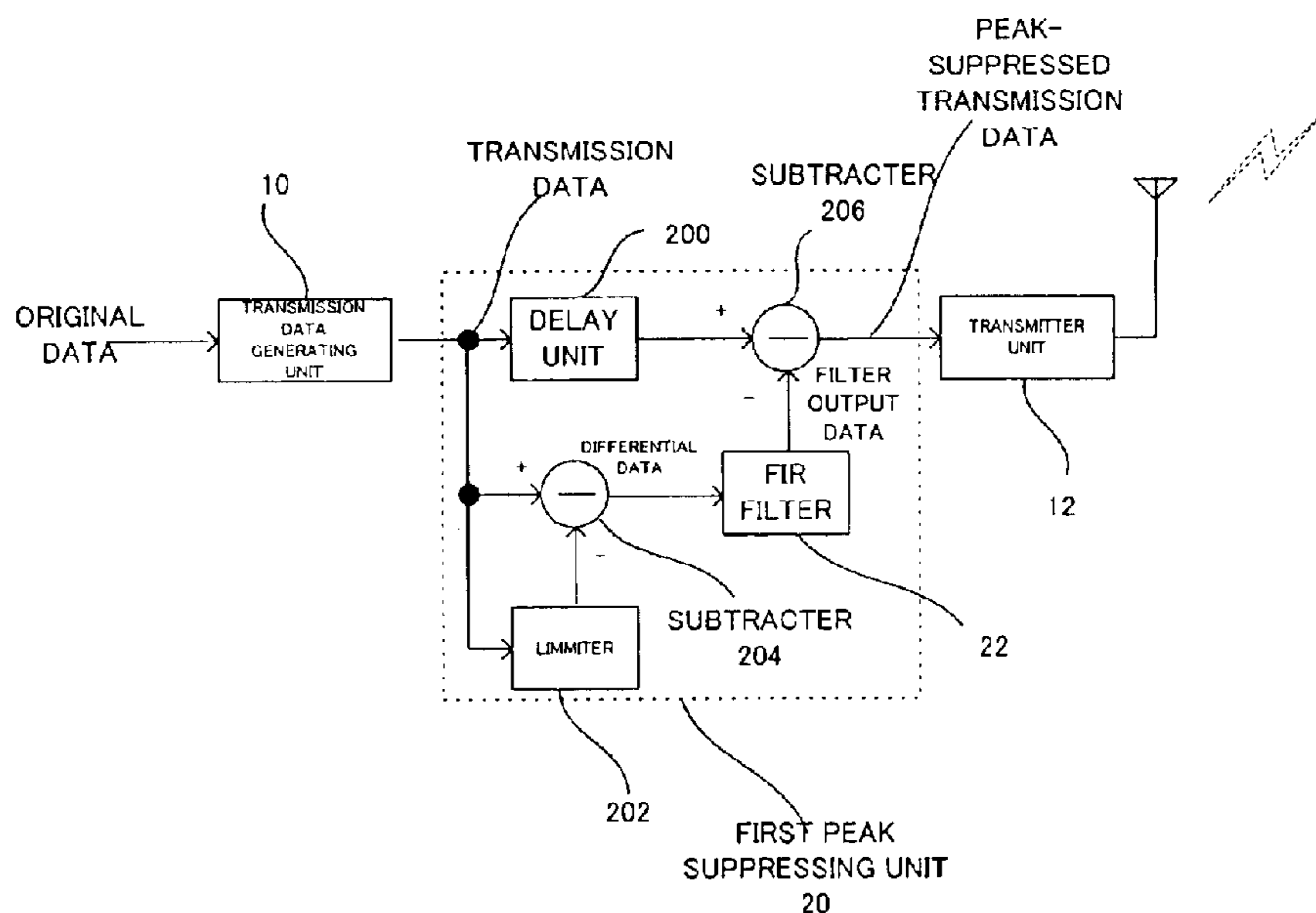
SECOND OFDM TRANSMITTER2
