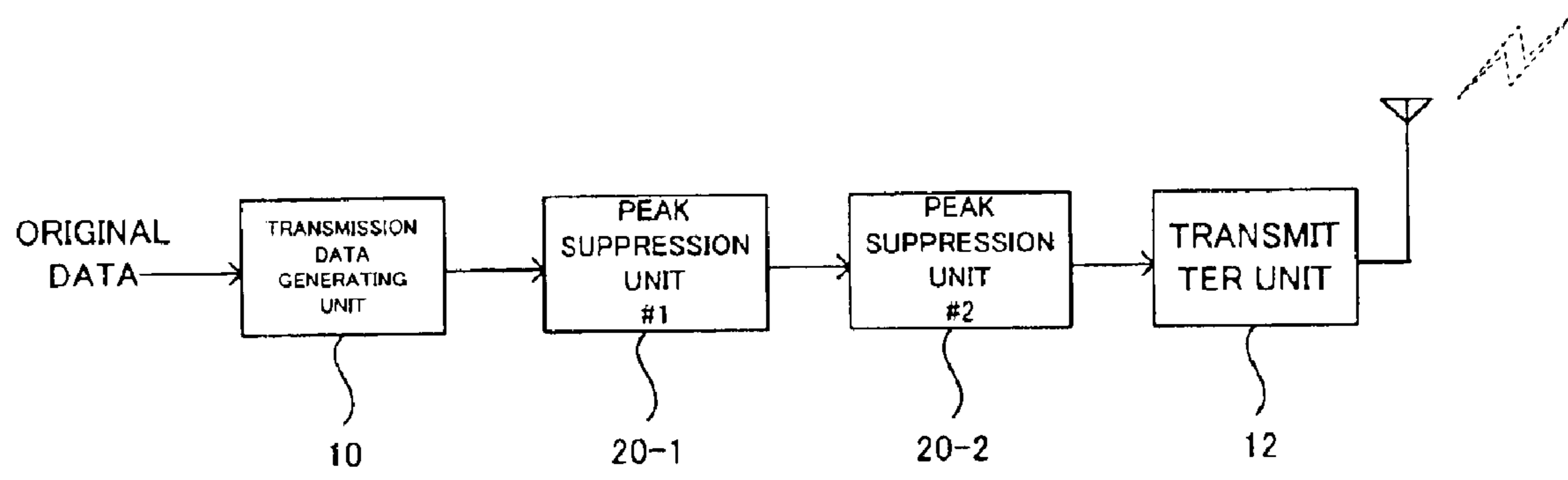
FOURTH OFDM TRANSMITTER 4
