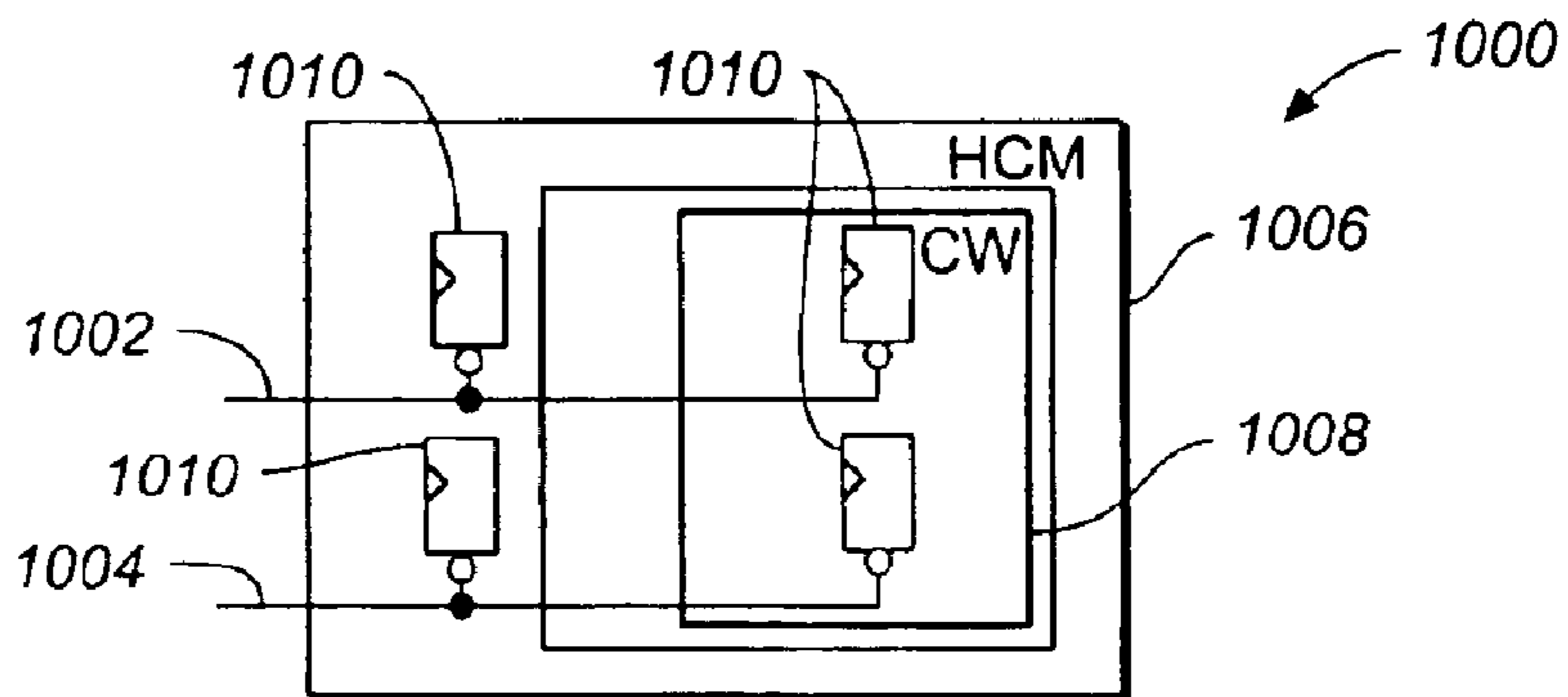
FIG. 10 (PRIOR ART)
