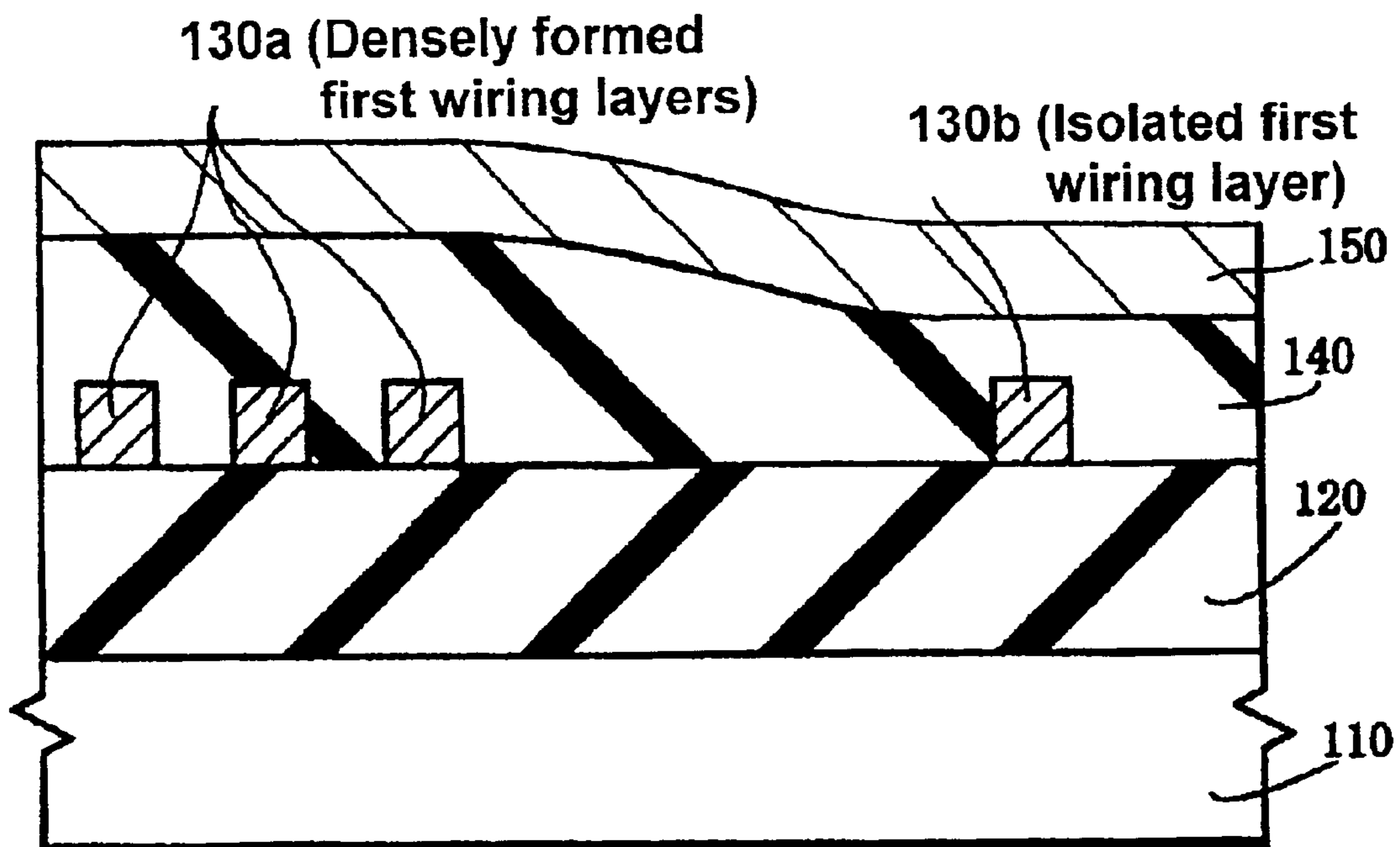
Fig. 18 (Prior Art)
