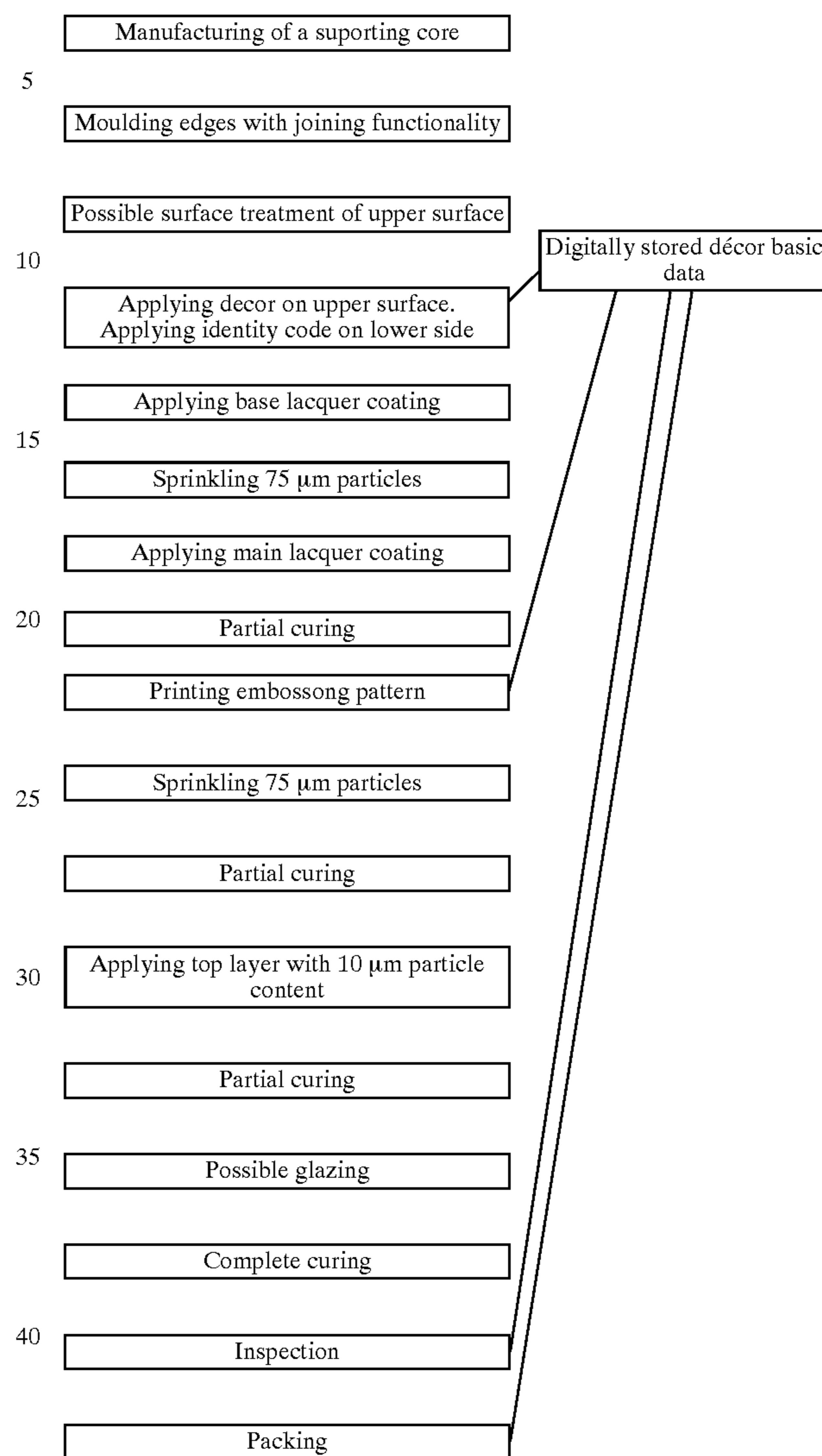
Process scheme 1.
