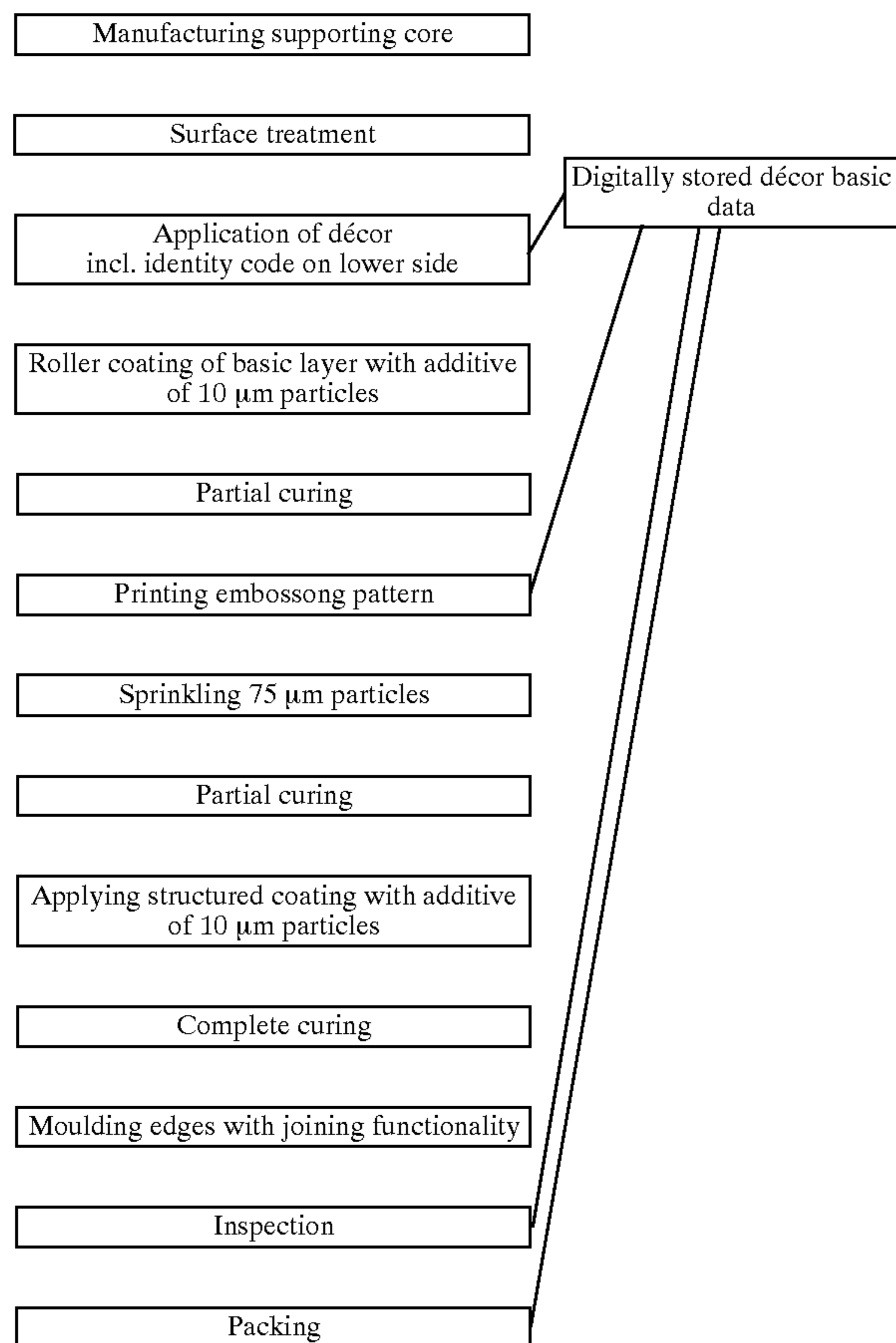
Process scheme 2
