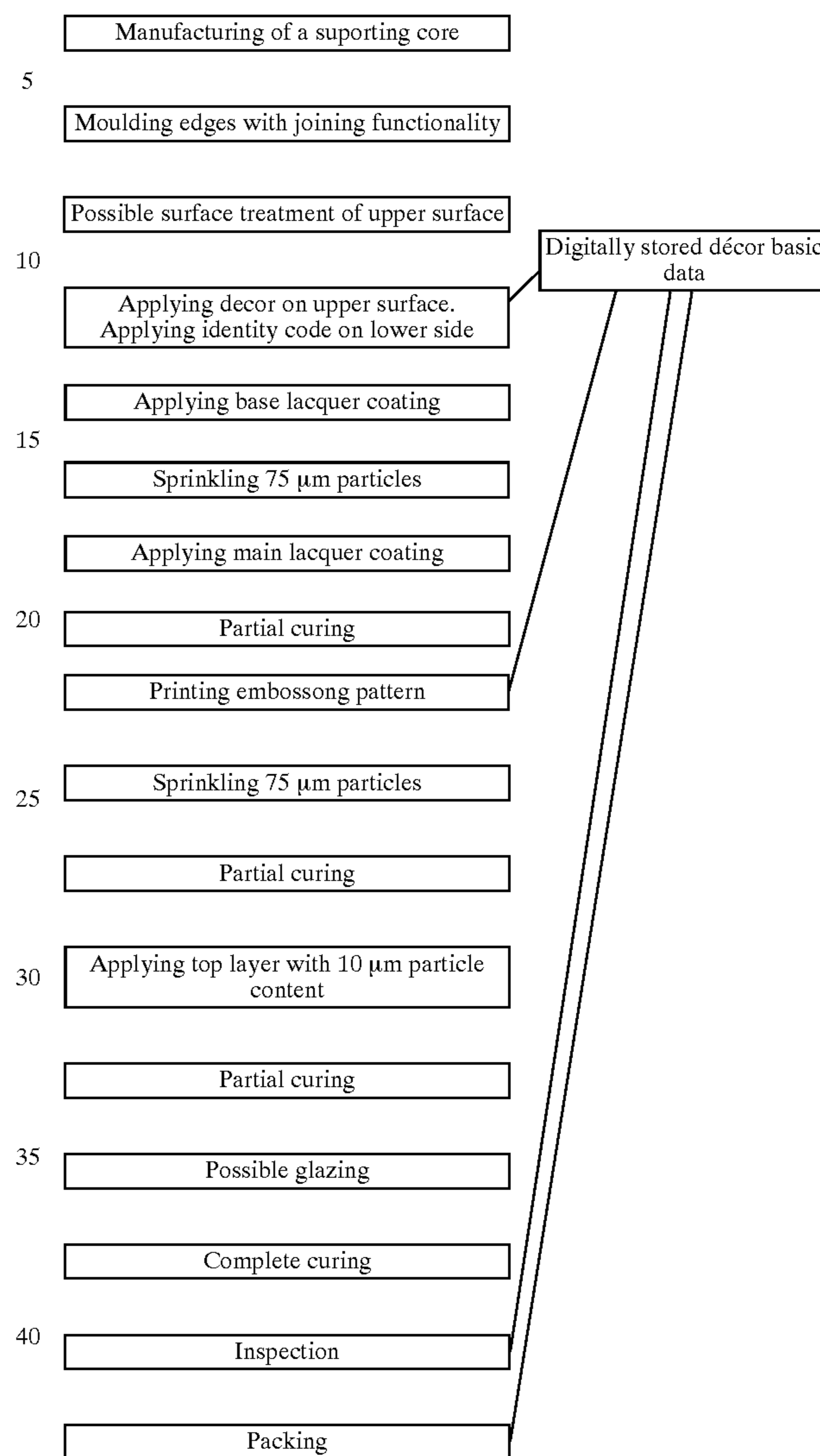
Process scheme 1.
