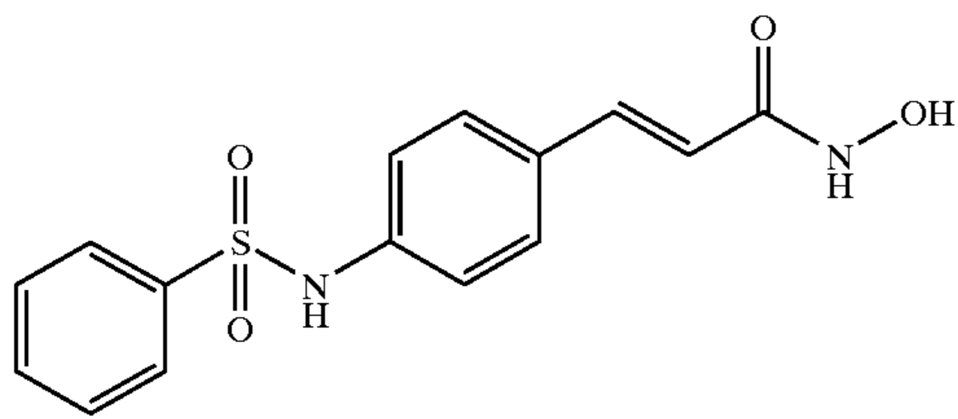
3-(4-Benzenesulfonylamino-phenyl)-N-hydroxyacrylamide (75) (PX106499)
