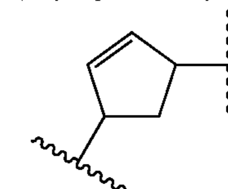
(4-cyclopenten-1,3-ylene)
