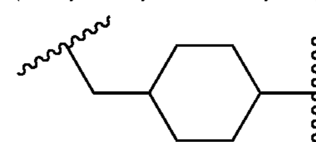
(methylene-cyclohex-1,4-ylene)
