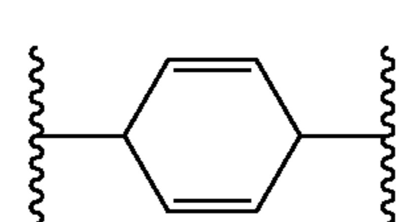
(2,5-cyclohexadien-1,4-ylene)
