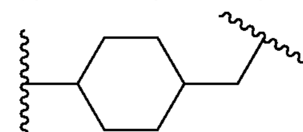
(cyclohex-1,4-ylene-methylene)
