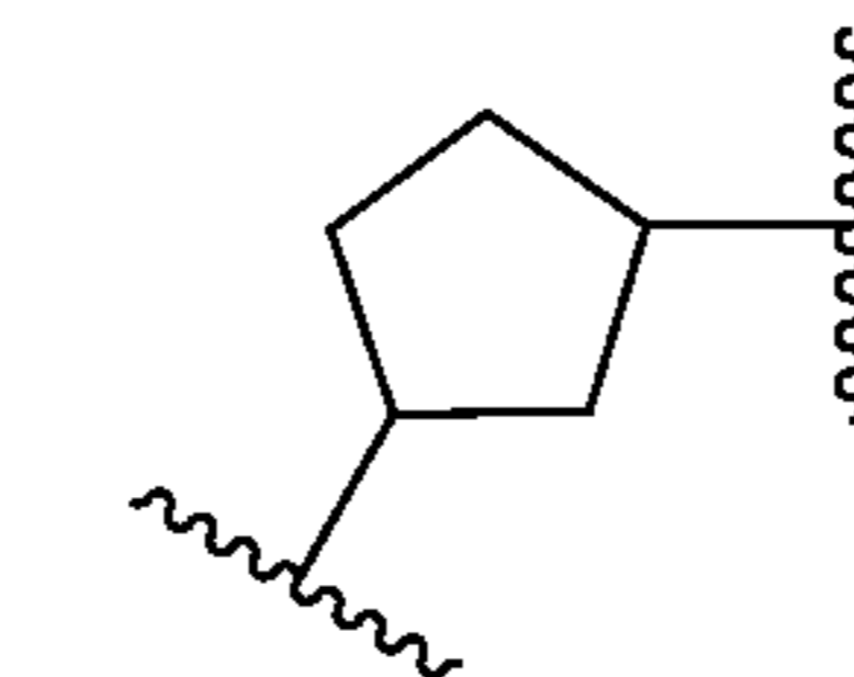
(cyclopent-1,3-ylene)
