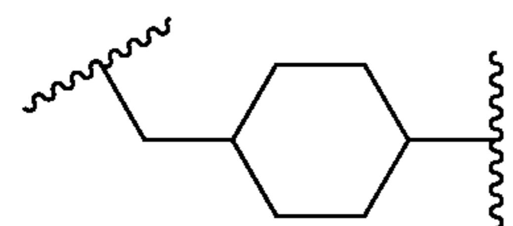
(methylene-cyclohex-1,4-ylene)
