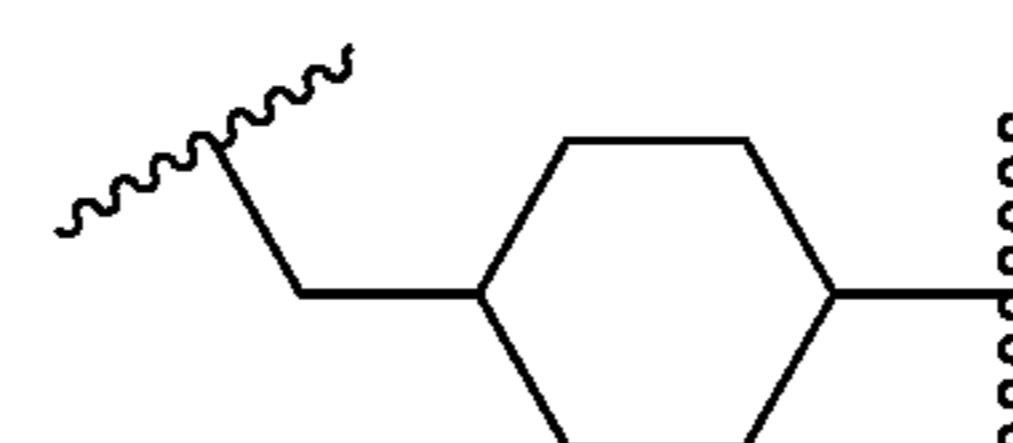
(methylene-cyclohex-1,4-ylene)
