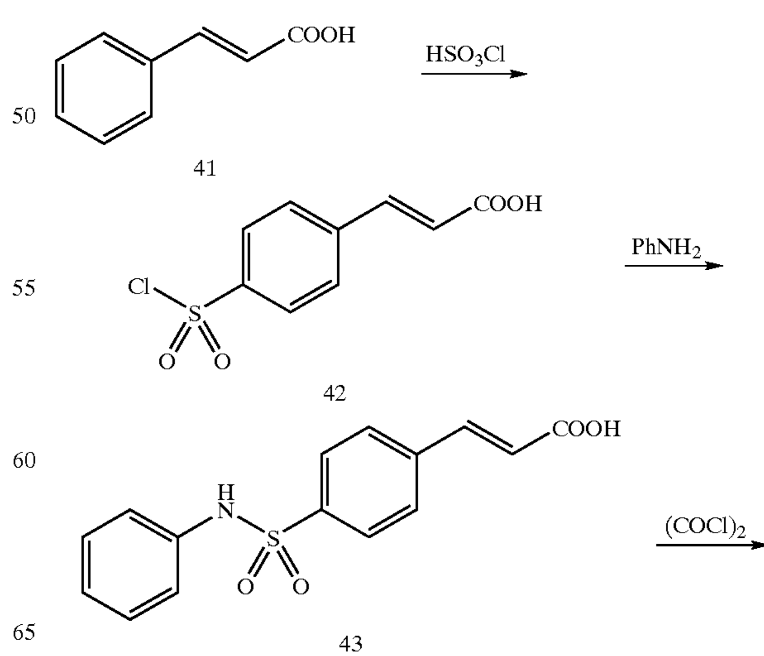
Scheme 5
