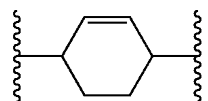
(2-cyclohexen-1,4-ylene)
