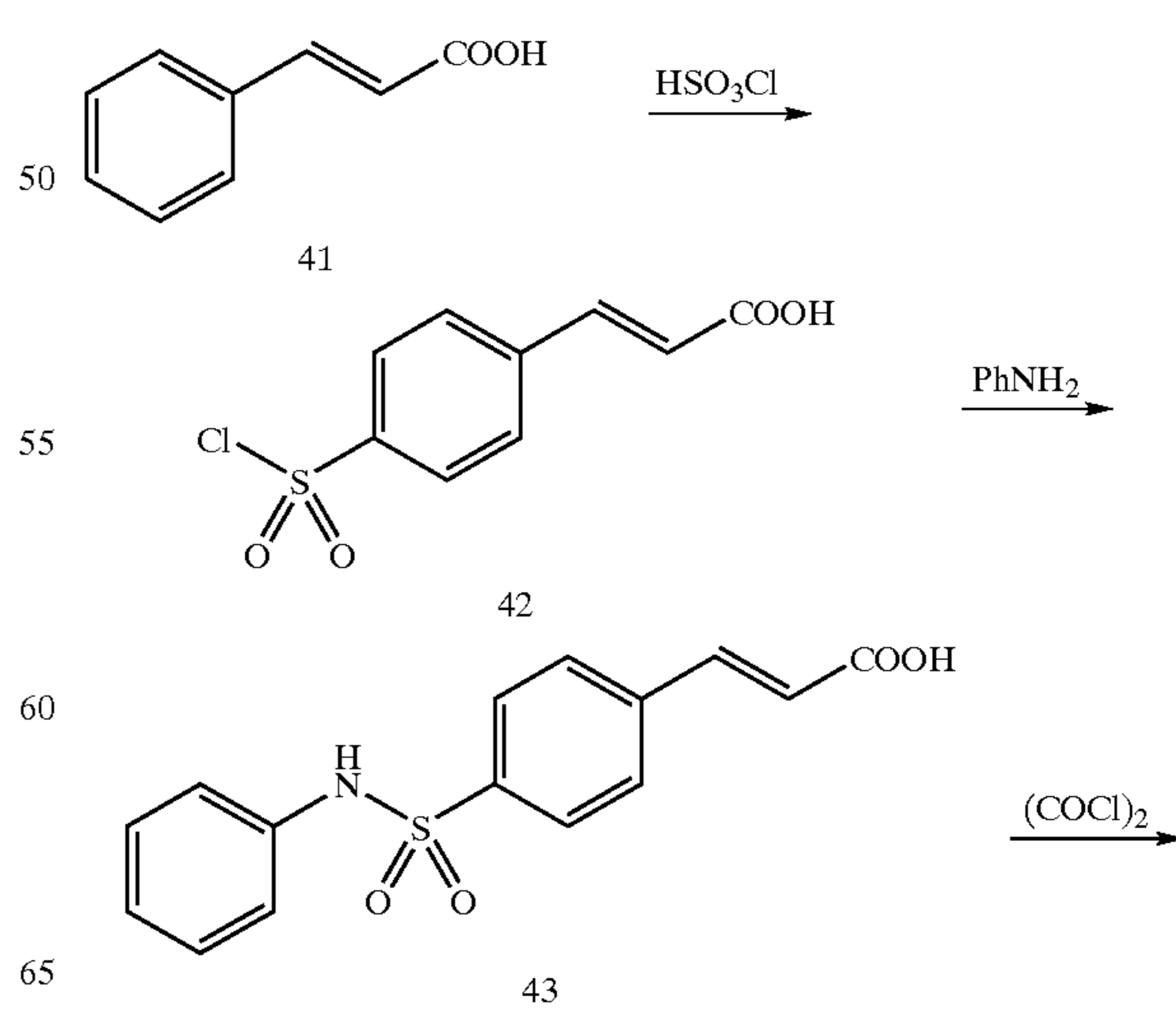
Scheme 5
