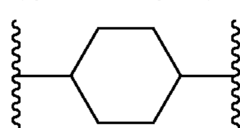
(cyclohex-1,4-ylene)
