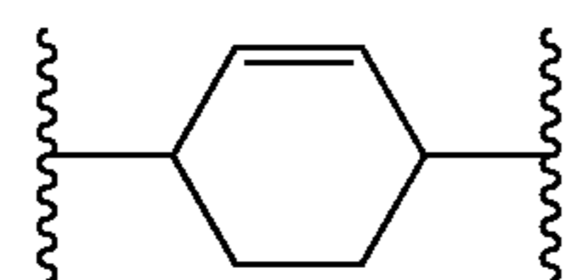
(2-cyclohexen-1,4-ylene)
