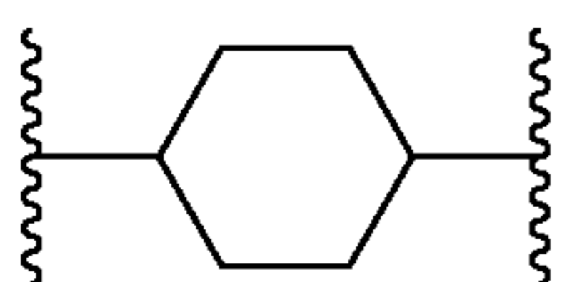
(cyclohex-1,4-ylene)
