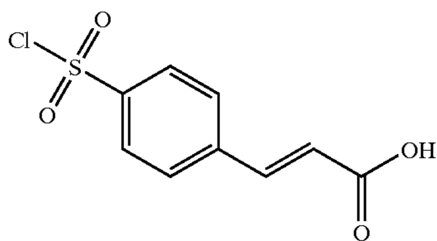
3-(4-Chlorosulfonyl-phenyl)-acrylic acid (42)
