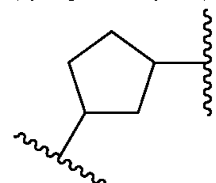
(cyclopent-1,3-ylene)
