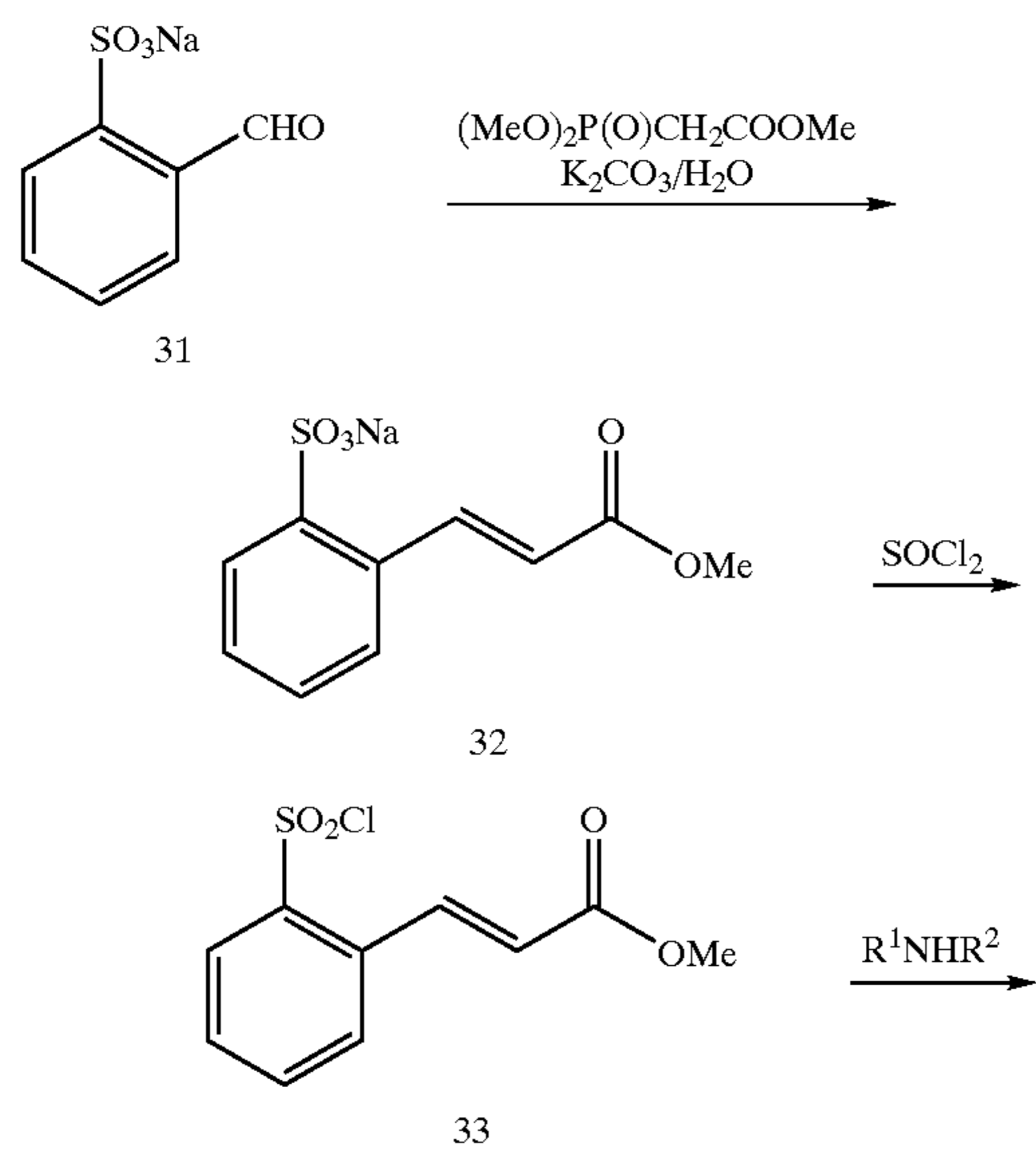
Scheme 4
