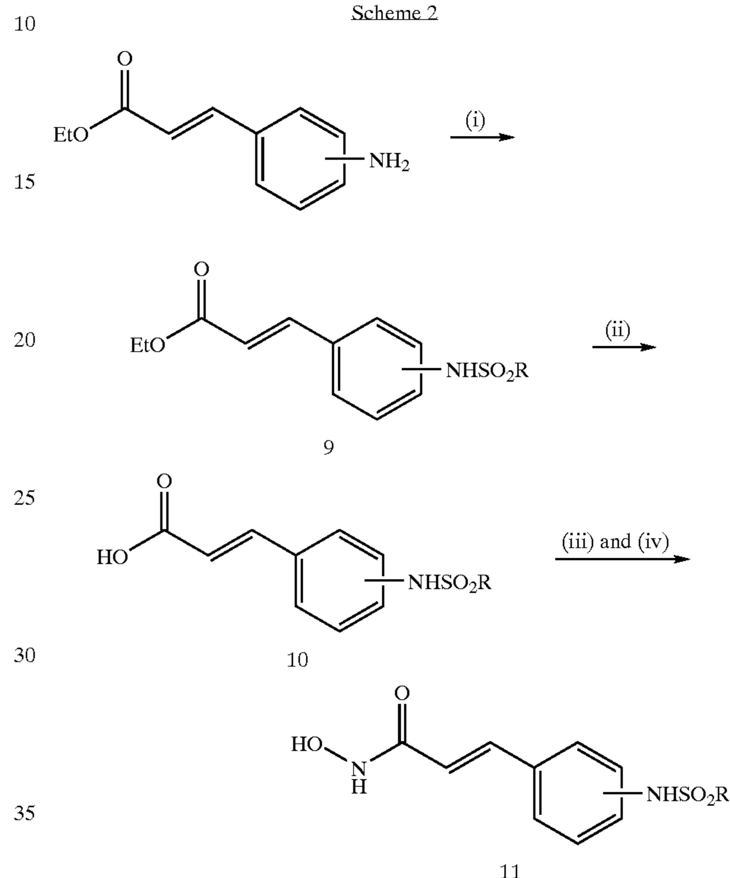
Scheme 2
