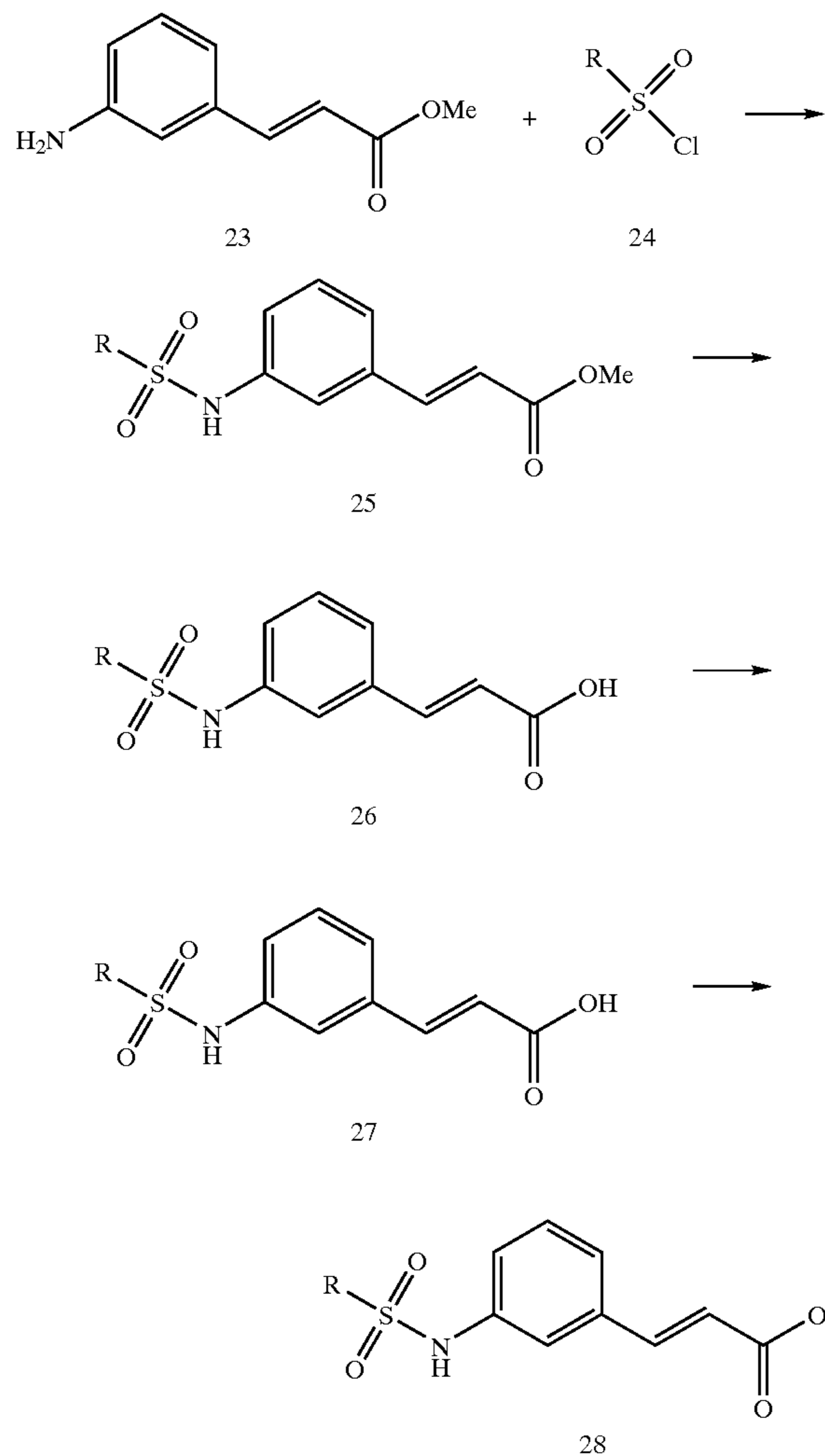
Scheme 3B
