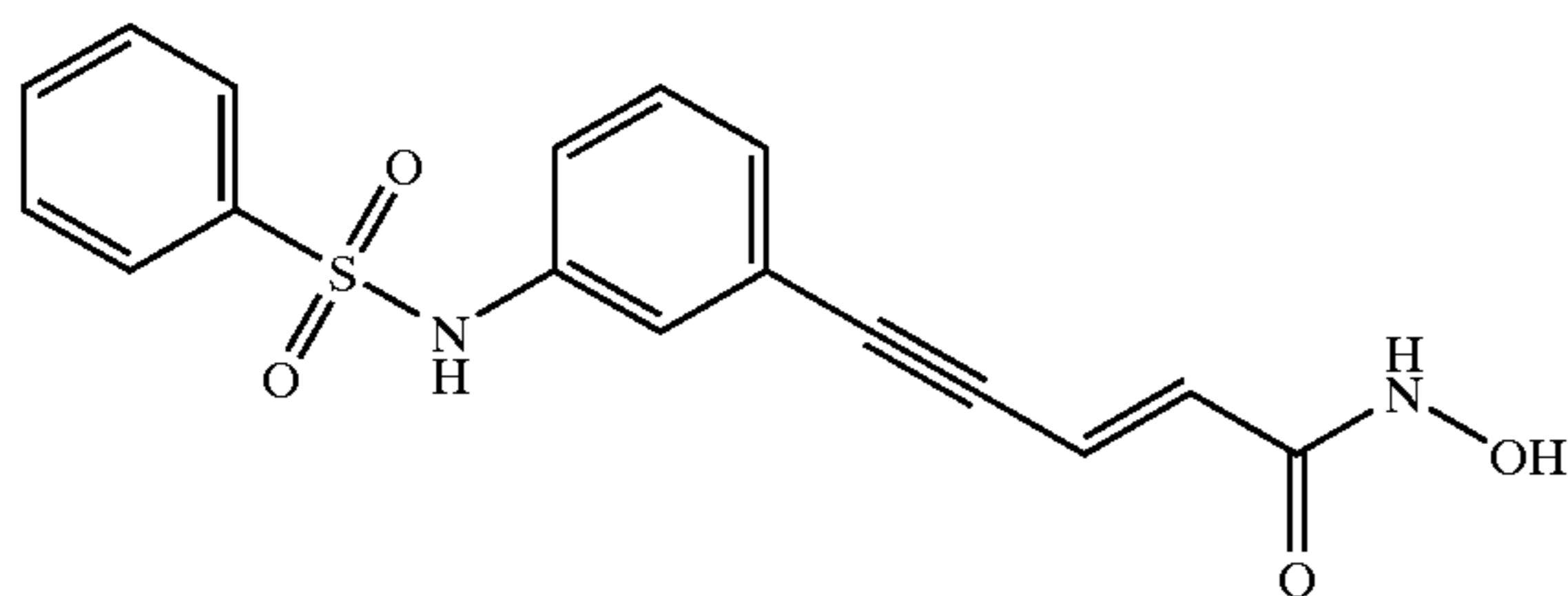
Oxamflatin
