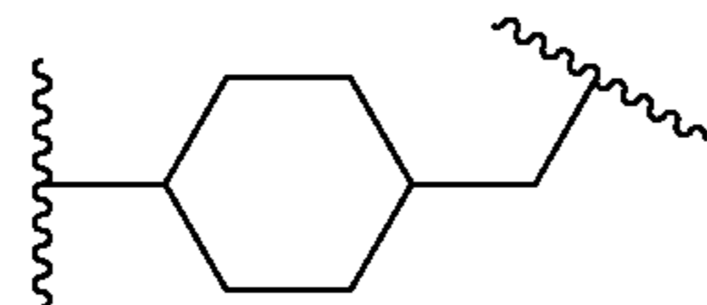
(cyclohex-1,4-ylene-methylene)
