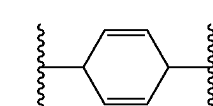
(2,5-cyclohexadien-1,4-ylene)
