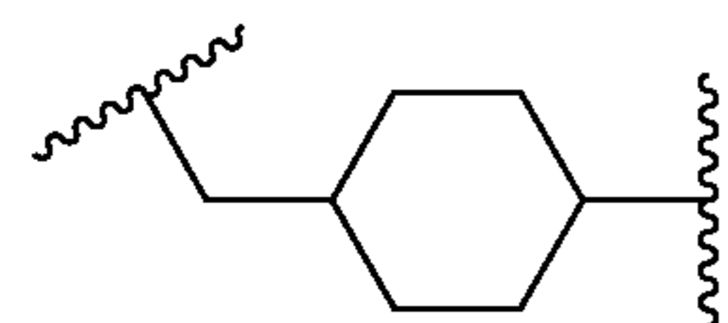
(methylene-cyclohex-1,4-ylene)
