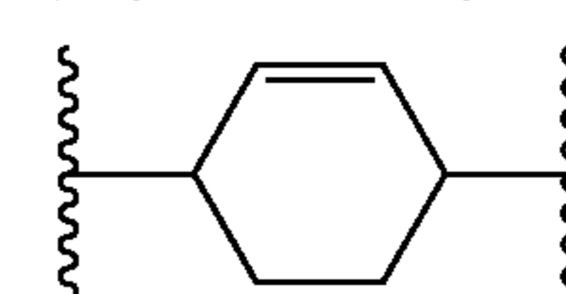
(2-cyclohexen-1,4-ylene)
