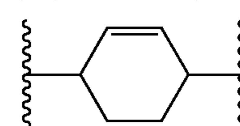
(2-cyclohexen-1,4-ylene)
