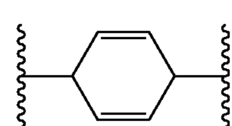
(2,5-cyclohexadien-1,4-ylene)
