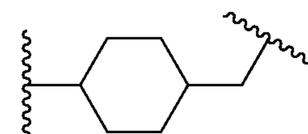
(cyclohex-1,4-ylene-methylene)
