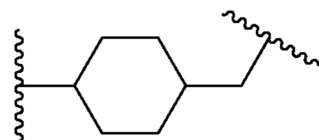
(cyclohex-1,4-ylene-methylene)
