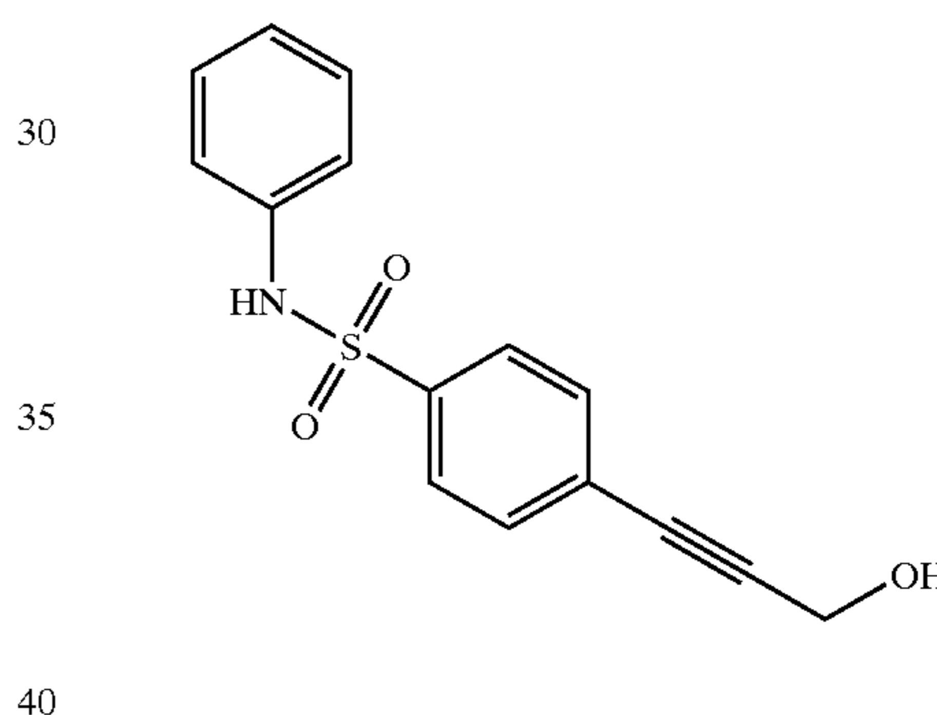
4-(3-Hydroxyprop-1-ynyl)-N-phenylbenzenesulfonamide (53b)
