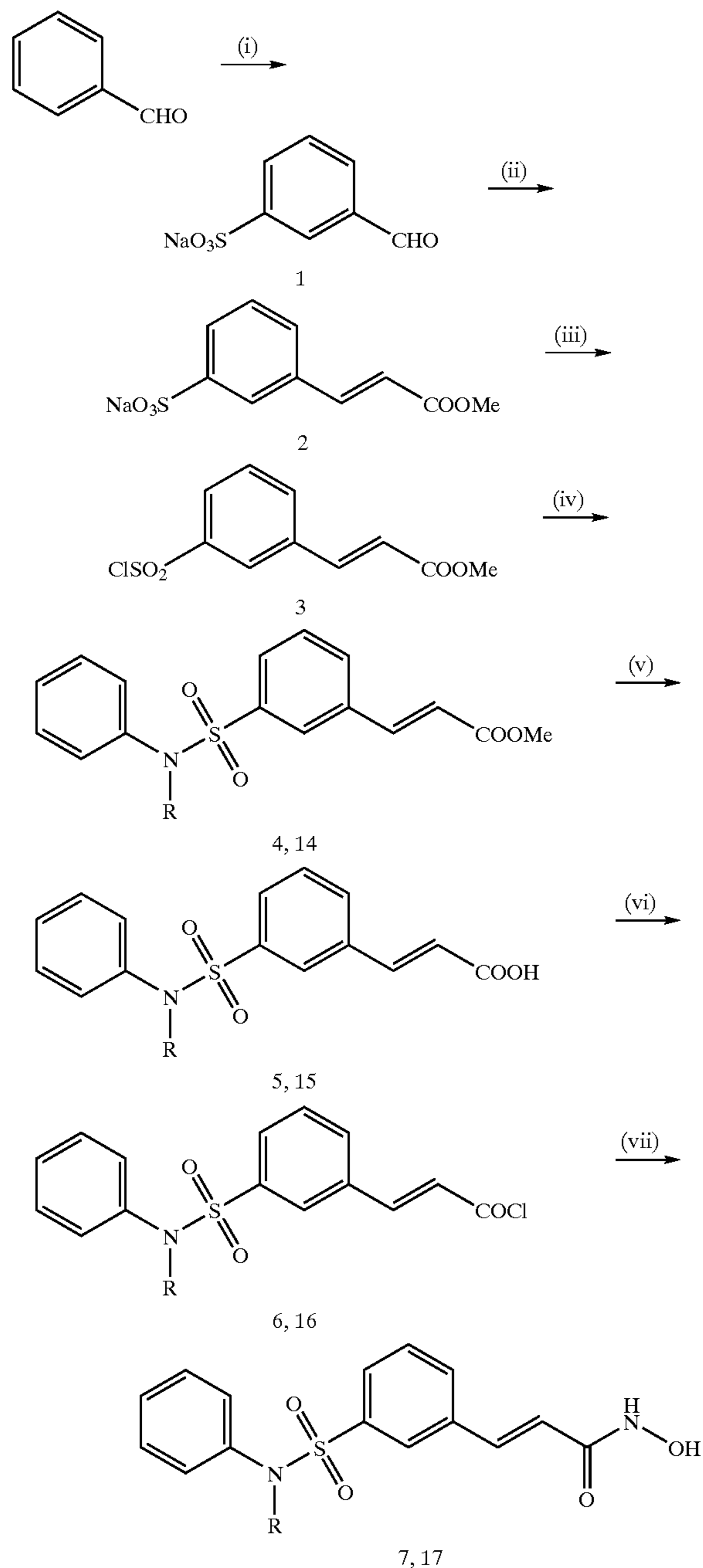
Scheme 1
