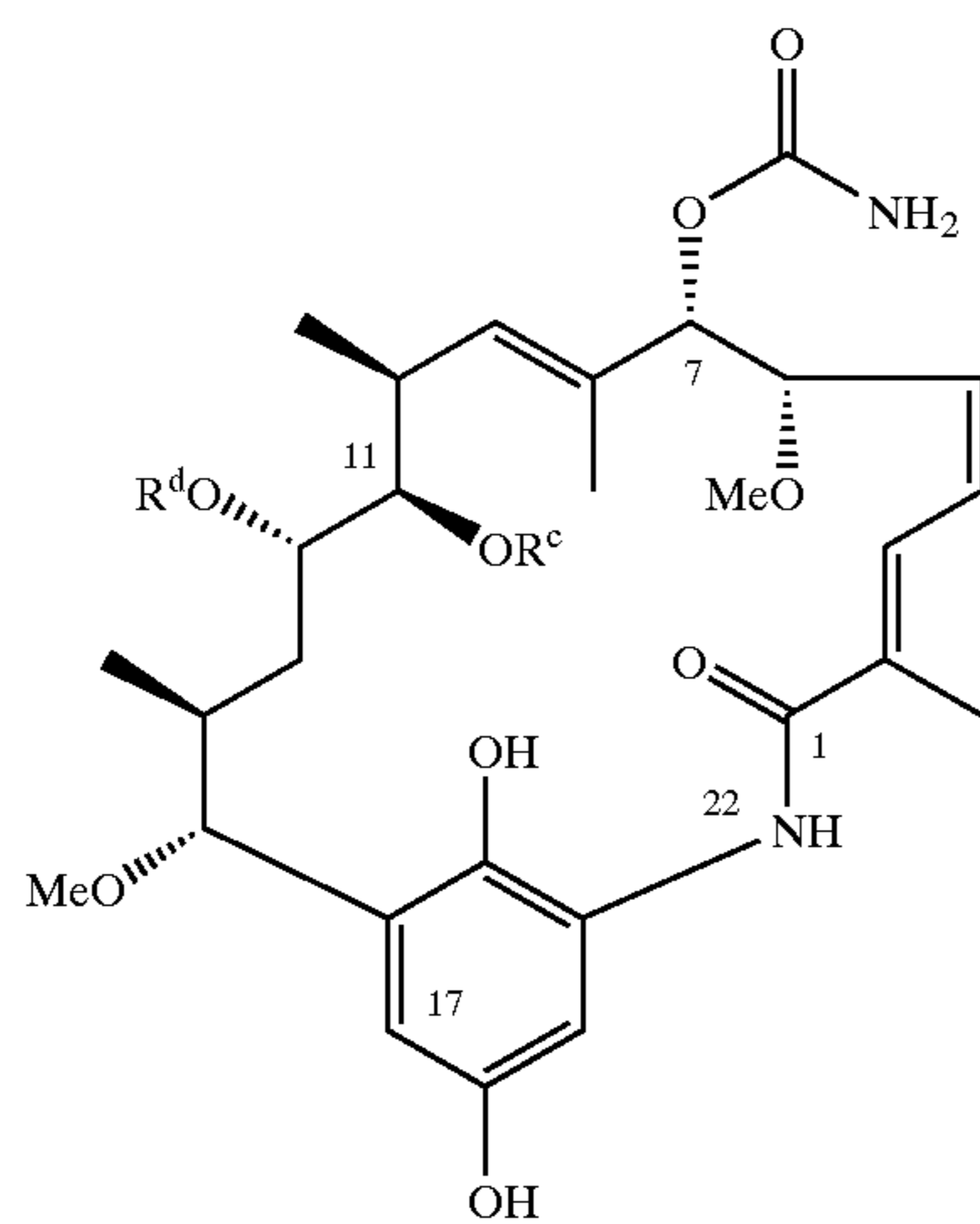
TAN-420 A: R c = H; R d = H C: R c = H; R d = Me E: R c = Me; R d = Me
