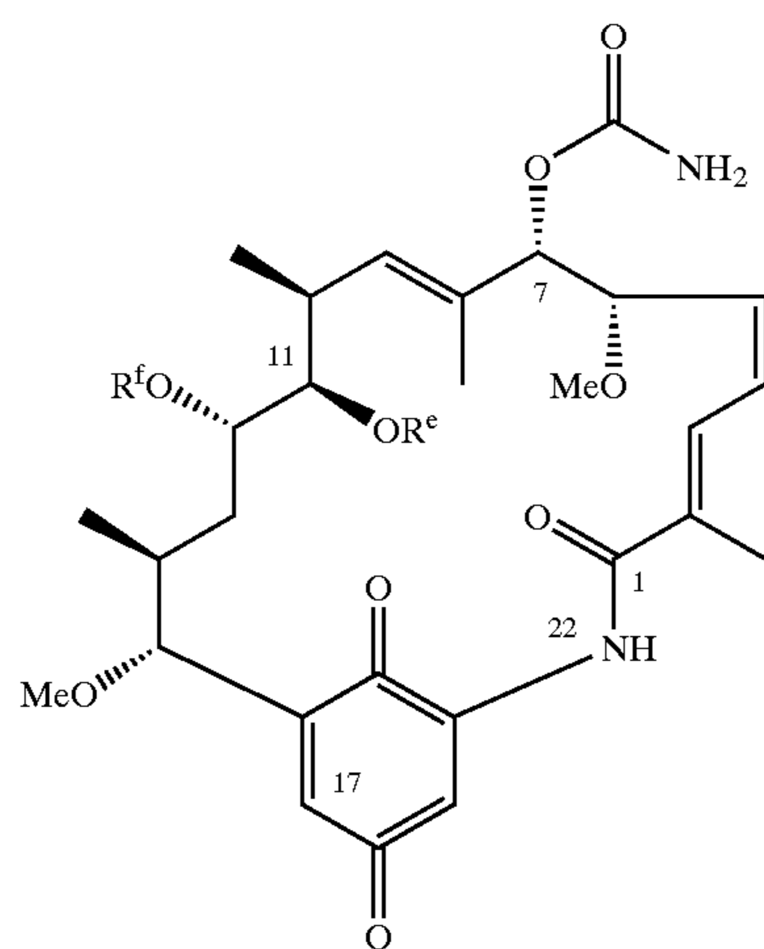
TAN-420 B: R e = H; R f = H D: R e = H; R f = Me
