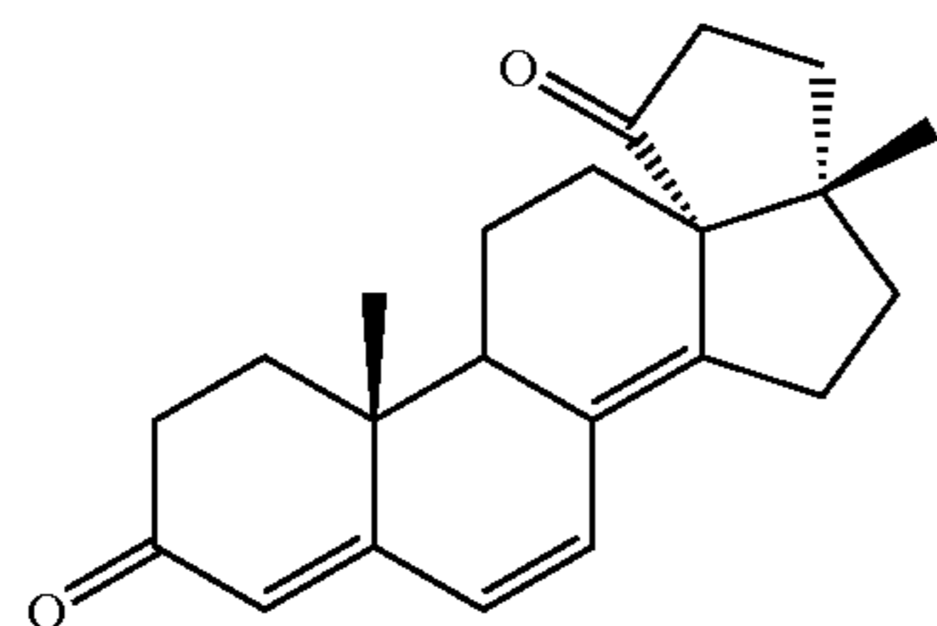
[13S, 17 \beta ]-3', 4'-dihydro-17-methyl-cyclopenta[13, 17]-18-norandrosta-4, 6, 8(14)-triene-3, 5'[2'H]-dione
