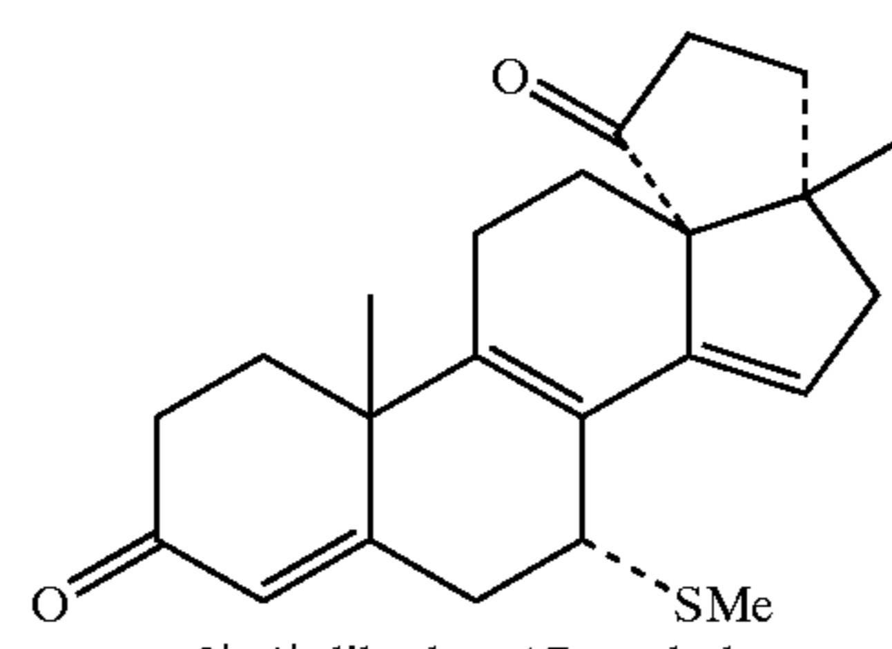
3', 4'-dihydro-17-methyl-7 \alpha -(methylthio)-cyclopenta[13, 17]-18-norandrosta-4, 8, 14-triene-3, 5'(2'H)-dione
