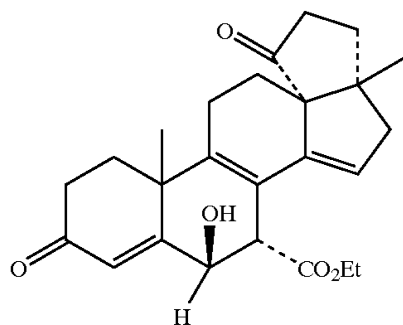
ethyl 3', 4', 5', 17-tetrahydro-6β-hydroxy-17β-methyl-3, 5'-dioxocyclopenta[13R, 17]-18-norandrosta-4, 8, 14-triene-7α-carboxylate
