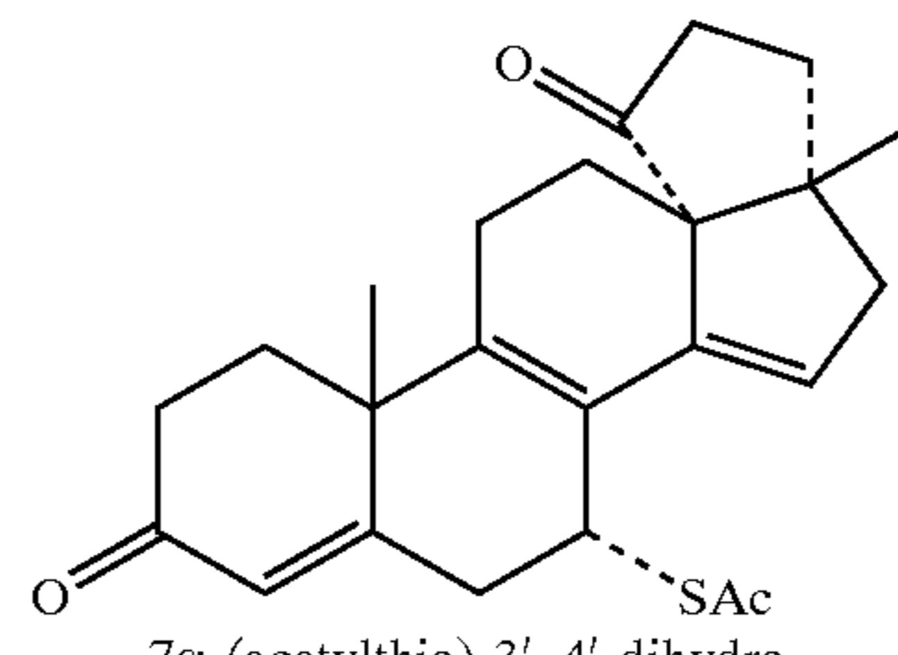
7 \alpha -(acetylthio)-3', 4'-dihydro-17-methyl-cyclopenta[13, 17]-18-norandrosta-4, 8, 14-triene-3, 5'(2'H)-dione
