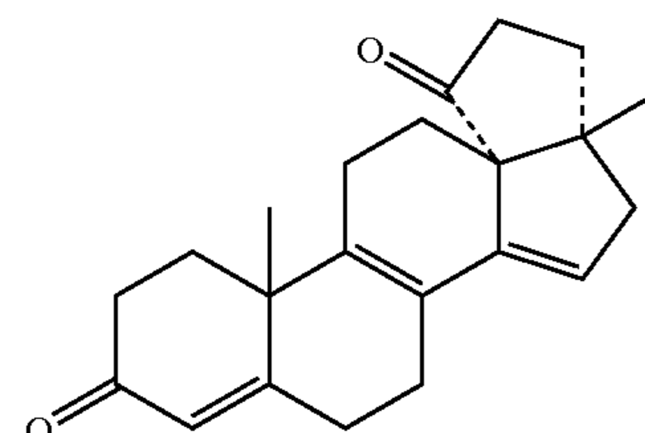
3', 4', 5', 17-tetrahydro-17β-methylcyclopenta[13R, 17]-18-norandrosta-4, 8, 14-triene-3, 5' (2'H)-dione
