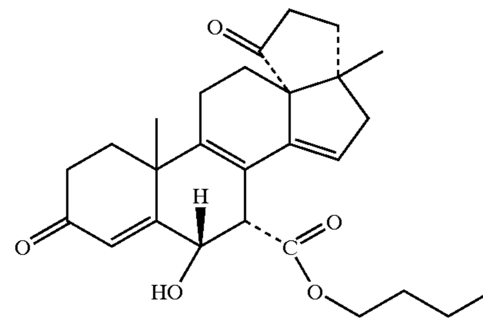
butyl 3', 4', 5', 17-tetrahydro-6α-hydroxy-17β-methyl-3, 5'-dioxocyclopenta[13R, 17]-18-norandrosta-4, 8, 14-triene-7α-carboxylate
