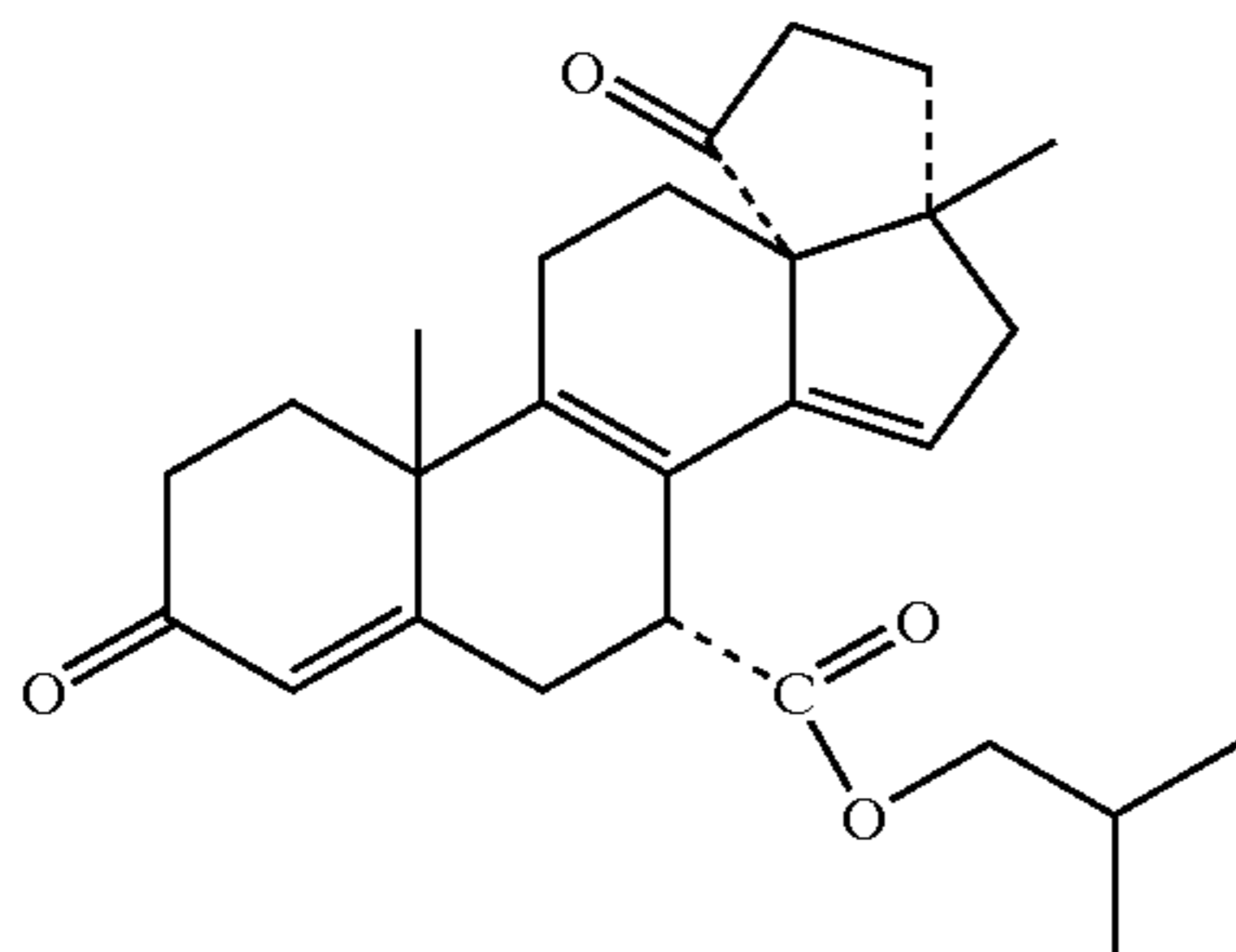
2-methylpropyl 3', 4', 5', 17-tetrahydro-17β-methyl-3, 5'-dioxocyclopenta [13R, 17]-18-norandrosta-4, 8, 14-triene-7α-carboxylate
