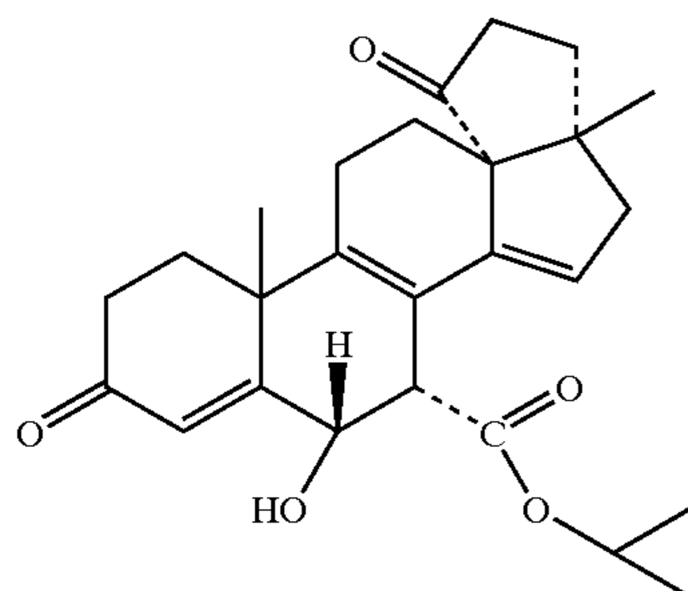
1-methylethyl 3', 4', 5', 17-tetrahydro-6α-hydroxy-17β-methyl-3, 5'-dioxocyclopenta[13R, 17]-18-norandrosta-4, 8, 14-triene-7α-carboxylate
