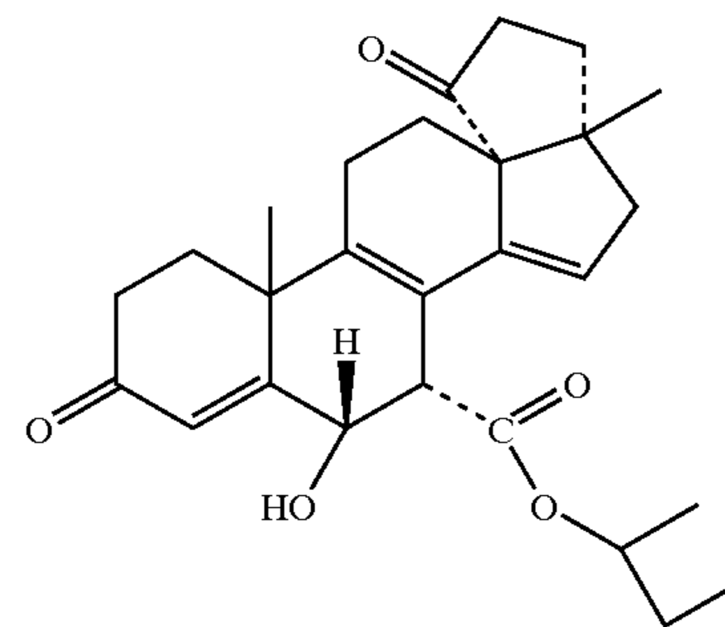
1-methylpropyl 3', 4', 5', 17-tetrahydro-6α-hydroxy-17β-methyl-3, 5'-dioxocyclopenta[13R, 17]-18-norandrosta-4, 8, 14-triene-7α-carboxylate
