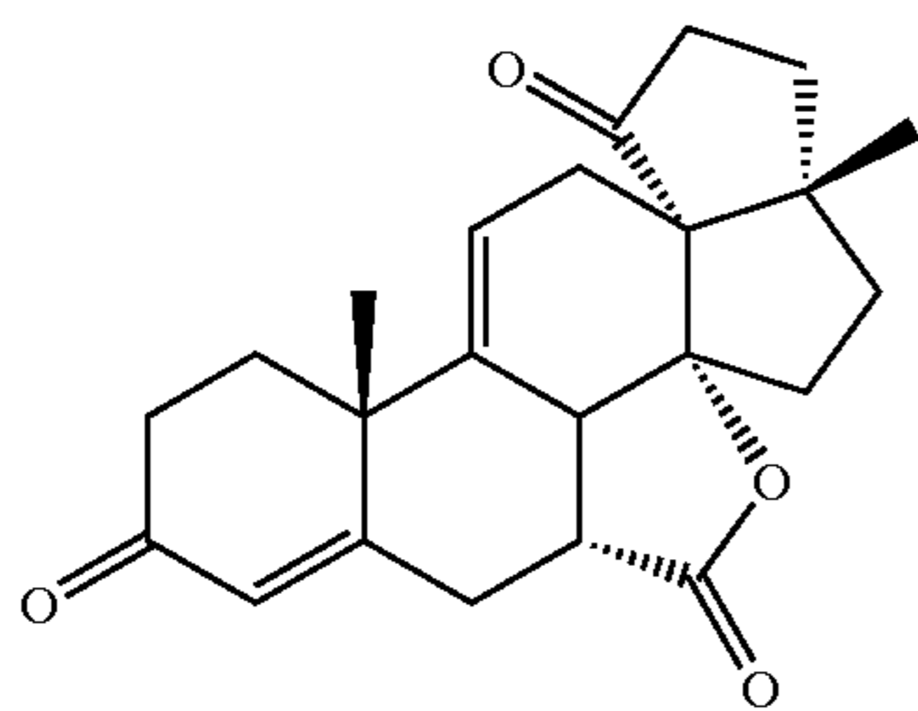
(7 \alpha , 13R, 17 \beta )-3', 4', 5', 17-tetrahydro-14-hydroxy-17-methyl-3, 5'-dioxo- \gamma -lactone, cyclopenta[13, 17]-18-norandrosta-4, 9(11)-diene-7-carboxylic acid
