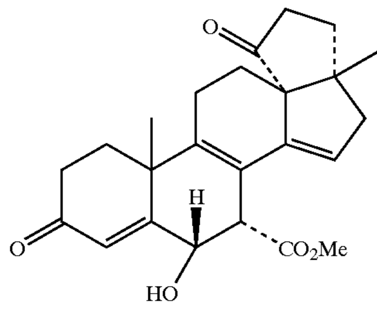
methyl 3', 4', 5', 17-tetrahydro-6α-hydroxy-17β-methyl-3, 5'-dioxocyclopenta[13R, 17]-18-norandrosta-4, 8, 14-triene-7α-carboxylate
