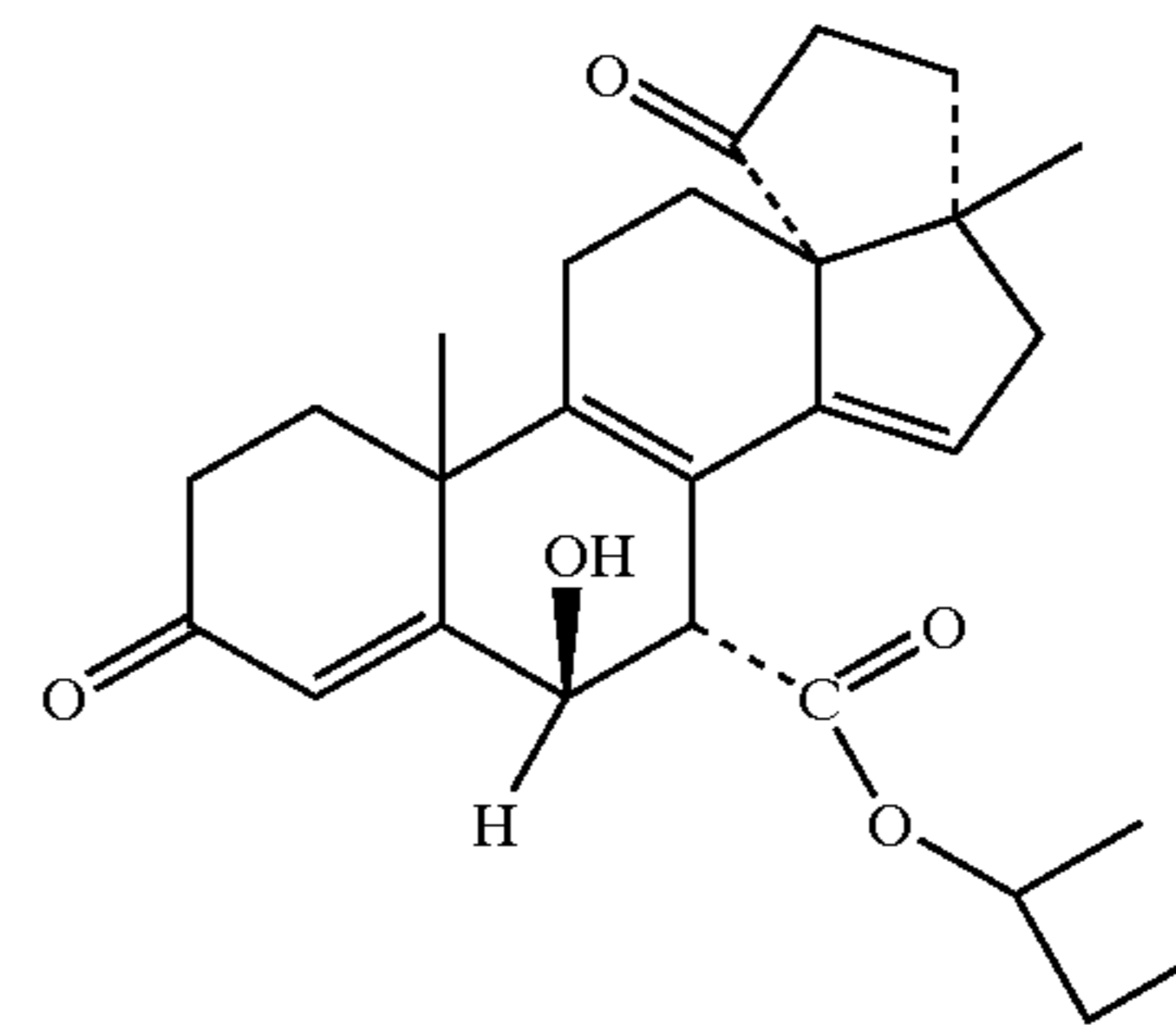
1-methylpropyl 3', 4', 5', 17-tetrahydro-6β-hydroxy-17β-methyl-3, 5'-dioxocyclopenta[13R, 17]-18-norandrosta-4, 8, 14-triene-7α-carboxylate
