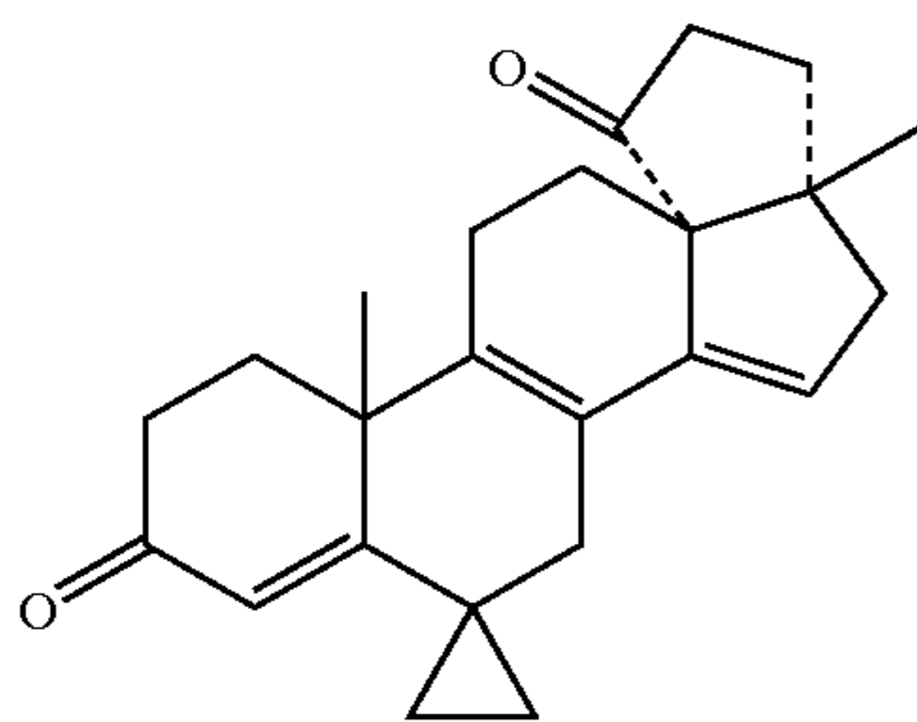
2', 3', 3' \alpha , 4', 6', 10', 11', 11' \alpha , 12', 13'-decahydro-3' aR, 3'a, 11'a-dimethyl-13' aR*-spiro[cyclopropane-1, 7' (9'H)-[1H]pentaleno[1, 6a-a]phenanthrene]-1', 9'-dione
