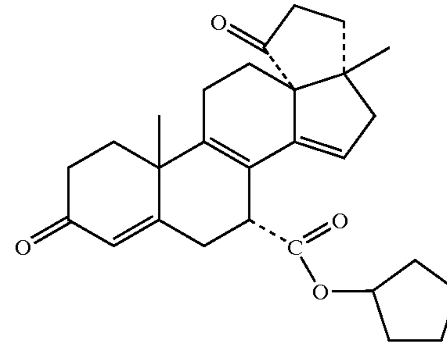
cyclopentyl 3', 4', 5', 17-tetrahydro-17β-methyl-3, 5'-dioxocyclopenta[13R, 17]-18-norandrosta-4, 8, 14-triene-7α-carboxylate
