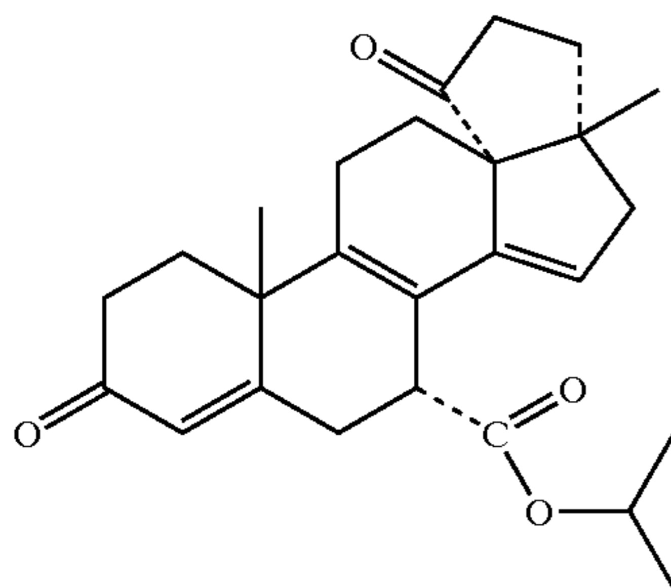
1-methylethyl 3', 4', 5', 17-tetrahydro-17β-methyl-3, 5'-dioxocyclopenta [13R, 17]-18-norandrosta-4, 8, 14-triene-7α-carboxylate
