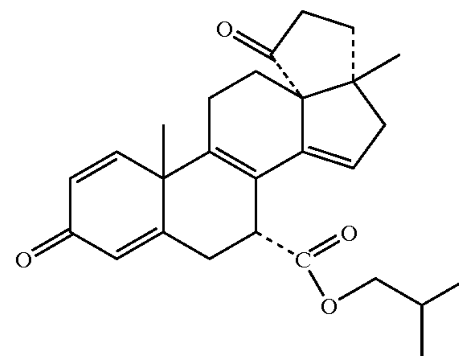
2-methylpropyl 3', 4', 5', 17-tetrahydro-17β-methyl-3, 5'-dioxocyclopenta [13R, 17]-18-norandrosta-1, 4, 8, 14-tetraene-7α-carboxylate
