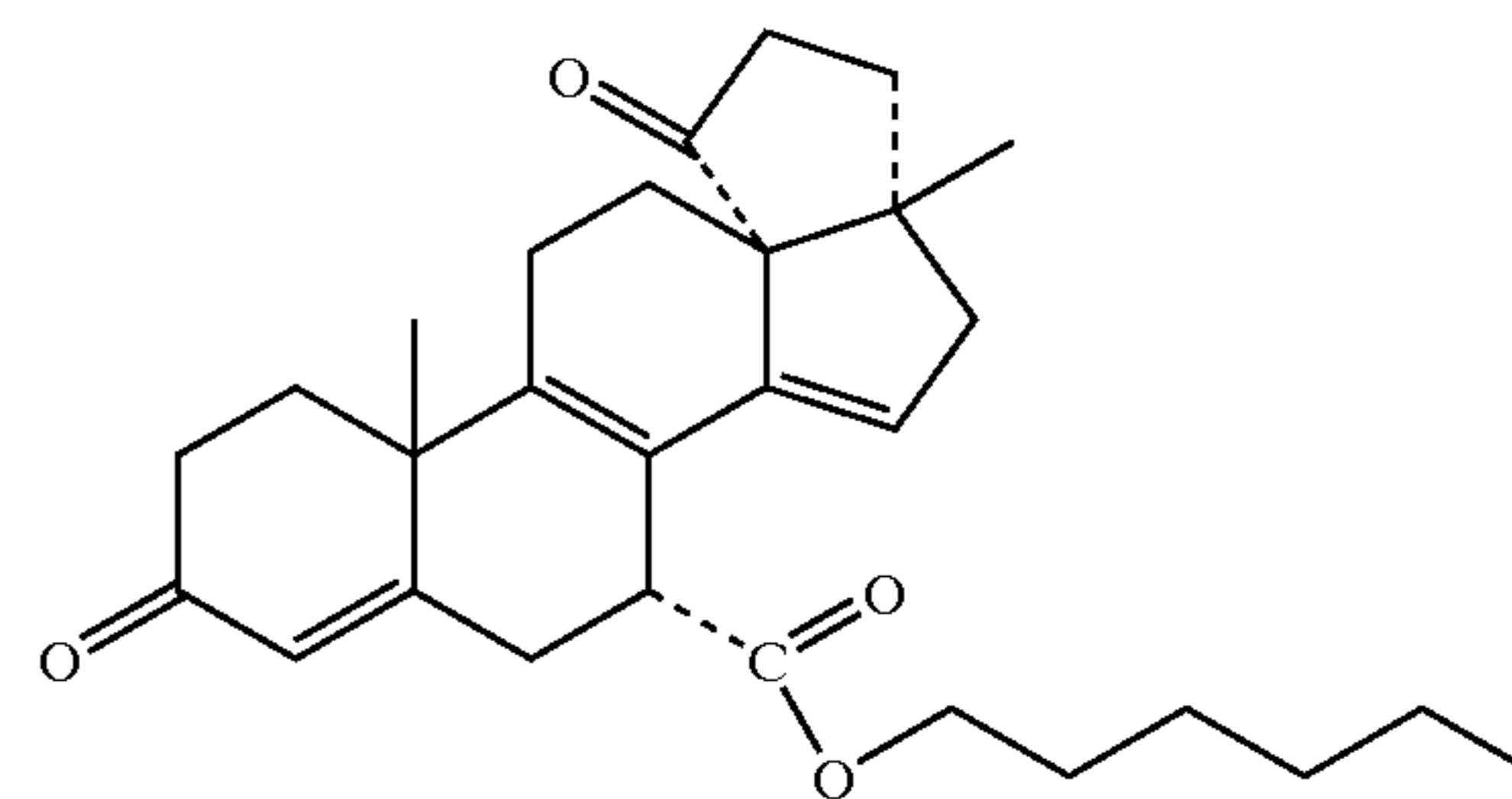
hexyl 3', 4', 5', 17-tetrahydro-17β-methyl-3, 5'-dioxocyclopenta [13R, 17]-18-norandrosta-4, 8, 14-triene-7α-carboxylate
