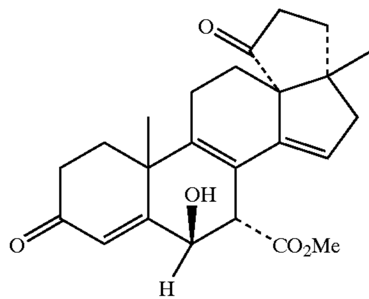
methyl 3', 4', 5', 17-tetrahydro-6β-hydroxy-17β-methyl-3, 5'-dioxocyclopenta[13R, 17]-18-norandrosta-4, 8, 14-triene-7α-carboxylate
