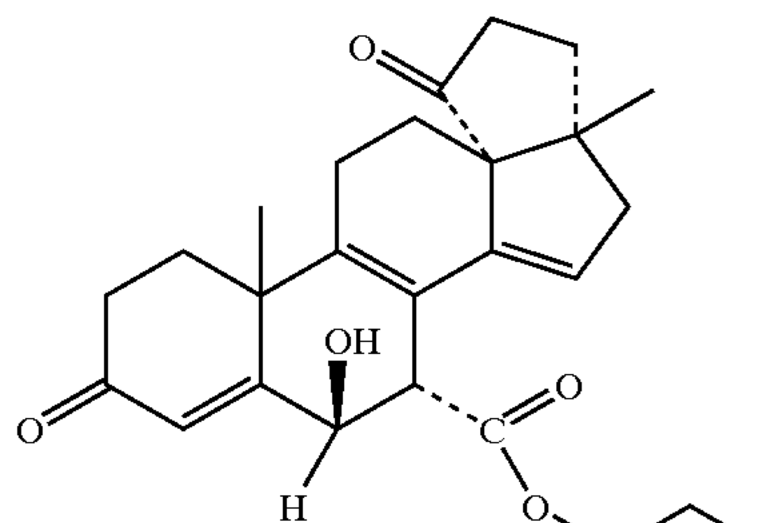
propyl 3', 4', 5', 17-tetrahydro-6β-hydroxy-17β-methyl-3, 5'-dioxocyclopenta[13R, 17]-18-norandrosta-4, 8, 14-triene-7α-carboxylate
