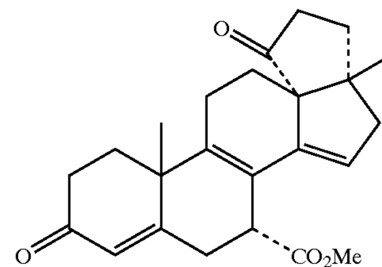
methyl 2, 2, 3a, 4, 6, 7, 9, 10, 11, 11a, 12, 13-dodecahydro-3αβ, 11αβ-dimethyl-1, 9-dioxo-1H-pentaleno[1, 6a-a]phenantrene-6α-carboxylate
