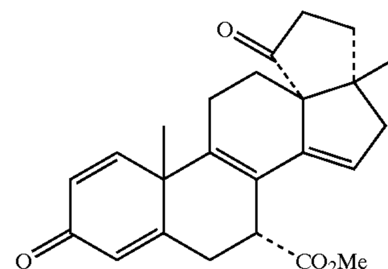
methyl 3', 4', 5', 17-tetrahydro-17β-methyl-3, 5'-dioxocyclopenta [13R, 17]-18-norandrosta-1, 4, 8, 14-tetraene-7α-carboxylate
