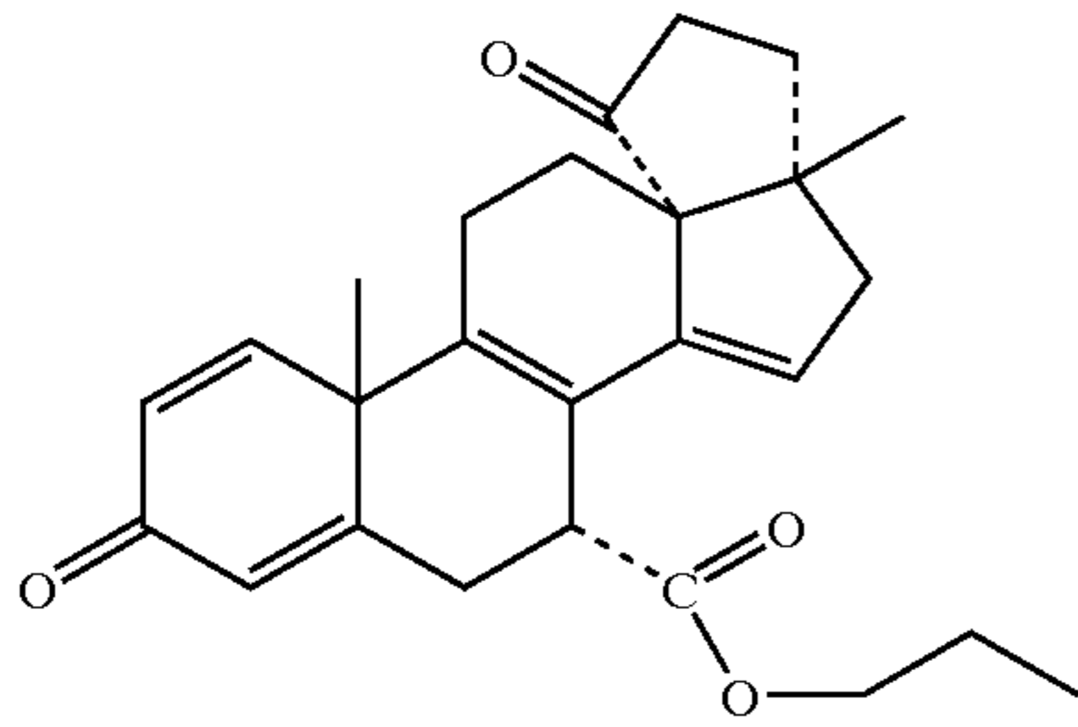
propyl 3', 4', 5', 17-tetrahydro-17β-methyl-3, 5'-dioxocyclopenta [13R, 17]-18-norandrosta-1, 4, 8, 14-tetraene-7α-carboxylate
