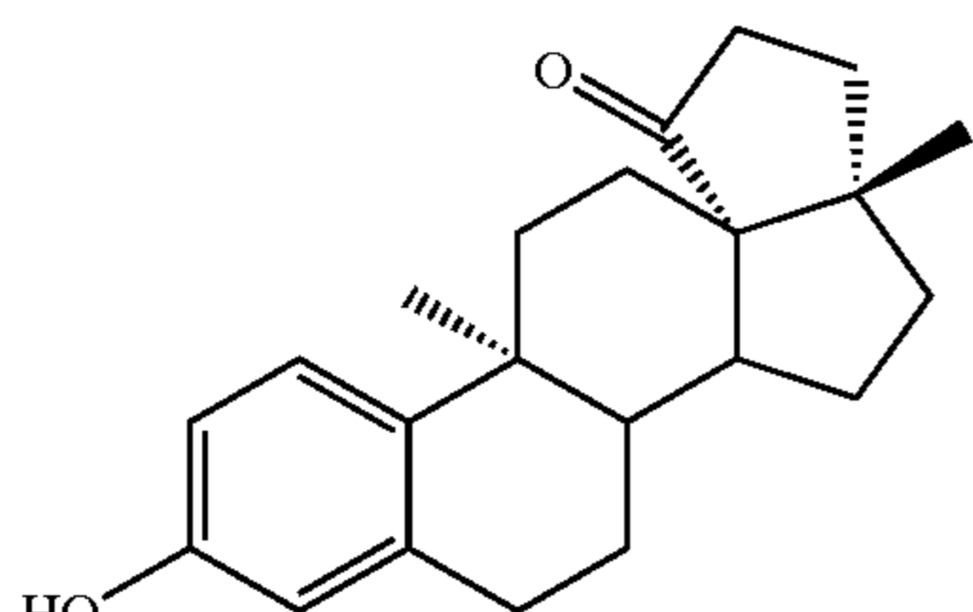
[13S, 17 \beta ]-3', 4'-dihydro-3-hydroxy-9, 17-dimethylcyclopenta[13, 17]gona-1, 3, 5(10)-triene-5'[2'H]-one
