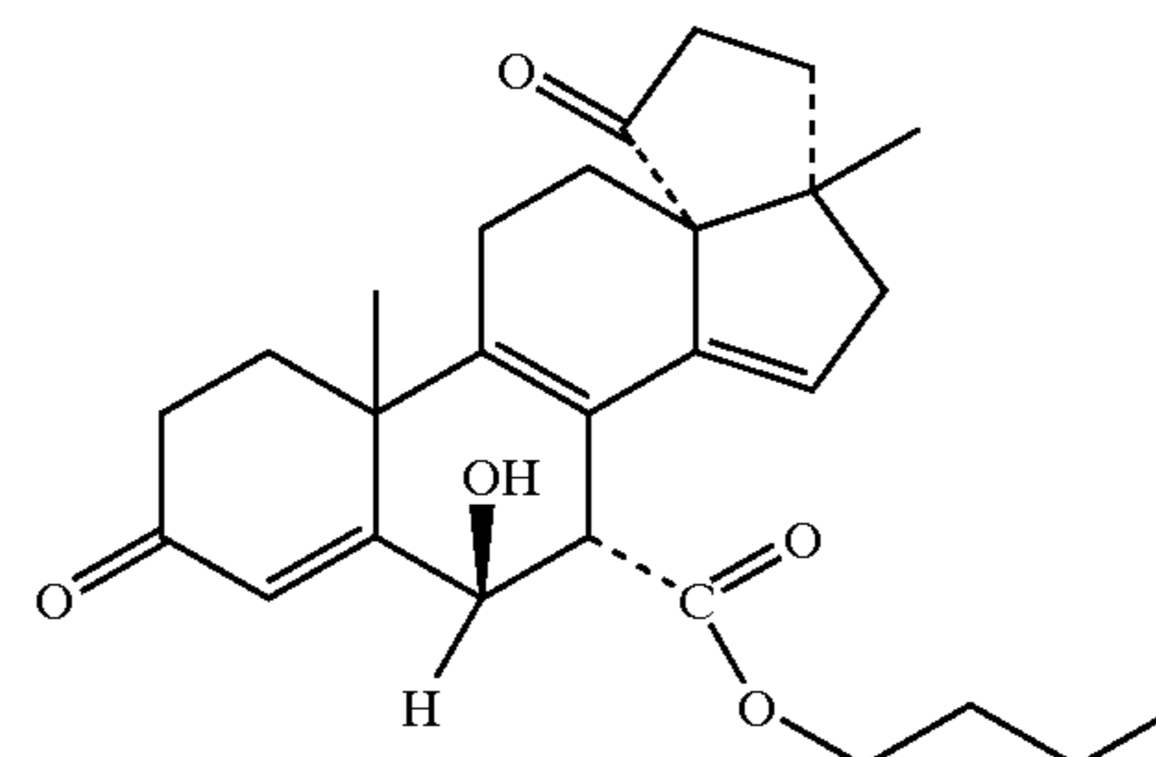
butyl 3', 4', 5', 17-tetrahydro-6β-hydroxy-17β-methyl-3, 5'-dioxocyclopenta[13R, 17]-18-norandrosta-4, 8, 14-triene-7α-carboxylate
