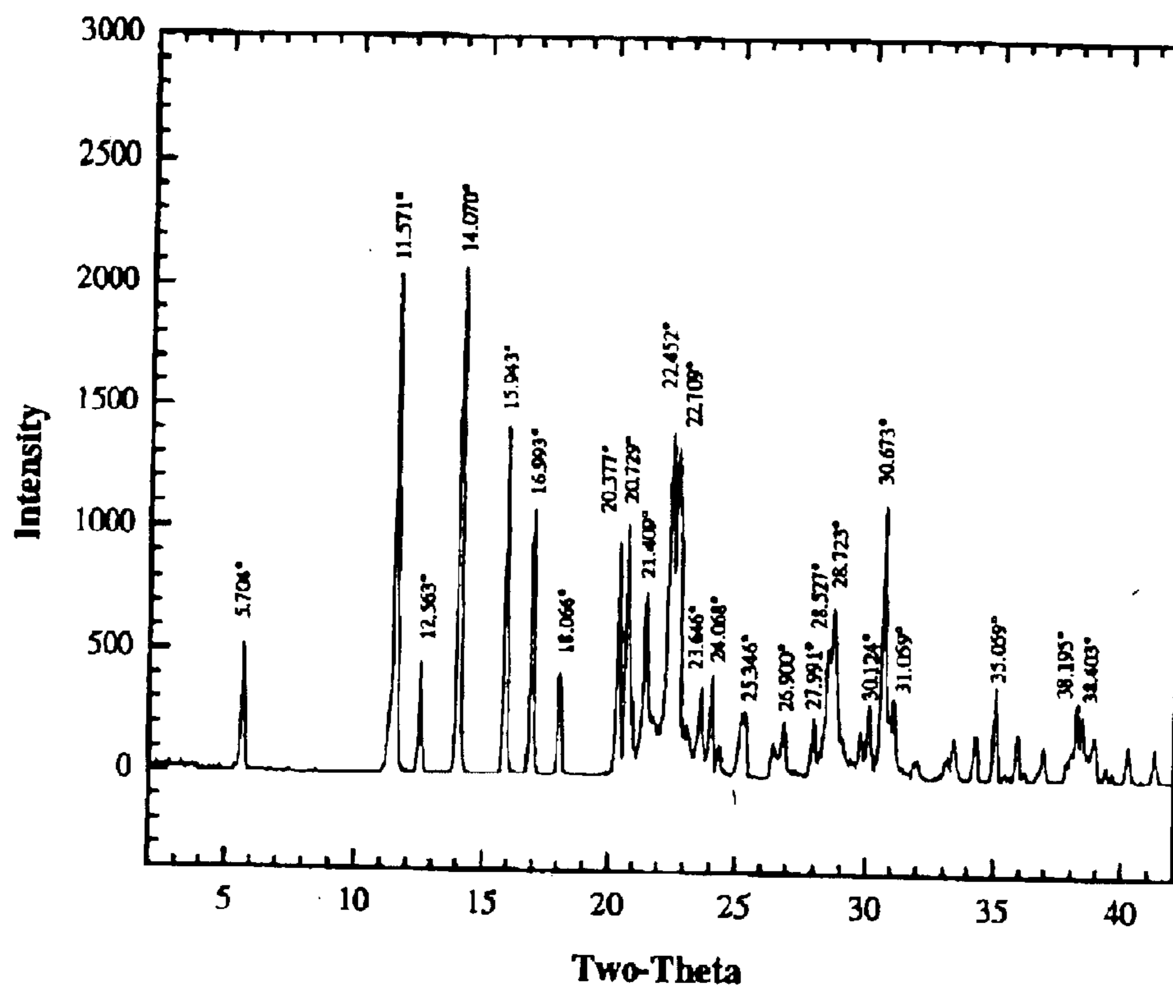
Figure 4 X-ray Powder Diffraction Pattern of Azacitidine, Form IV, Labeled with the more Prominent 2\theta Angles (Cu K \alpha Radiation)
