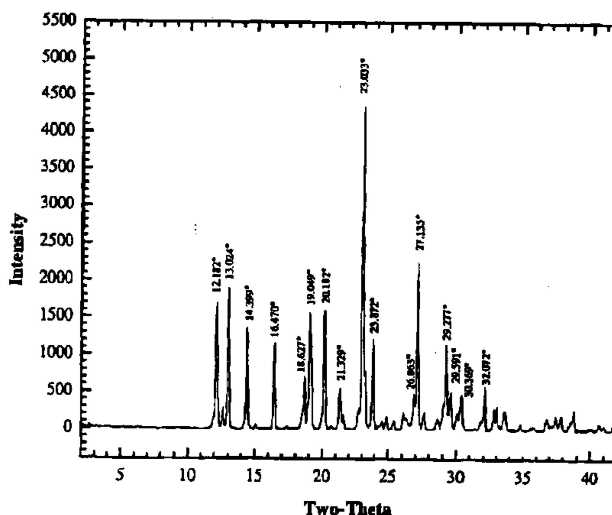
X-ray Powder Diffraction Pattern of Azacytidine, Form I, Labeled with the more Prominent 2θ Angles (Cu Kα Radiation)
