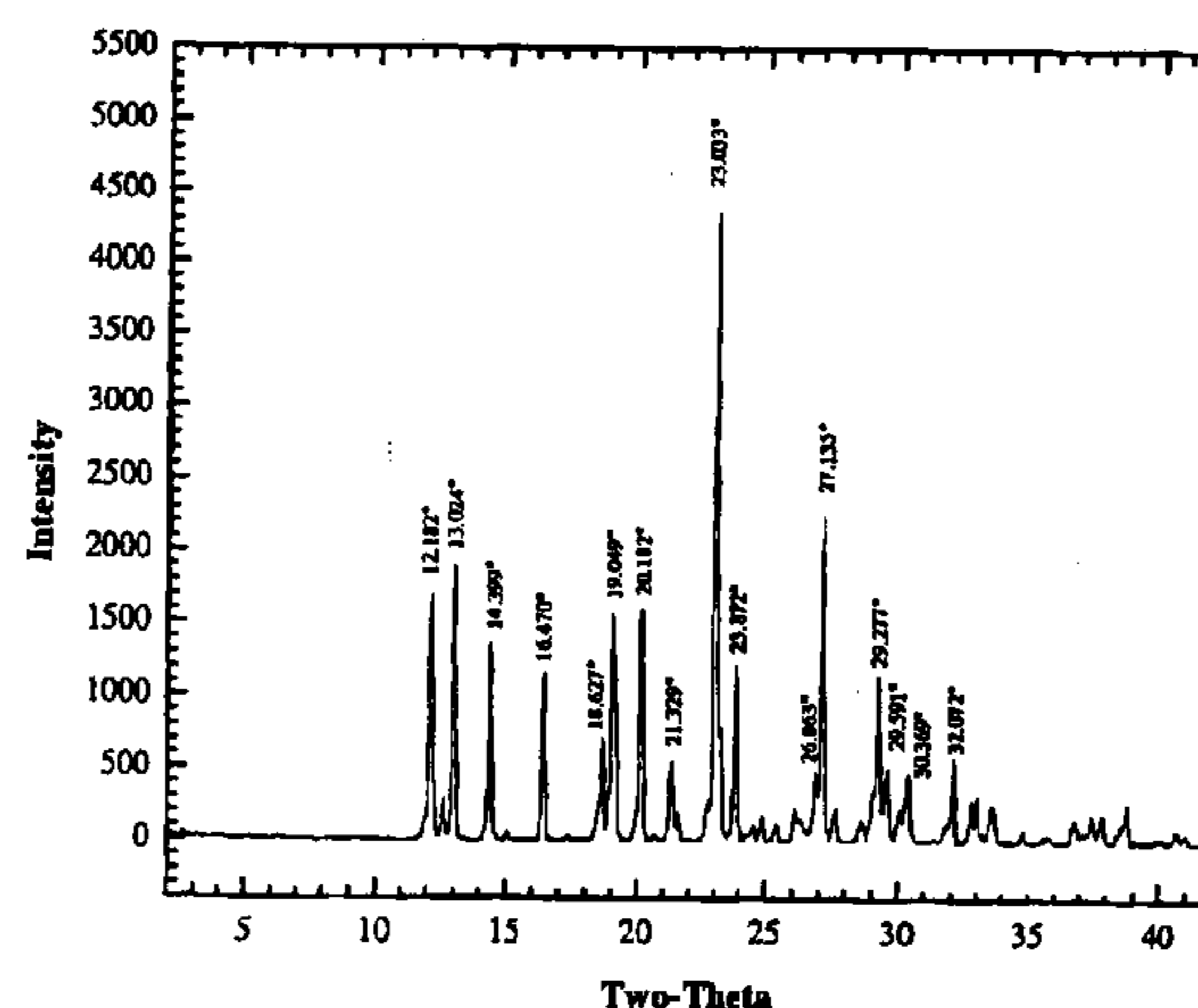
X-ray Powder Diffraction Pattern of Azacitidine, Form I, Labeled with the more Prominent 2θ Angles (Cu Kα Radiation)
